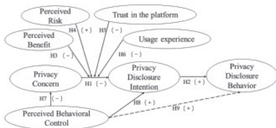
Figure 2. Conceptual Model
