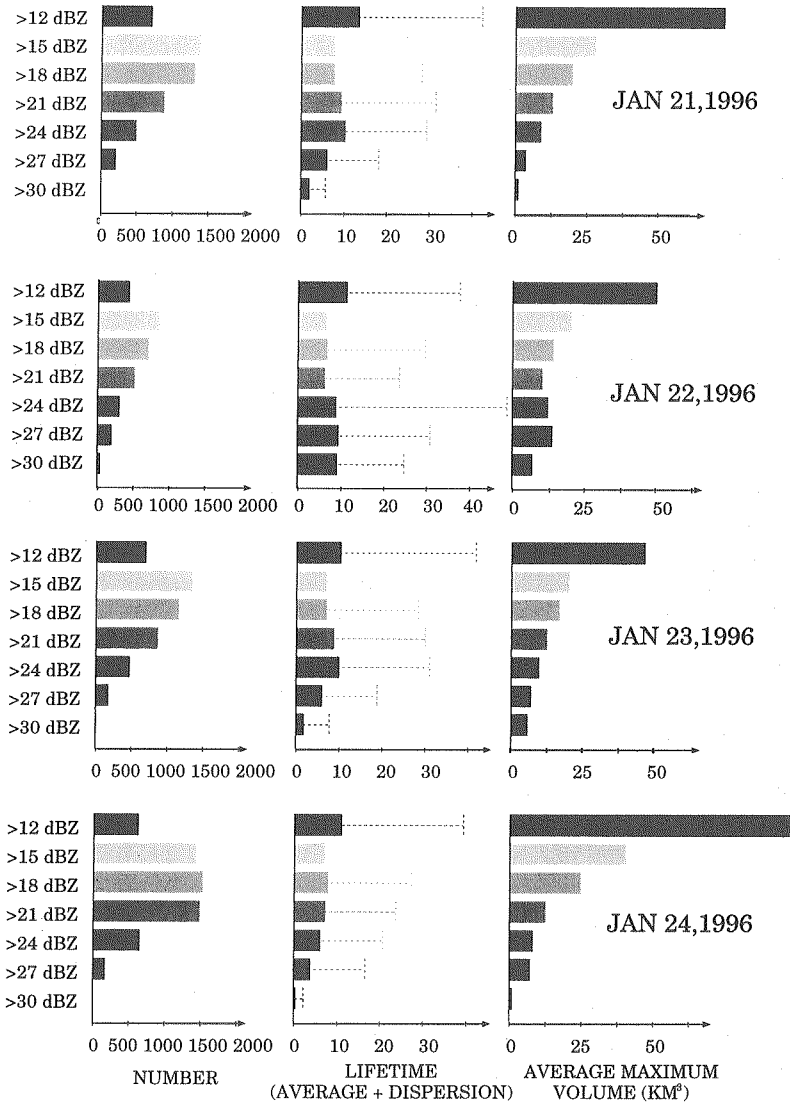
Fig. 8. Average lifetime of separate echoes (fixed reflectivity level tracking)
