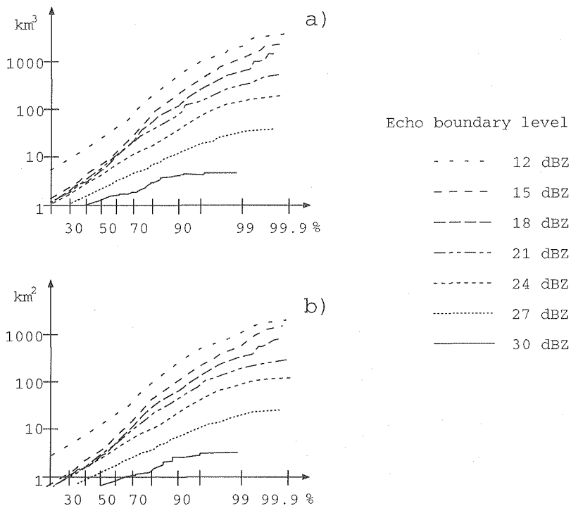
Fig. 2. Frequency distribution of observed echo sizes for different reflectivity levels. a) echo volumes, b) echo areas.
