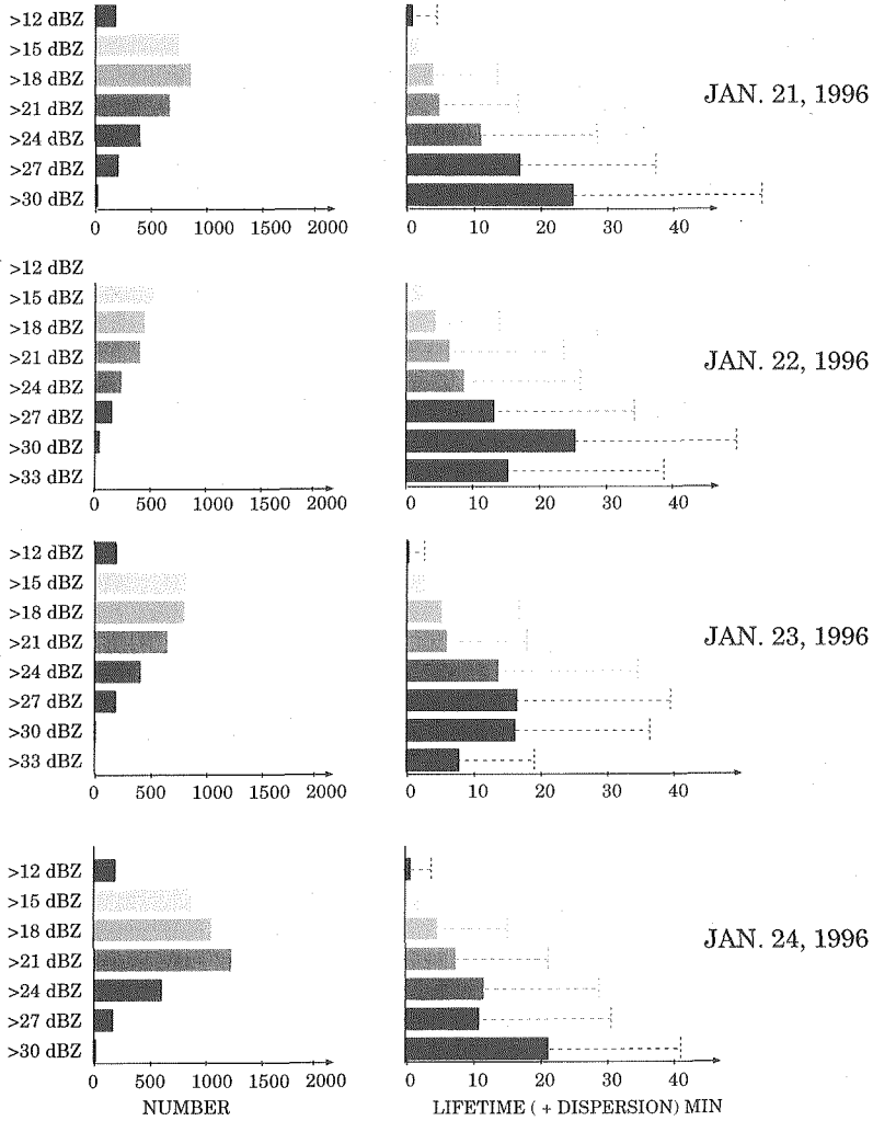
Fig. 9. Average lifetime of echo cores (maximal tracking).
