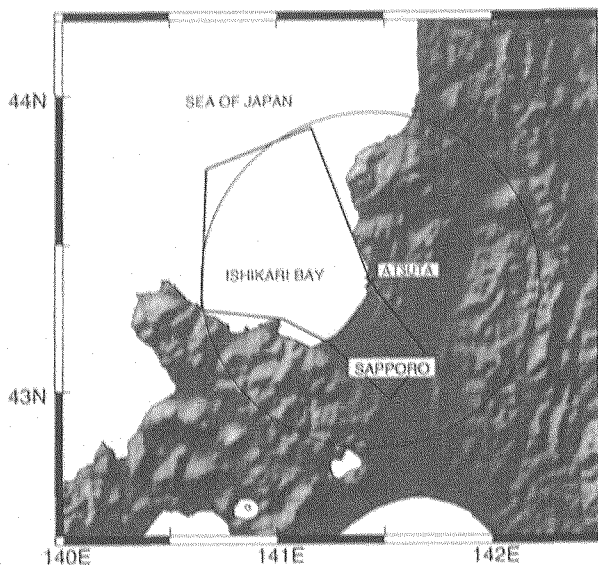
Fig. 1. Location of the radar site and observation range.
