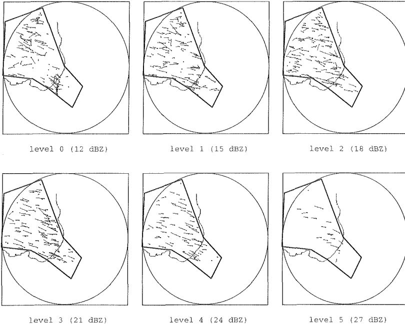
Fig. 5. Locations of echo centers at the time of maximal development for a volume criterion by reflectivity levels (fixed level tracking).
