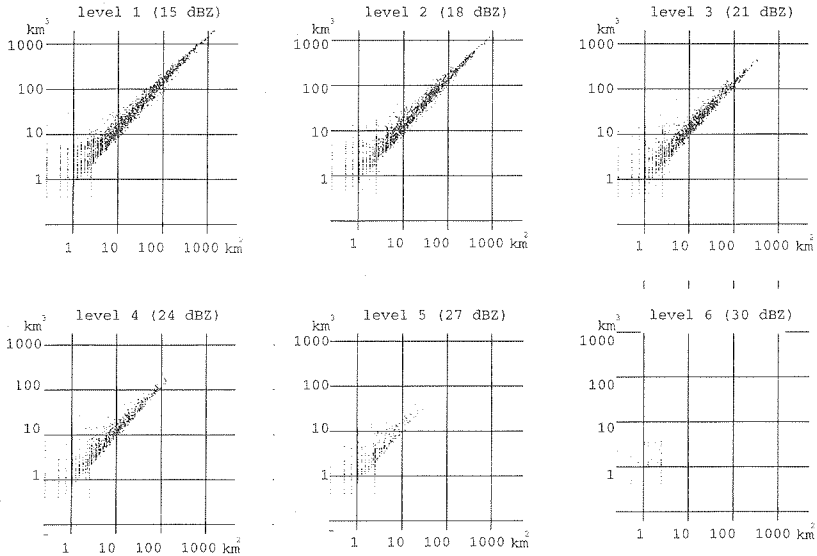
Fig. 4. Scatter-plot of volume versus area of individual echoes.
