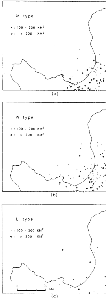
Fig. 6. Distributions of echo centers at the time of maximal echo sizes. Letters M, W, and L denote monsoon type, final period of monsoon type and low pressure type of the general weather pattern respectively. (After Kikuchi et al. (1989))
