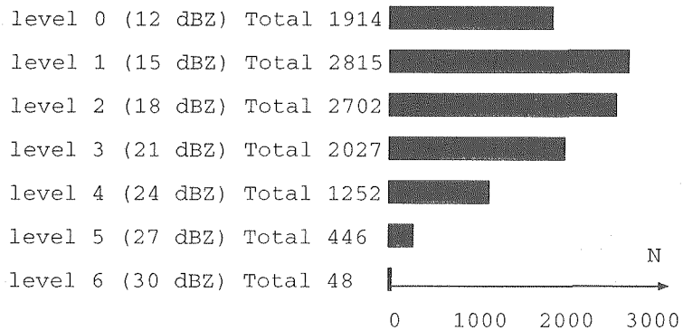
Fig. 3. Total number of echoes for different reflectivity levels.
