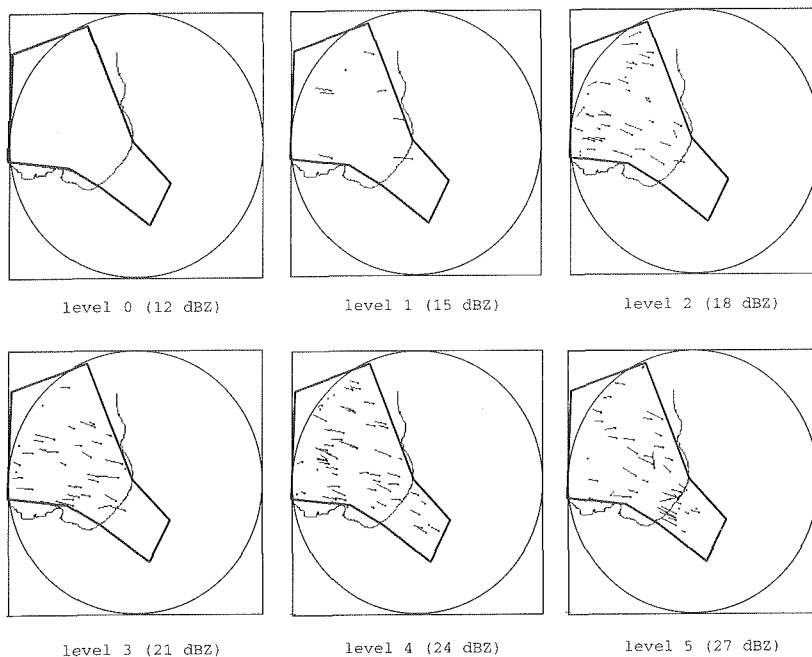
Fig. 7. Distributions of maximal echo development by reflectivity levels for a maximal reflectivity criterion.
