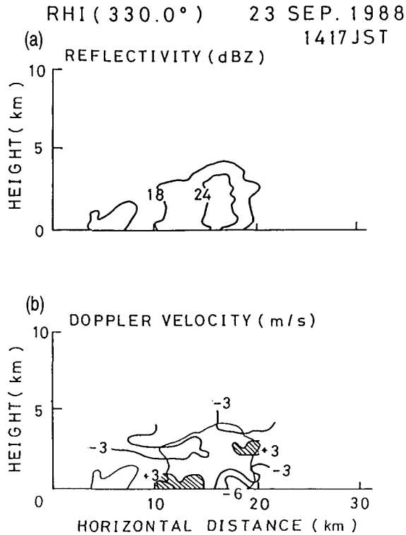
Fig. 5. Vertical cross sections (RHI scan) of (a) reflectivity and (b) Doppler velocity along 330.0^\circ in azimuth at 1417 JST on September 23, 1988. Contour intervals of reflectivity are 6 dBZ from 18 dBZ and those of Doppler velocity are 3 m/s.
