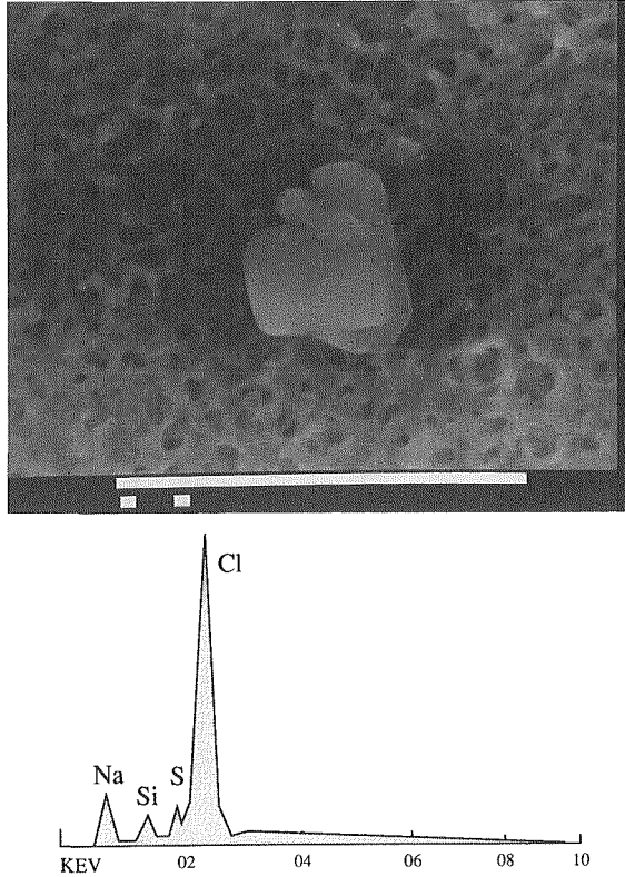
Fig. 10. Photograph of a mixed particle consisting of a large sea salt particle with small soil particle and the spectra of elements. (scale ; 10 \mu\text{m} )
