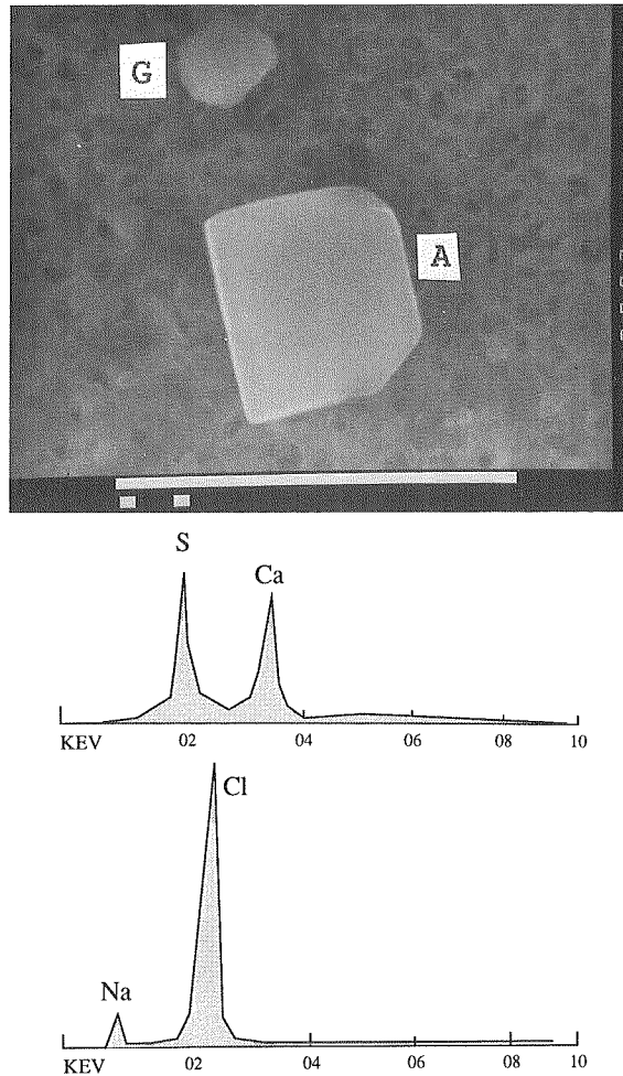
Fig. 7. Photograph of the SEM image. (A) a sea salt particle ; (G) a gypsum particle with spectra. (scale ; 10 \mu m)
