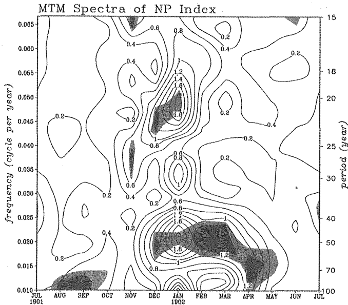
Fig. 1. MTM spectra of NP index for each month. The contour indicates the spectrum amplitude and the color denotes the significance of the spectrum. Heavy and light shade indicates where the spectrum peak is significant at 90 and 95 % confidence limits, respectively.
