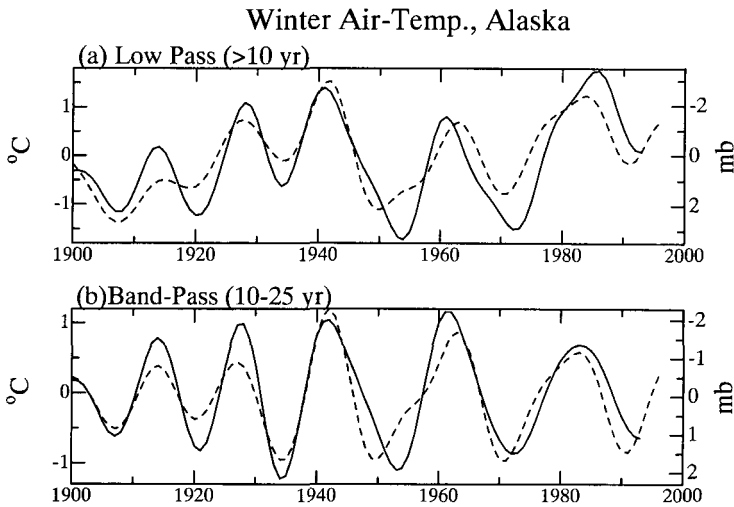
Fig. 7. (a) Low-pass filtered and (b) band-pass filtered winter air-temperature over Alaska (solid curve with left axis) and NP index (dashed curve with right axis). The cut-off period of the low-pass filter is 10 years, and cut-off periods of the band-pass filter are 10 and 25 years. For the easier comparison between the air-temperature and NP index, the axis for the NP index is reversed (negative direction is toward the top of the page).
