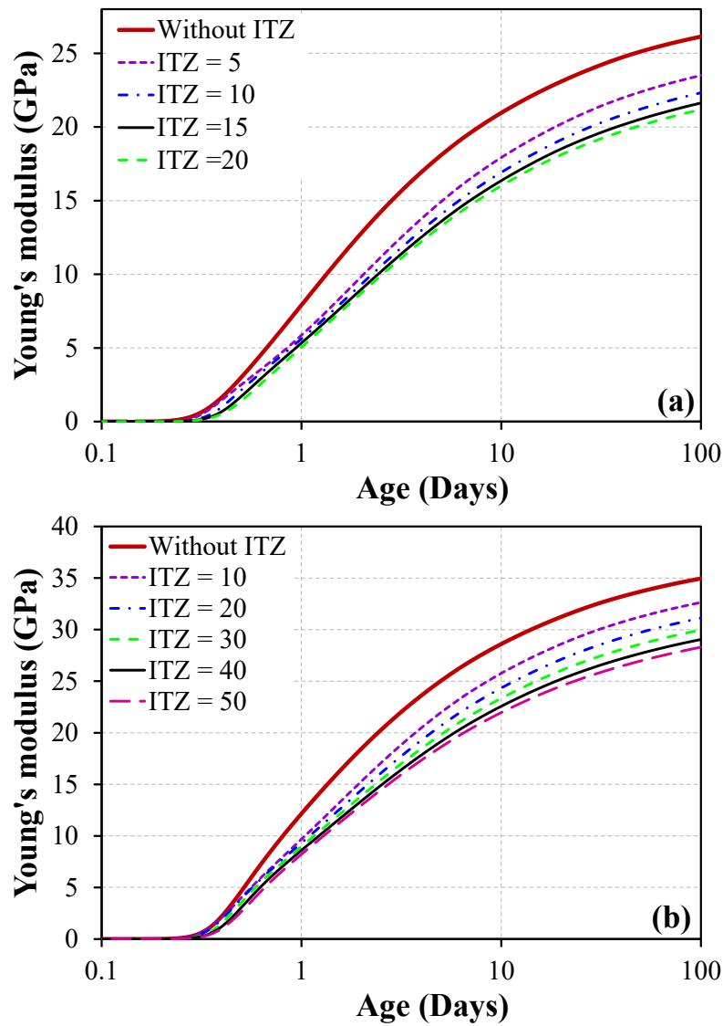
Figure 4.7: Variation of Young's modulus with hydration period for different ITZ thickness (a) for mortar and (b) for concrete
