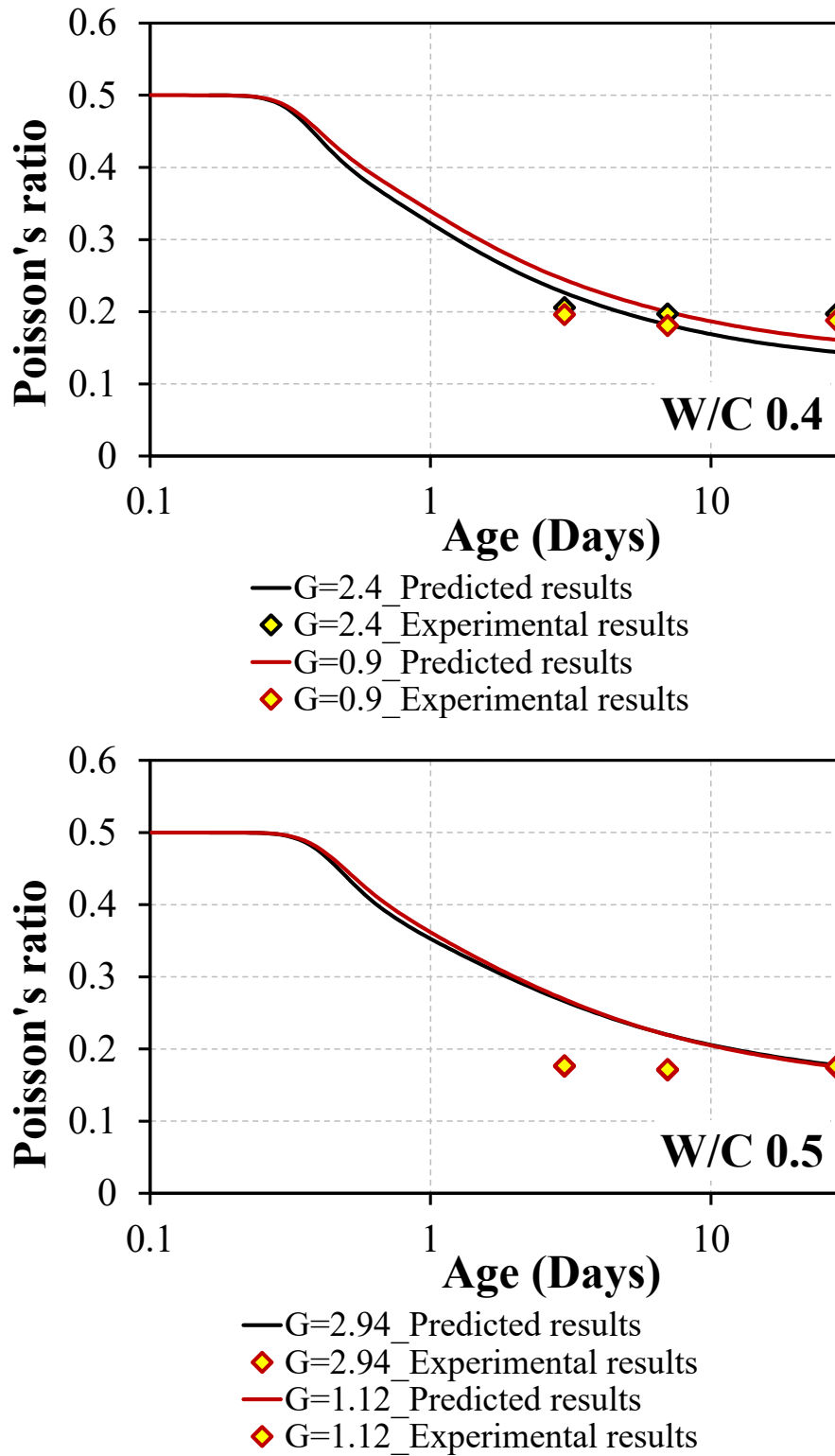
Figure 4.16: Validation of Poisson's ratio with hydration period for w/c ratio of 0.4 and 0.5 (G stands for weight ratio coarse aggregate/cement)
