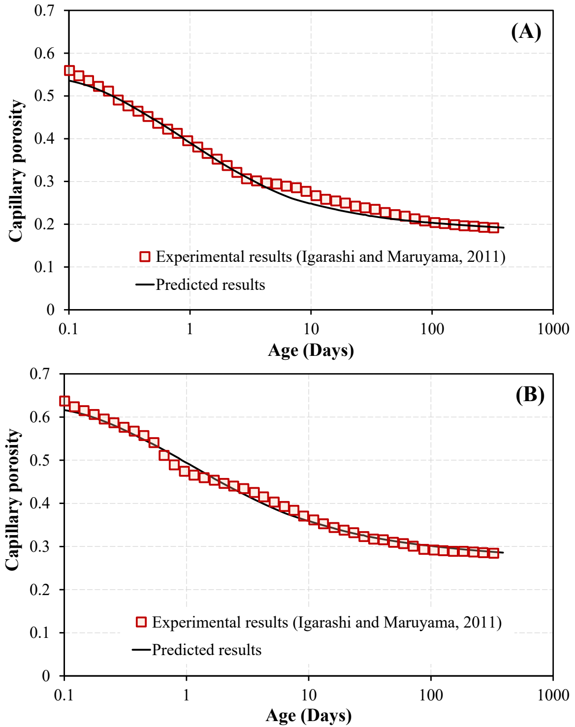
Figure 3.8: Variation of capillary porosity with hydration period for w/c of (A) 0.4 and (B) 0.55.
