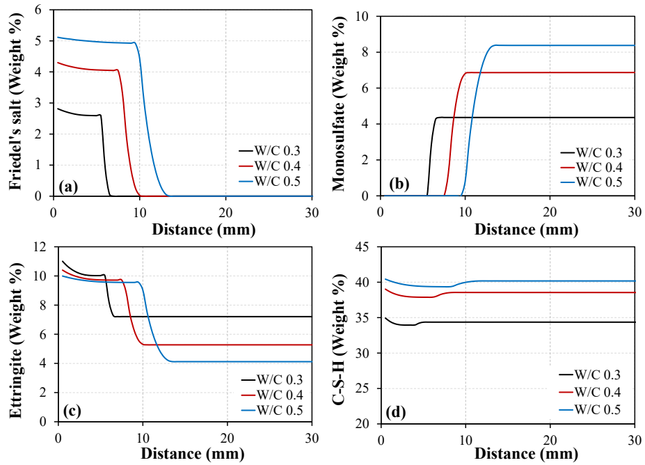
Figure 5.7: Variation of weight % of (a) Friedel's salt, (b) Monosulfate, (c) Ettringite and (d) C-S-H for w/c of 0.3, 0.4 and 0.5
