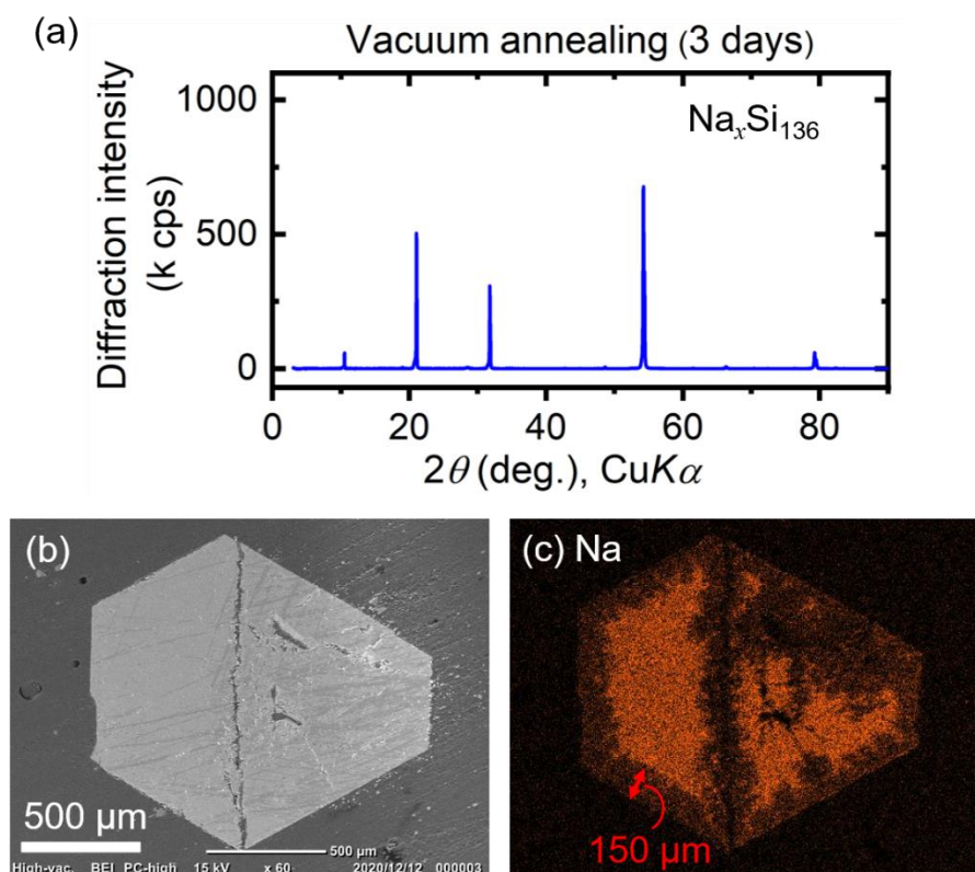
Figure S2. (a) X-ray diffraction (XRD) pattern, (b) scanning electron microscopy (SEM) image, and (c) EDS mapping of Na in the \text{Na}_x\text{Si}_{136} sample that was obtained via vacuum annealing at 450\ ^\circ\text{C} for 3 days.
