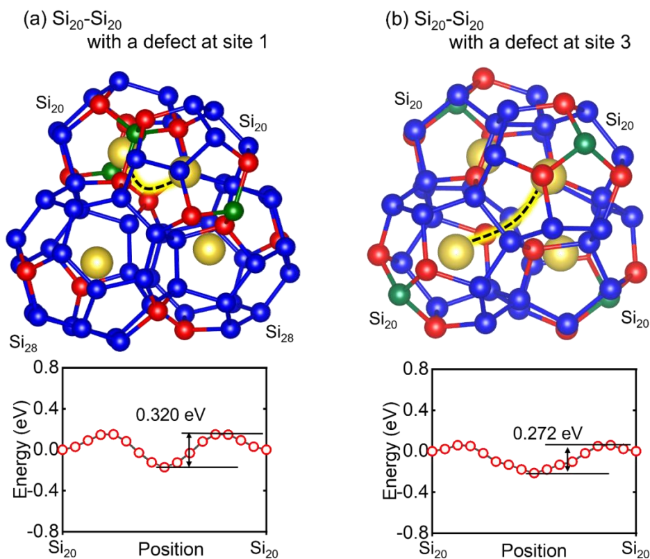
Figure 6. Two cases of the migrations between \text{Si}_{20}\text{-Si}_{20} in the model with Si defects at Sites (a) 1 and (b) 3. These cases exhibit the lowest and second-lowest \Delta G s among the seven cases in the model exhibiting a defect. The other cases are shown in Figure S13. The migration paths are highlighted, and the energies along the migration paths are shown in the bottom figures. The crystal structures were drawn with VESTA. [7]
