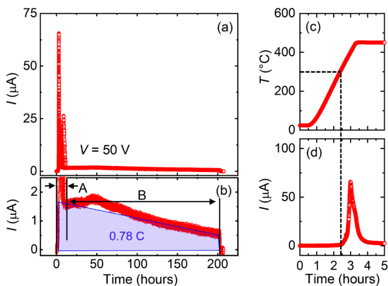
Figure S4. (a) Dependence of the electrical current ( I ) on time during the ADC process at V = 50\text{ V} . (b) Magnified view of (a) between 0 and 2.5 \mu\text{A} . (c and d) Magnified views of the temperature ( T ) and I between 0 and 5 h. (A) DC polarization occurred between 0 and 15 h, and (B) \text{Na}^+ migrated from the sample to NASICON between 15 and 200 h. A and B correspond to those in Figure 4(a). The final product is shown in Figure S5.
