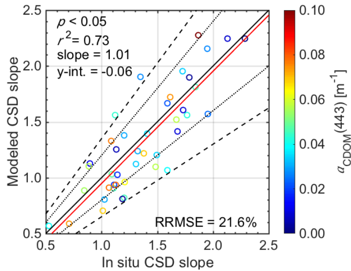
Figure 3.2. Comparison of in situ CSD slope values determined from in situ chl a size and modeled CSD slope derived from estimated a_{ph}^{std}(\lambda) through a modified quasi-analytical algorithm using the in situ PRR data. Black and red solid lines represent the 1:1 agreements and regression lines, respectively. Dotted and dashed lines represent \pm 20\% and \pm 35\% ranges. Color of markers represents in situ measured a_{CDOM}(443) .
