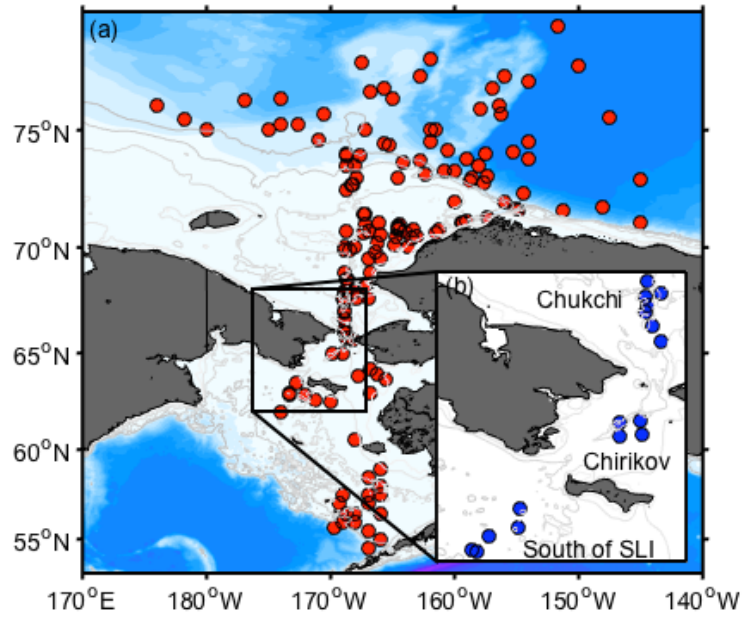
Figure 3.1. In situ observation stations for (a) optimizing the chlorophyll- a (chl a ) size distribution (CSD) model and (b) evaluating of changes in biomass and distribution of the benthic macrofauna.
