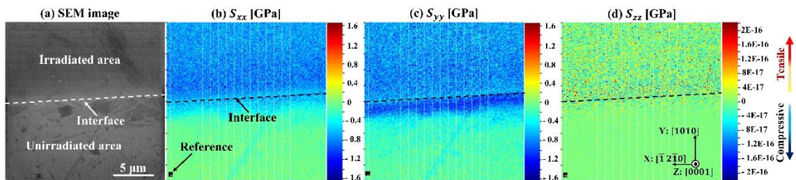
Fig. 3.9. Stress distribution in the selected-area \text{He}^+ ion irradiated 4H-SiC with fluence of 5 \times 10^{16} \text{ cm}^{-2} . (a) SEM image. (b)-(d) corresponding to stress composition in X, Y and Z
