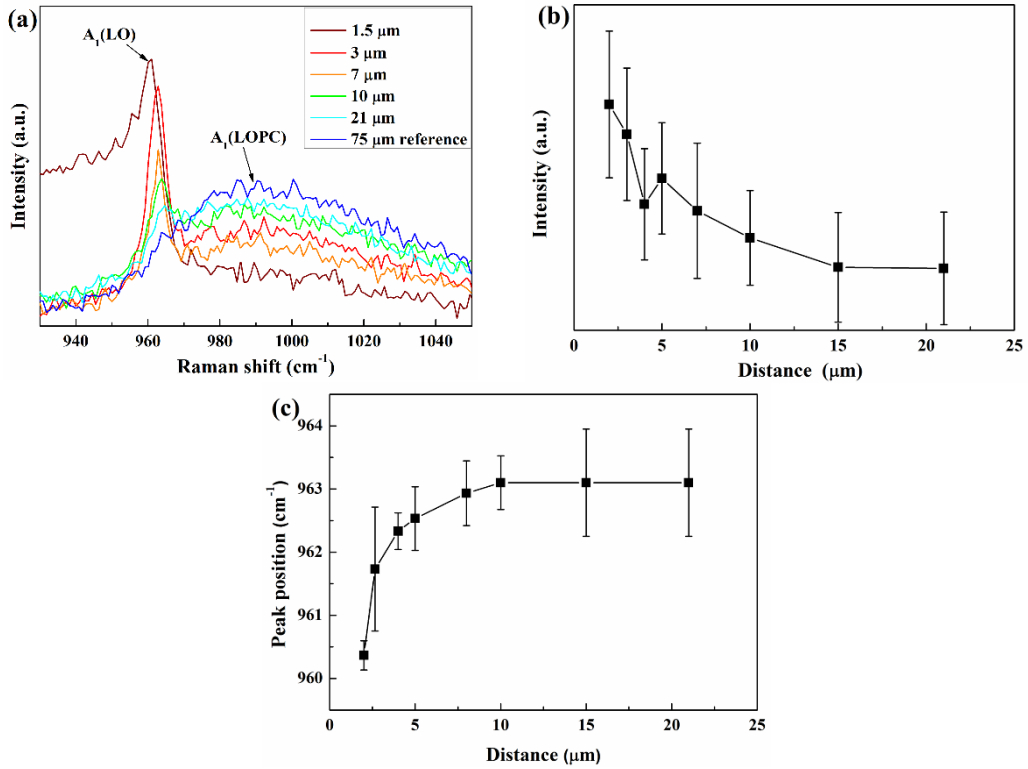
Fig. 2.10. Variation of the A_1(\text{LO}) mode in the substrate close to the irradiated/unirradiated interface. (a) Variation of the A_1(\text{LO}) mode (b) intensity and (c) peak position of A_1(\text{LO}) as a function of the distance from the interface [21].
