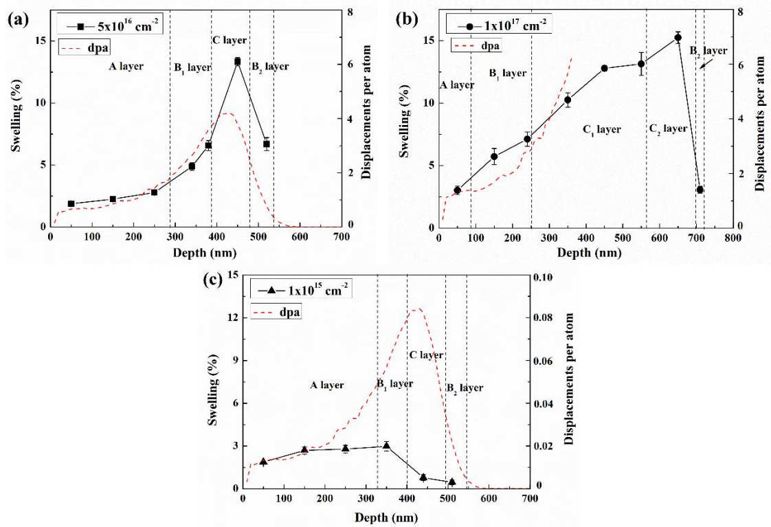
Fig. 4.3. Swelling Profile as a function of depth combined with the estimated dose profile in selected-area He + ion-irradiated 4H-SiC irradiated with medium fluence (a) high fluence (b) and low fluence (c). Due to the expansion of amorphous region at this fluence,
