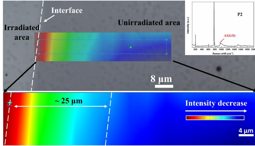
Fig. 2.9 Raman mapping scanning results of A_1(\text{LO}) mode around the interface.
