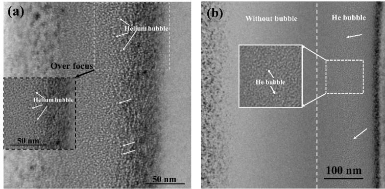
Fig. 4.7. TEM images He bubbles in the \text{He}^+ ion-irradiated samples with medium fluence (a) and high fluence (b) [21].
