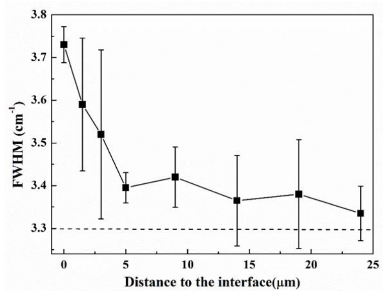
Fig. 2.5. FWHM of E_2(\text{TO}) with the distance to the interface.
