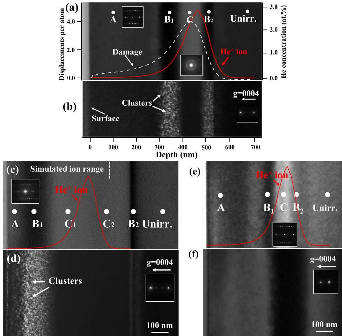
Fig. 4.1. Cross-section image of He + ion irradiated 4H-SiC with different fluences. (a, b) At medium fluence. (a) along the [11\bar{2}0] zone combined with the displacement damage (white dashed line) and the He + ion concentration (red solid line) profile. (b) Weak-beam dark-field TEM image under the g/3g , g=0004 condition. (c, d) At high fluence. (c) along the [11\bar{2}0] zone and (d) weak-beam dark-field TEM image under the g/3g , g=0004 condition. (e, f) At low fluence. (e) near the [11\bar{2}0] zone and (f) two-beam bright-field TEM image under the g=0004 condition. The inset images in (a), (c) and (e) are the selected-area diffraction pattern of the constituent areas, and the inset images in (b), (d) and (f) correspond to the diffraction condition when taking each image [21].
