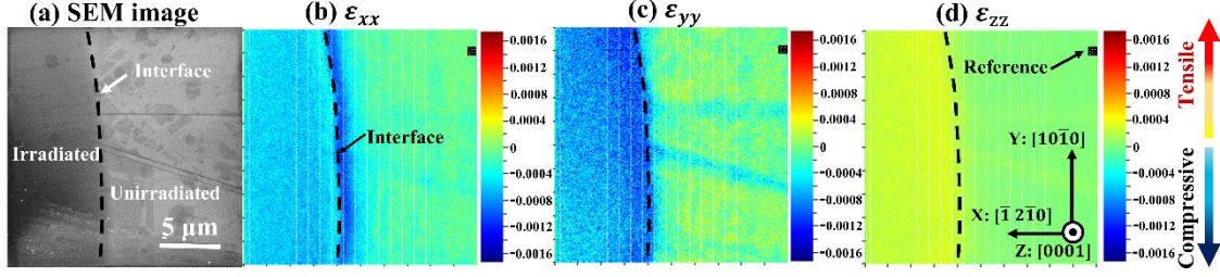
Fig. 2.3. Strain maps in selected-area \text{He}^+ ion irradiated 4H-SiC. (a) SEM image, (b–d) residual elastic strains with (b) \epsilon_{xx} , (c) \epsilon_{yy} , and (d) \epsilon_{zz} representing the strain horizontal ( X ), vertical ( Y ) and normal to the sample surface ( Z ), respectively. A reference was selected for the strain analysis at unirradiated area as shown in (d). Strain formed at some positions of unirradiated area is owing to the scratch on the sample surface [21].
