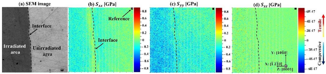
Fig. 3.10. Stress distribution in the selected-area \text{He}^+ ion irradiated 4H-SiC with fluence of 1 \times 10^{15} \text{ cm}^{-2} . (a) SEM image. (b)-(d) corresponding to stress composition in X, Y and Z direction.
