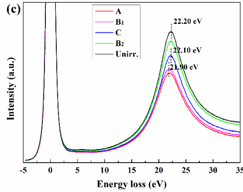
Fig. 4.2. Plasmon-loss EELS spectra at different damage regions in samples irradiated with fluences of (a) 5 \times 10^{16} , (b) 1 \times 10^{17} , and (c) 1 \times 10^{15} \text{ cm}^{-2} . The spectra in (a–c) correspond to the regions marked in Fig. 4.1(a), (c), (e), respectively [21].
