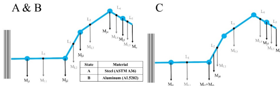
Figure 23- Components weight diagram in A, B, and C design
