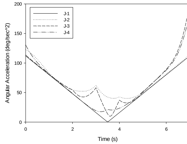
Figure 35. Angular acceleration of joints in upward motion.
