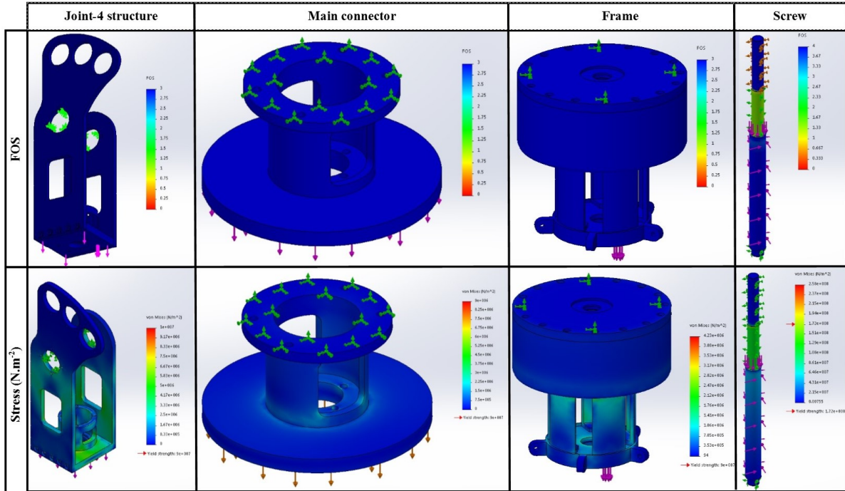
Figure 80. Static simulation of main components.
