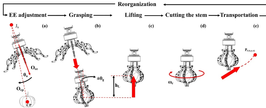
Figure 67. Robotic harvesting methodology.
