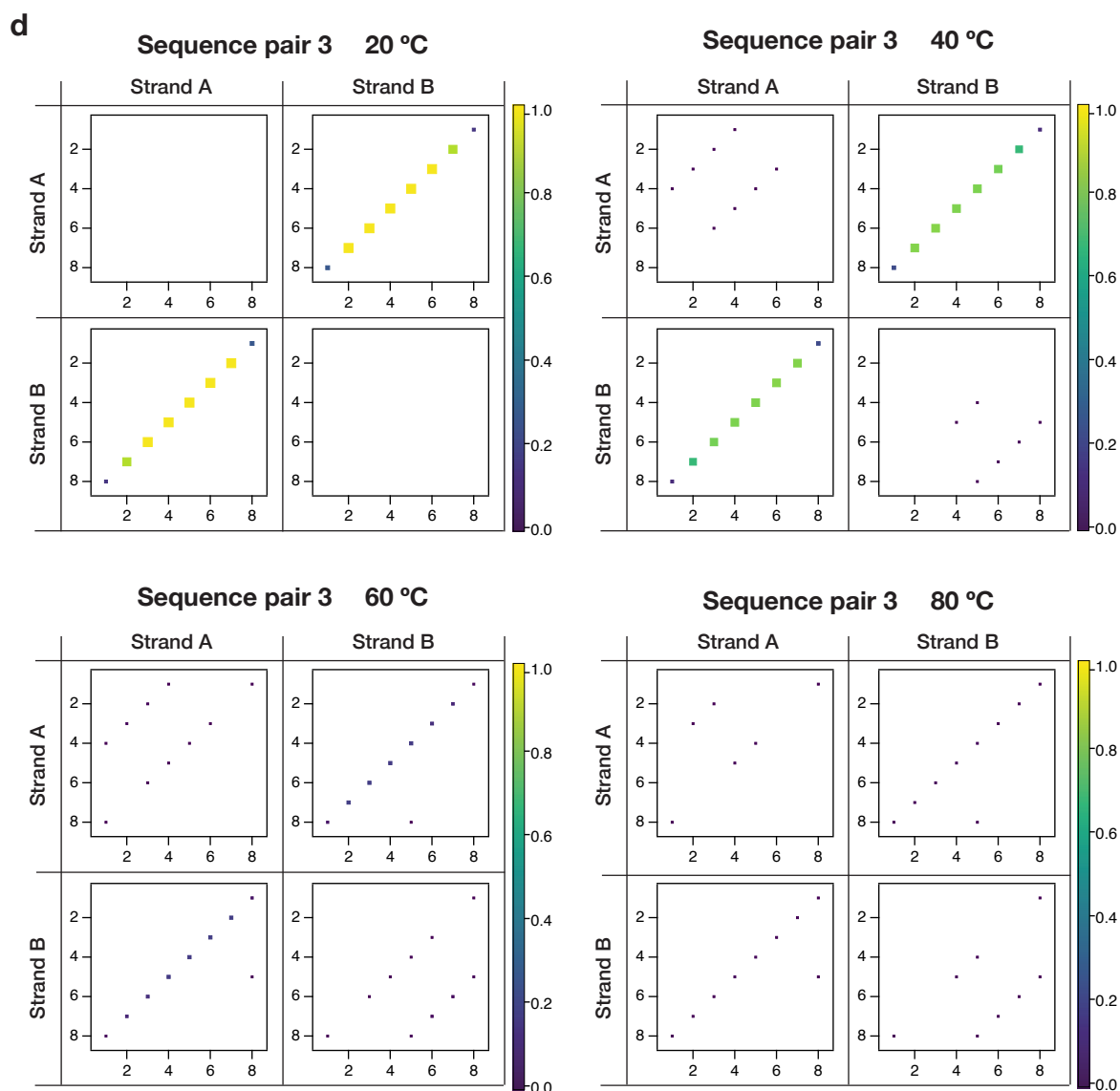
Figure S2. The equilibrium pair probability matrices for the designed sequences in this work and the examples of inappropriate sequences (the sequences are the same as in Fig S1). The pair probability matrices were calculated using NUPACK [10] from 20 °C to 80 °C at the sodium concentration of 50 mM. The sodium concentration in the calculation was slightly higher than the actual concentration (37.5 mM) due to the limitation of the software. The colored marks in each matrix represents the pair probabilities for the i th base in a DNA strand hybridizing with j th base in another DNA strand. The base index starts from 5'-terminal and ends at 3'-terminal. The size of marks with low probability was reduced to improve the visibility. For sequences showing the ideal two-state transition, we should only observe the diagonal elements and only in the combination of strand A vs strand B and strand B vs strand A. While the sequence pair used in this work and the sequence pair 3 (short oligo DNA, 8 mer)
