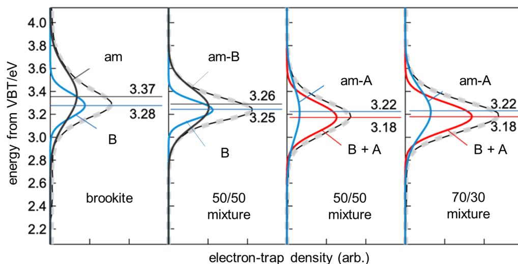
Figure 5-12 Deconvolution of ERDT patterns for (a) brookite, (b) mixture of brookite and amorphous titania in the ratio of 50/50, (c)–(d) mixture of brookite and anatase (ST-21) in the ratio of 50/50 and 70/30 with Gaussian-curve fitting.
