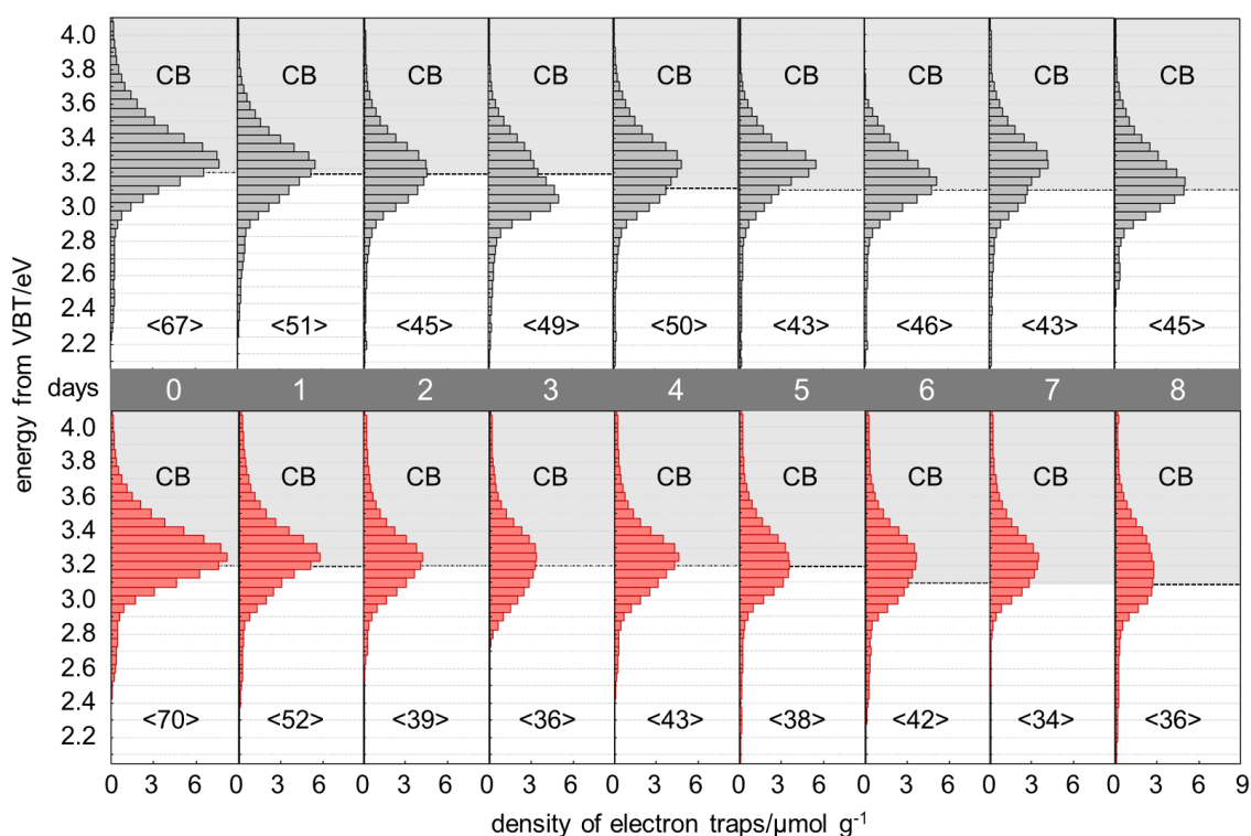
Figure 5-9 ERDT/CBB patterns of (upper) original, brayed and (lower) post-calcined samples. Doted lines indicate conduction band-bottom position and figures in < > denote total density of electron traps.
