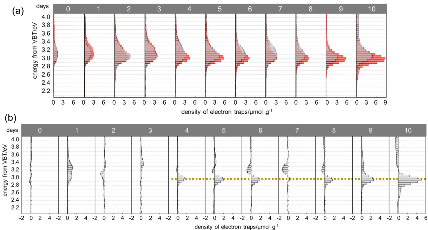
Figure 4-10 (a) Overlapping ERDT patterns of (black) original, brayed and (red) post-calcined samples and (b) subtracted ERDT patterns of post-calcined samples from original and brayed samples. Peaks of electron traps in negative and positive value indicate decrease and increase by post calcination, respectively. Dotted line indicates the peak position of the sample brayed for >3 d.
