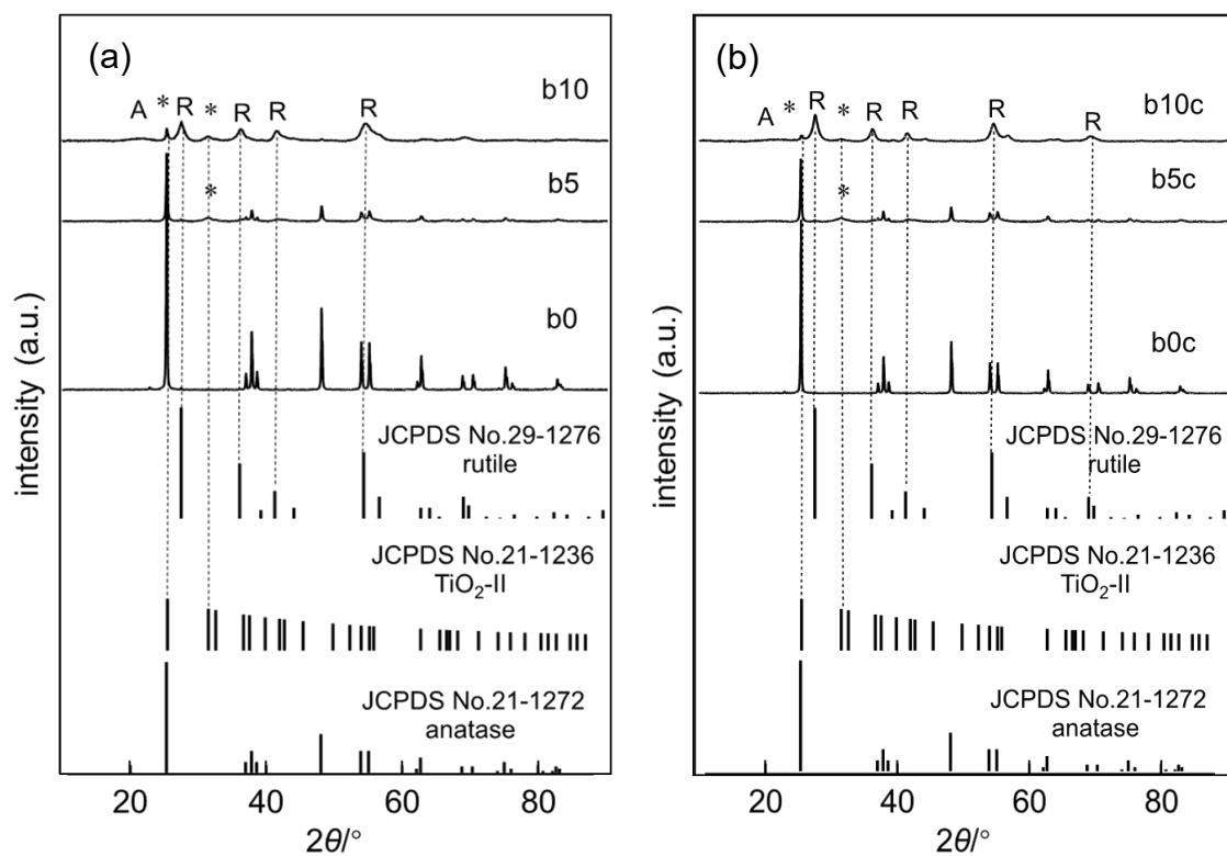
Figure 4-6 X-ray diffraction patterns of (a) original rutile, brayed and (b) post-calcined samples and those of pure rutile, \text{TiO}_2\text{-II} and pure anatase.
