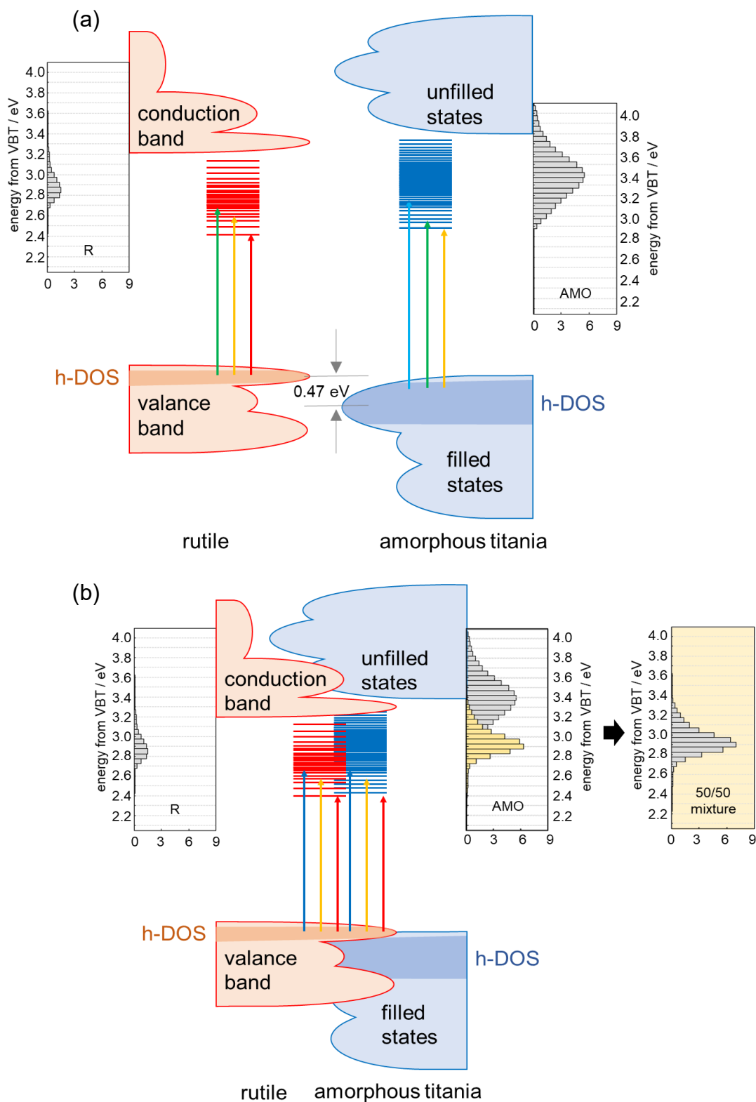
Figure 3-14 Interparticle charge-transfer excitation of rutile and amorphous titania. mixtures with (a) isolated and (b) contacted samples.
