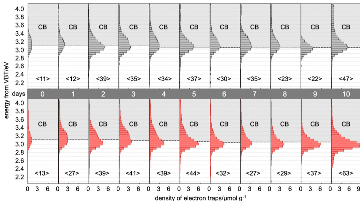
Figure 4-9 ERDT/CBB patterns of (upper) original, brayed and (lower) post-calcined samples. Doted lines indicate conduction band-bottom position and figures in <> denote total density of electron traps.
