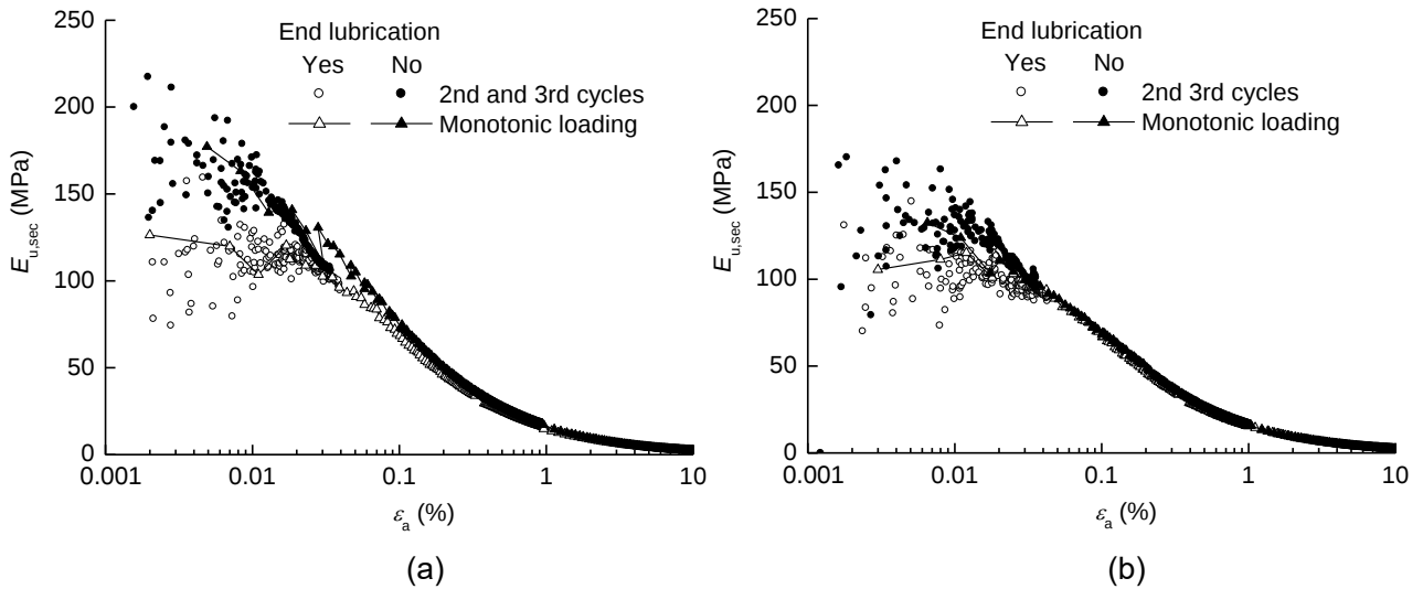
Figure 21: Secant undrained Young's modulus calculated by image analysis under triaxial compression with and without end lubrication: (a) Over whole H , (b) Over middle H/3 . Front-Rear averages are shown for monotonic loading, and four-face averages for 2nd and 3rd cycles.
