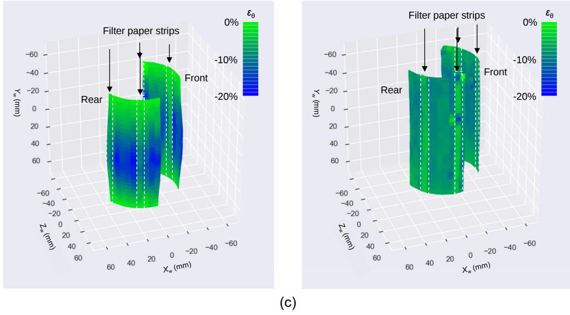
Figure 18: Strain distributions due to undrained triaxial compression: (a) Axial strain, \epsilon_a , (b) Radial strain, \epsilon_r , (c) Circumferential strain, \epsilon_\theta (Left: Non-lubricated Case NL, Right: Lubricated Case L).
