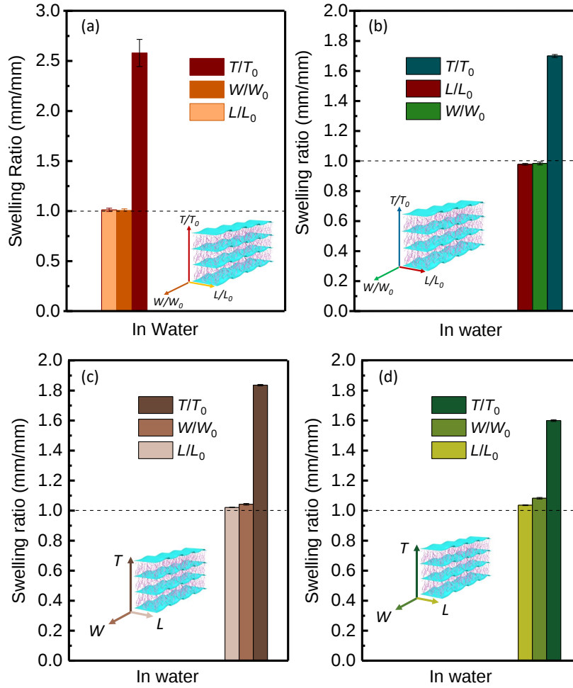
Figure 3.6 The swelling behavior of PDGI/PAAM bilayer hybrid gel thin film. The gel were synthesized using different space thicknesses (a) to (d) 0.5 mm, 100 \mu m, 50 \mu m, respectively. The gels thickness reaches in equilibrium condition as 1.29 mm, 170 \mu m and 90 \mu m and 80 \mu m, respectively. Along thickness axis (perpendicular to the bilayers) increases while it remains constant along the length axis (parallel to the bilayers), i.e. , no swelling at all, which indicates the superb anisotropic swelling. Where, L_0 , T_0 , W_0 ; and L , T , W are the length, thickness and width of the bilayer hybrid gels at as prepared state; and water swollen state, respectively.
