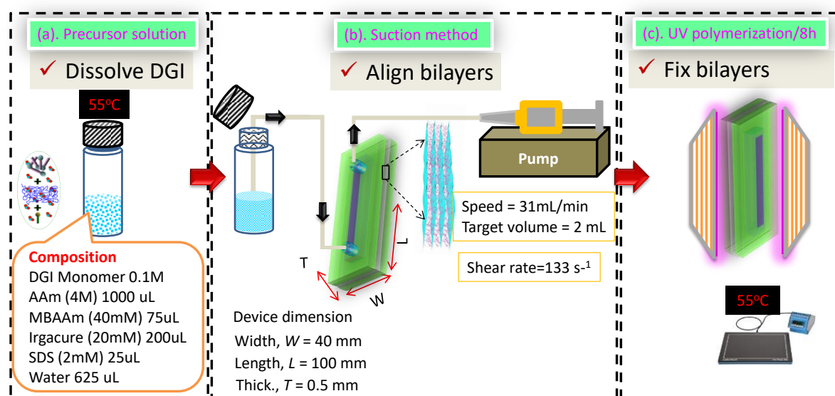
Figure 4.1.2 Schematics representation of anisotropic lamellar hydrogel. The method is comprise of three major steps. (a) Precursor solution preparation. (b) Applying suction to induce bilayer alignment by shear flow. (c) Polymerization by UV to start gelation for the bilayers fixing in hybrid gel. Temperature from solution to polymerization is constant.
