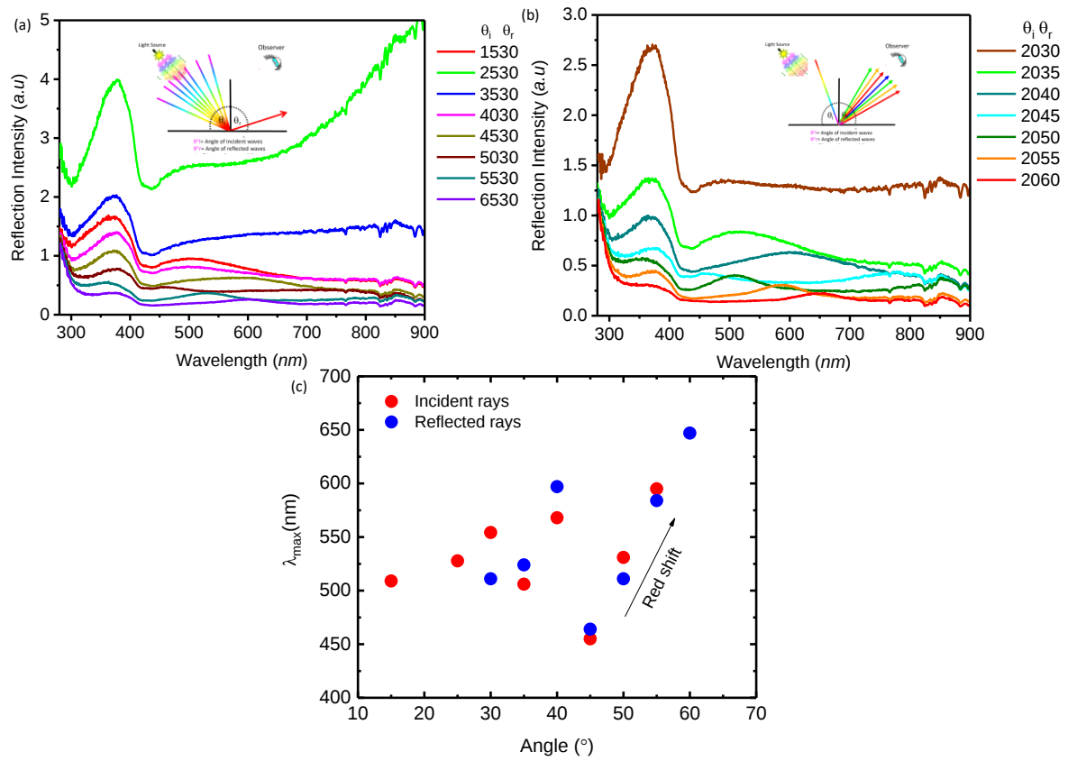
Figure 5.9 (a) Reflection spectra of PDGI/PAAm dry patterned sample at different angle of incident of light waves at constant viewing angle 30°. (b) Reflection spectra of PDGI/PAAm dry specimen at different angle of viewing angle at fix incident angle 20°. (c) Color tuning \lambda_{max} as a function of changing angle of incident and reflection.
