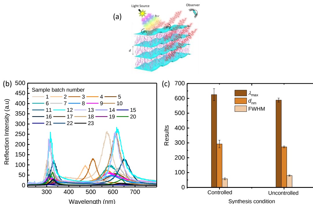
Figure 3.3 (a) Schematics of bilayer hybrid gel illuminated with high intensity white light for the collection of reflection spectra. The light was shined on surface of gel samples keeping Braggs angle of 60^\circ . (b) The gels reflection intensity as a function of wavelength nm in visible region of electromagnetic spectrum of light. (c) The average value of maximum wavelength of reflected color \lambda_{max} , the distance between bilayers d nm and full width at half maxima FWHM of the reflected color peaks of the controlled and uncontrolled condition gel synthesis, respectively.
