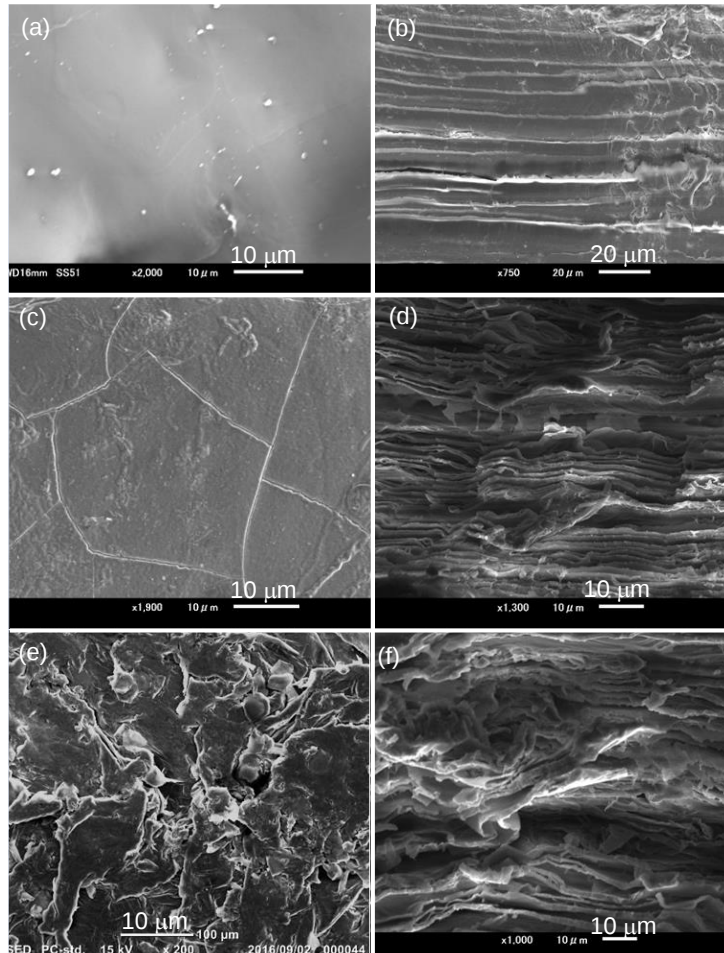
Figure 5.7 SEM micrographs of PDGI/PAAm samples. (a) & (b) Top view and cross-sectional view images of constrained air dry sample. (c) & (d) Top view and cross-sectional view images of sample pressed after drying. (e) & (f) PDGI/PAAm sample after applying random stress.
