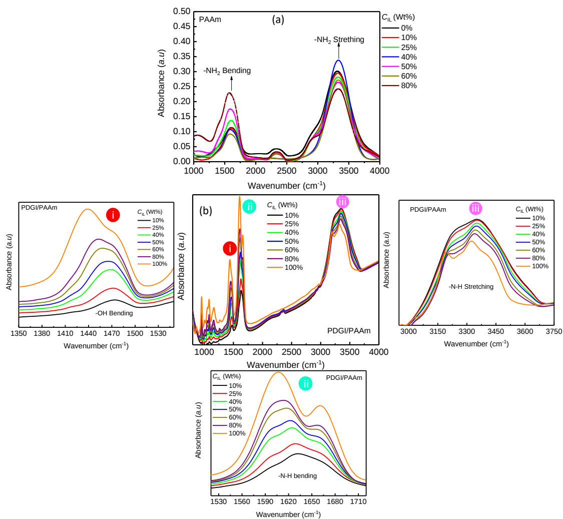
Figure 4.2.9 FTIR absorbance as a function of wavenumber 1000-4000 \text{cm}^{-1} at increasing ionic liquid concentration in co-solvent. (a) PAAm; (b) PDGI/PAAm. For clarity the PDGI/PAAm FTIR regions of interest are shown as an enlarged view (i)-(iii), respectively.
