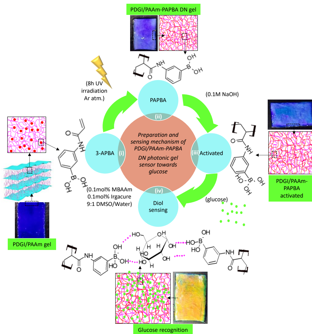
Figure 7.1 Schematics for the preparation of PDGI/PAAm-PAPBA DN photonic sensor. (i) Soaking PDGI/PAAm gel for 24h in monomer of 3-APBA solution. The monomer diffuses inside the PAAm gel layers. Then polymerization for 8h in inert argon atmosphere. (ii) After polymerization the PDGI/PAAm-PAPBA interpenetrating double network as prepared gel contains glucose recognition unit. (iii) Activating the gel for glucose sensing by placing in 0.1 M basic solution for 1 min without heating. (vi) Glucose sensing mechanism of the gel. Step (vi) to (ii) is reversible just by washing the sensor with distilled water.
