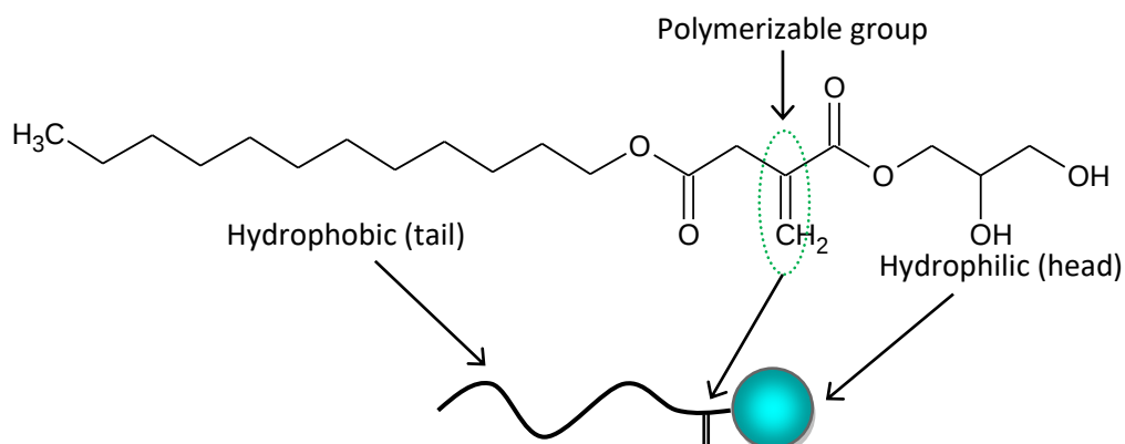
Figure 2.1: Chemical structure of amphiphilic surfactant DGI (dodecyl glyceryl itaconate) molecule.
