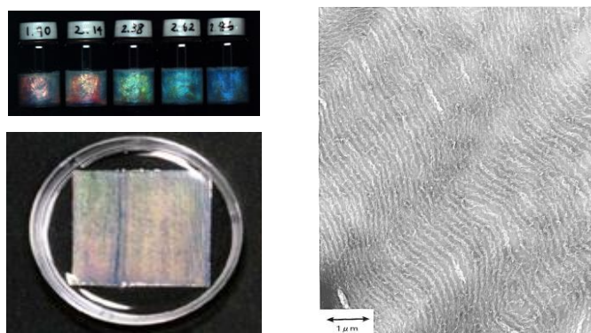
Figure 2.9: The photographs of the PDGI/PAAm gel prepared without shear flow (left-top) and at a shear flow of 0.5 mm/s (shear rate \sim 1 \text{ s}^{-1} ) (left-bottom). Freeze-fracture transmission
