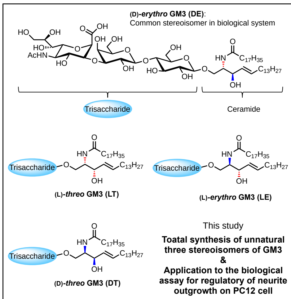
Figure 1. Structures of common GM3 structure in biological system and unnatural three stereoisomers of GM3.
