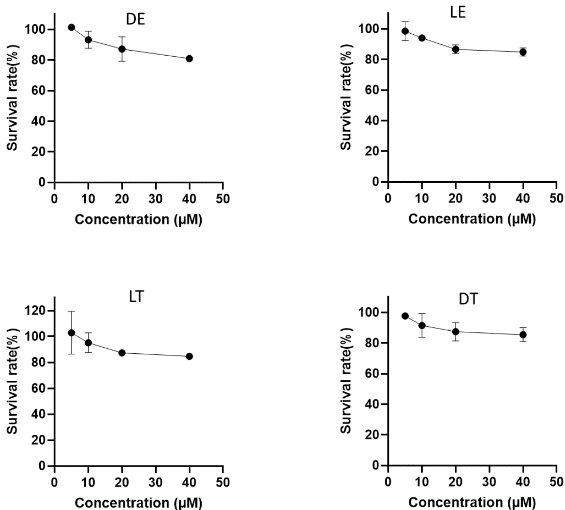
Figure 2. Viability assays of PC12 cells exposed to three stereoisomers of GM3 and control normal (D)-erythro GM3. Cell viability were tested after 24 hours of treatment with four compounds at concentration levels of 5-40 \mu\text{M} . Data are presented as the mean \pm standard deviation (SD).
