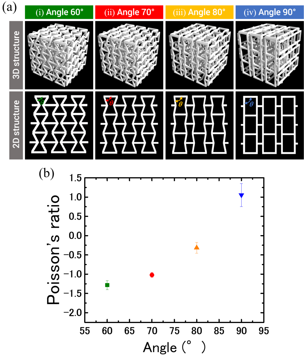
Figure 6.7 | 3D architectures of reinforcing phase with controllable Poisson's ratio (a) Schematic illustration of lattice-like 3D architectures determined by the interior angle, \theta . (b) Relationship between Poisson's ratio of grid, \mu and interior angle, \theta . The green, red, yellow, and blue dots represent the 60°, 70°, 80°, and 90° of interior angle in the shape of reinforcing phase, respectively. The Poisson's ratios are estimated from the ratio of transverse extension strain to longitudinal compression strain in the direction of compressive force (compression strain: \sim 1.1 ).
