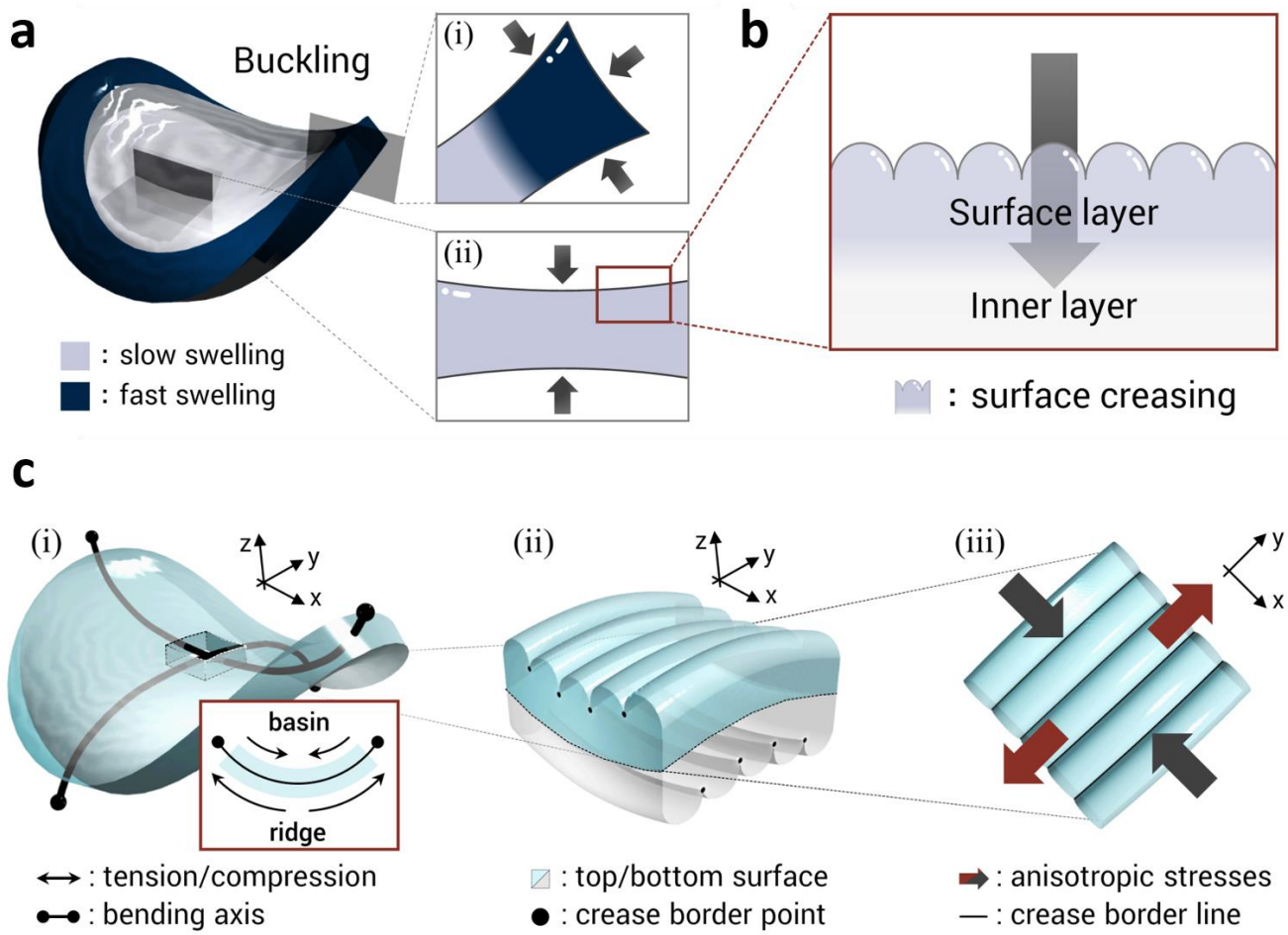
Figure 4.3 | Schematic illustration of two kinds of swelling mismatch and their coupling to induce anisotropic surface creases during fast free swelling of a polyelectrolyte gel. (a) Swelling mismatch between the annulus (dark blue) and the inner disc (light blue) induced by the difference in swelling kinetics between the annulus and the inner disc. The annulus can absorb water from three directions (a-i), while the inner disc can only absorb water from two directions (a-ii) as shown by arrows in (a-i, ii). This swelling mismatch induces a saddle-like bending to minimize the swelling mismatch. (b) Swelling mismatch between the surface layer (light blue) and inner layer (gray) induced by the difference in swelling kinetics between the surface layer and the inner layer. Surface creasing instability is induced to minimize this swelling mismatch. (c) The two mechanical instabilities are coupled to induce anisotropic surface crease pattern. Bending of the sample exerts a tension to the ridge and a compression to the basin (c-i). The saddle-like bending induces anisotropic stresses, perpendicularly oriented, on the two surfaces of the sample (c-ii), which changes the isotropic polygonal crease patterns into the anisotropic stripe crease patterns aligned in right angles on the two surfaces (c-iii).
