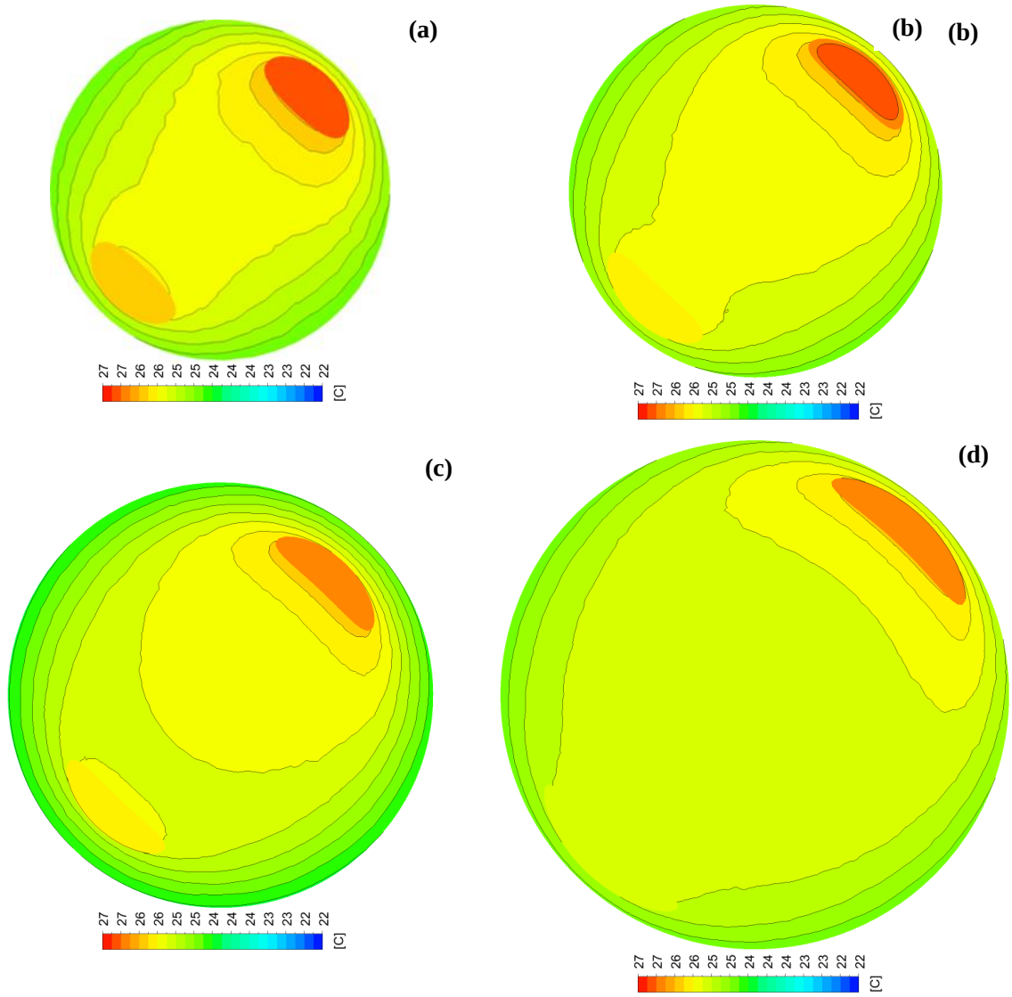
Fig. 29. Temperature contours on a horizontal plane at a depth of 10 m at different borehole diameters: (a) 180, (b) 240, (c) 300, and (d) 360 mm
