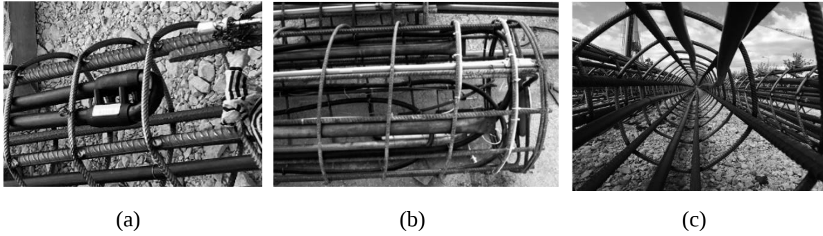
Fig. 3. Installation procedure and difficulties of GHX (a) Thermally welded U-bend, (b) Pipe bending at the end edge of the GHX, and (c) Multi-U tubes fixed by a steel cage
