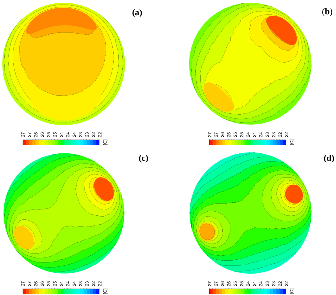
Fig. 21. Temperature contours on a horizontal plane at a 10 m depth for a) 0.05 m, b) 0.1 m, c) 0.15 m, and d) 0.2 m pitch
