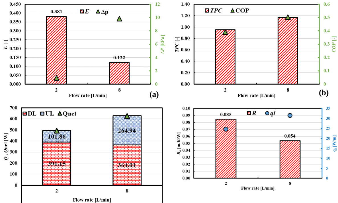
Fig. 22. Effect of different flow rates on (a) E and \Delta P , (b) TPC and COP , (c) Q and Q_{net} and (d) R and q_l
