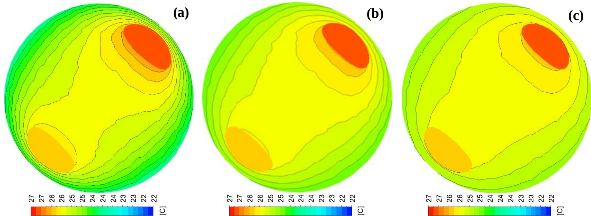
Fig. 27. Temperature contours on a horizontal plane at a 10 m depth at different grout
