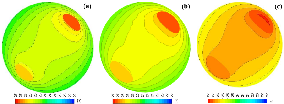
Fig. 25. Temperature contours on a horizontal plane at a 10 m depth at a (a) 20, (b) 26, and (c) 30 mm tube diameter
