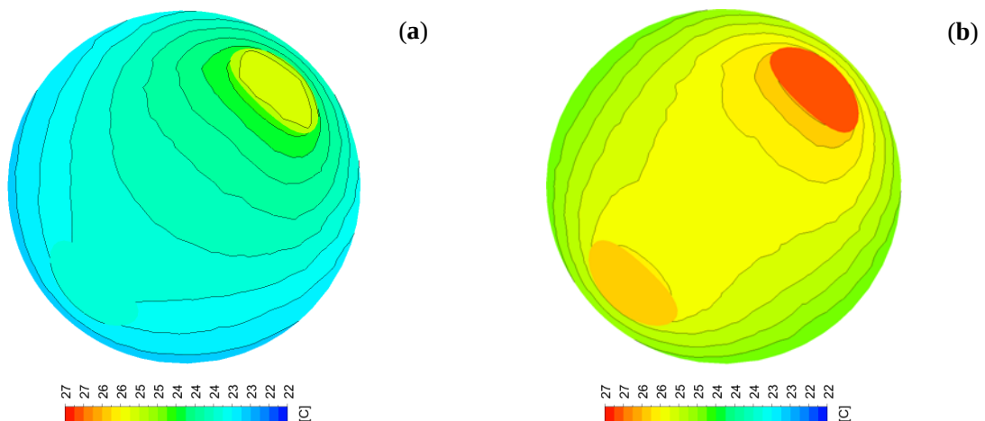
Fig. 23. Temperature contours on a horizontal plane at a 10 m depth at (a) 2 L/min and (b) 8 L/min
