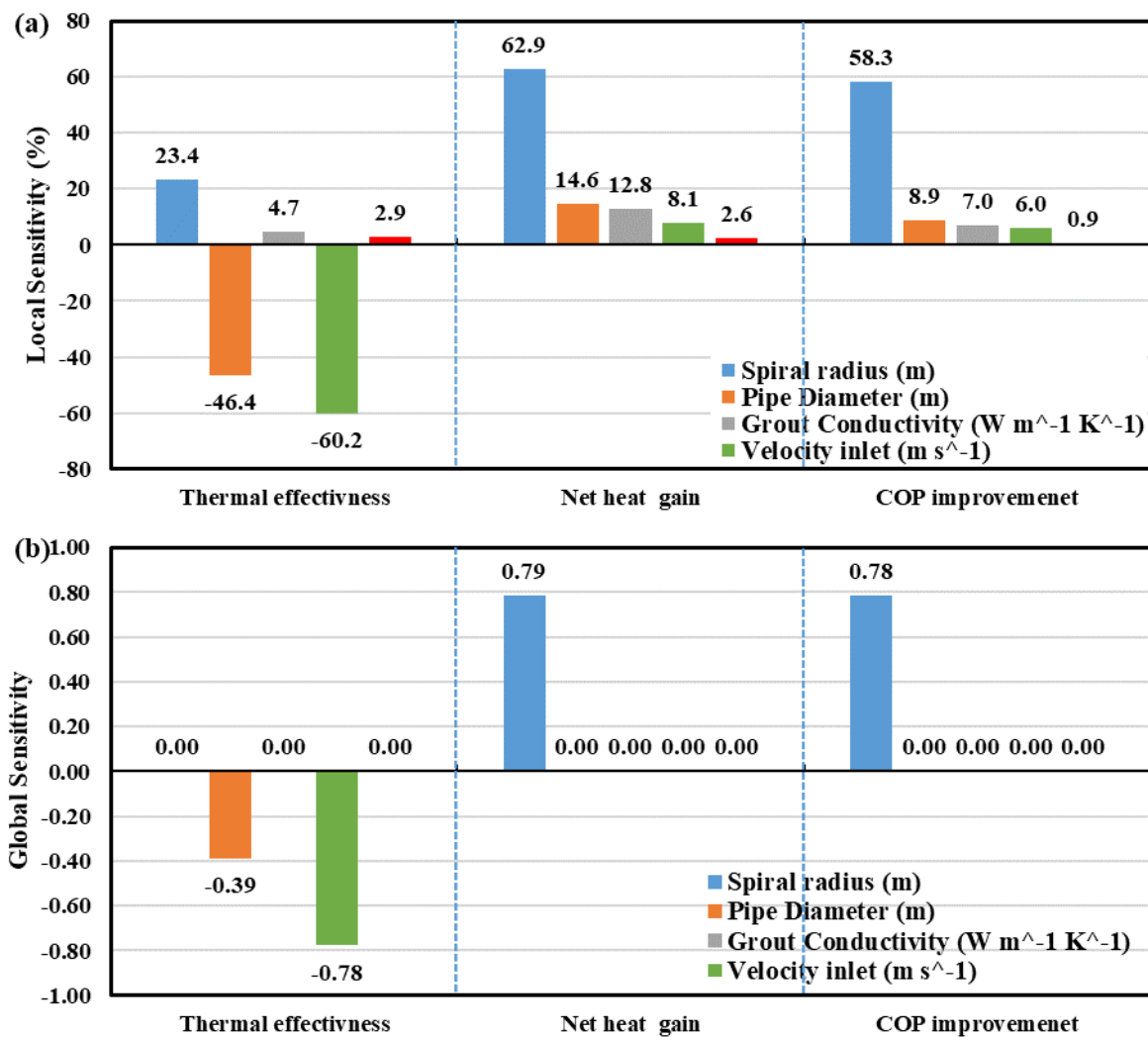
Fig. 31. a) Local and b) global sensitivity analyses
