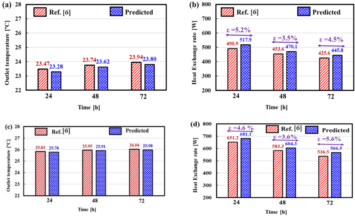
Fig. 12. Comparison of current predicted results with the numerical results indicated by [6] for spiral GHX at (a) fluid outlet temperature under the flow rate of 2 L/min, (b) heat exchange rate under the flow rate of 2 L/min, (c) fluid outlet temperature under the flow rate of 8 L/min, and (d) (b) heat exchange rate under the flow rate of 8 L/min
