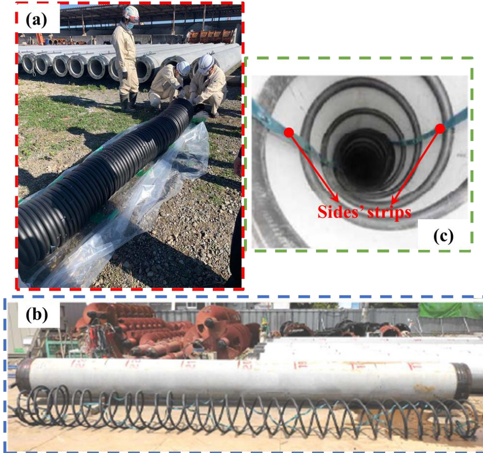
Fig. 2 The new spiral-double GHX (a) Folded form, (b) elongated form, and (c) the supporting sides' strips
