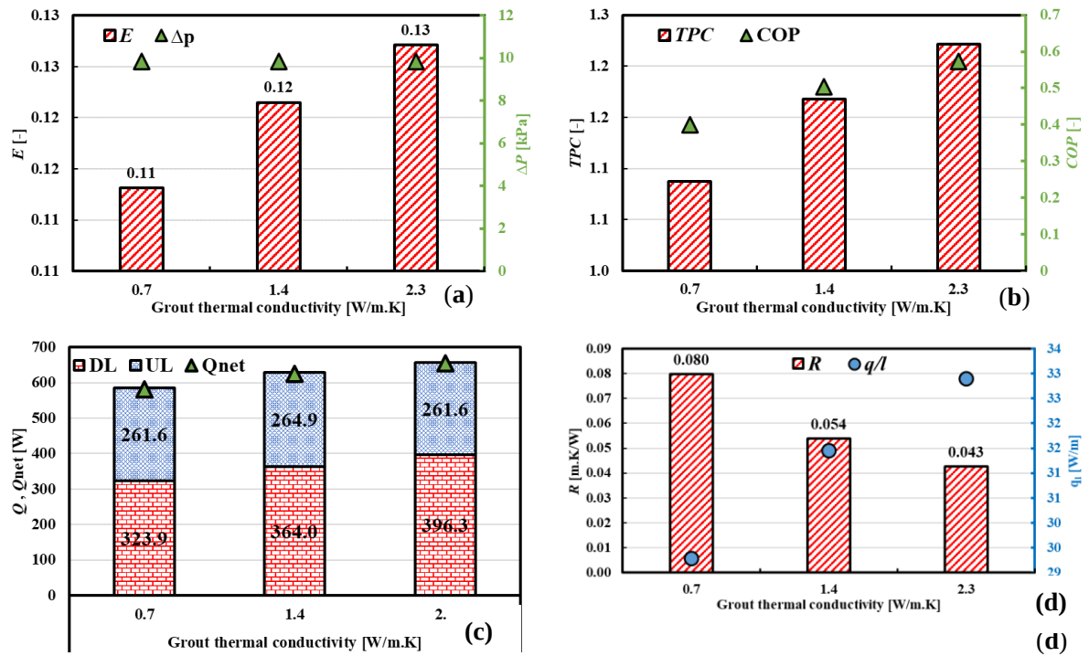
Fig. 26. Impact of grouting thermal conductivities on (a) E and \Delta P , (b) TPC and COP , (c) Q_{net} and Q_{net} and (d) R and q/l
