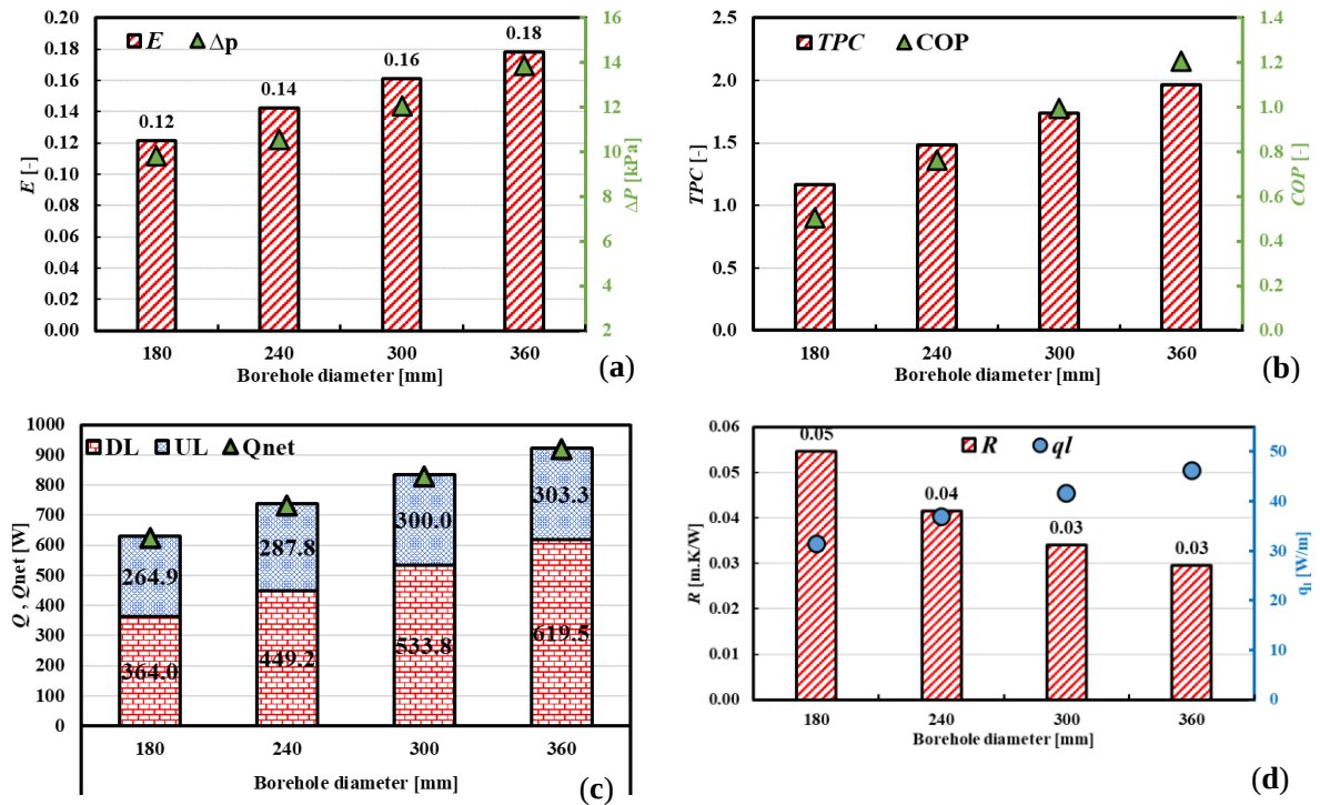
Fig. 28. Impact of borehole diameter on (a) E and \Delta P , (b) TPC and COP , (c) Q and Q_{net} and (d) R and q_l
