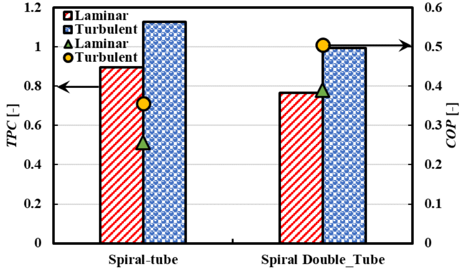
Fig. 18. Comparison of TPC and COP improvement between spiral and spiral-double GHXs under different flow rates
