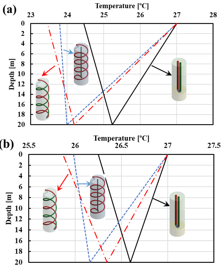
Fig. 15. Fluid temperature profile comparison for (a) laminar and (b) turbulent flow conditions
