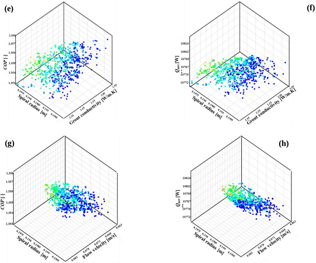
Fig. 33. Trade-off charts for each parameter on each output (a, c, e, and g) COP and (b, d, f, and h) Q_{net} . The blue color indicates a possible feasible value
