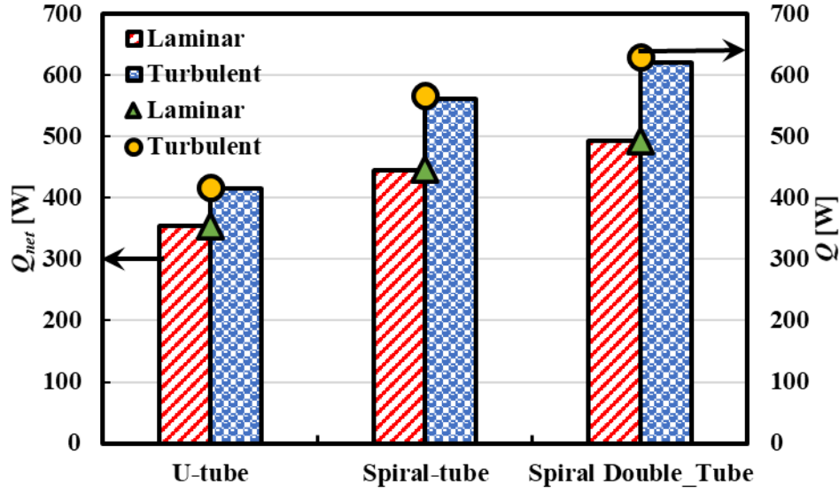
Fig. 17. Total and net heat energy rejected by GHXs under different flow rates
