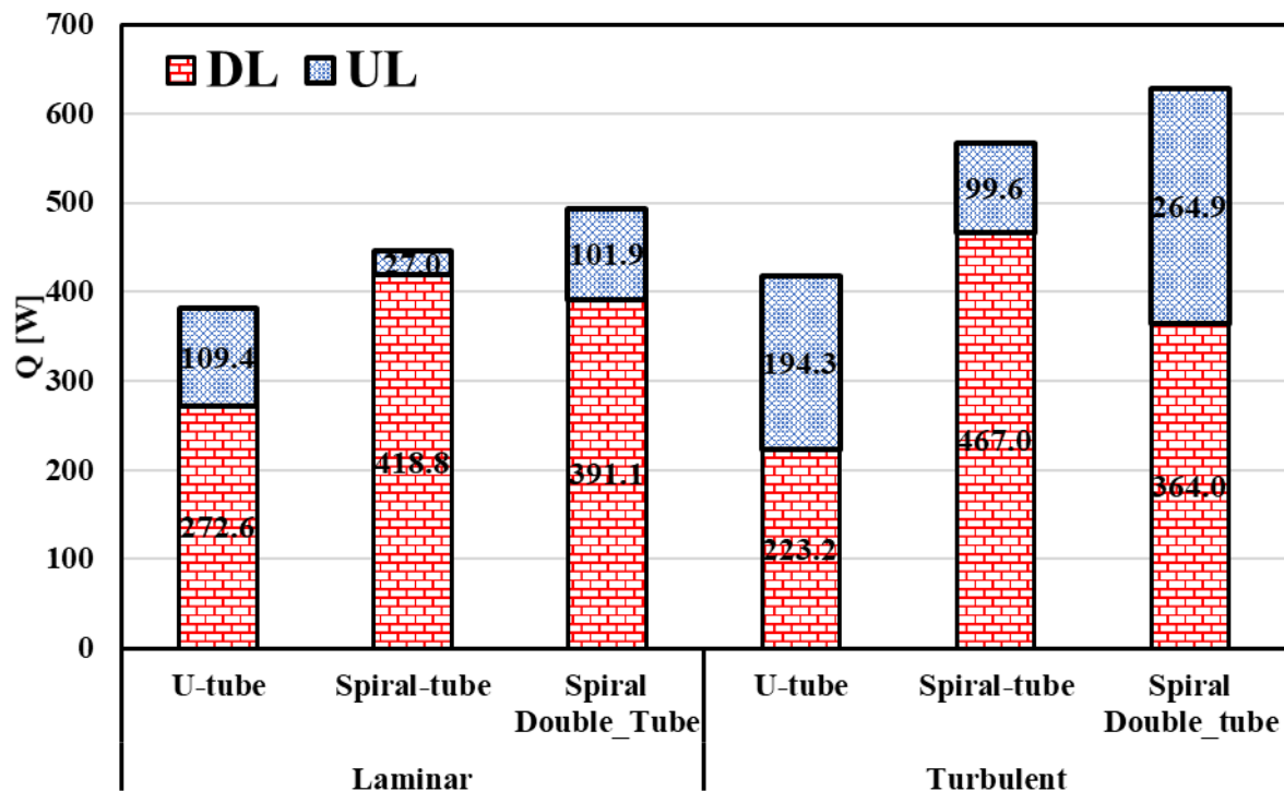
Fig. 16. Heat transfer rate in each tube leg for flow rates of laminar and turbulent flow conditions
