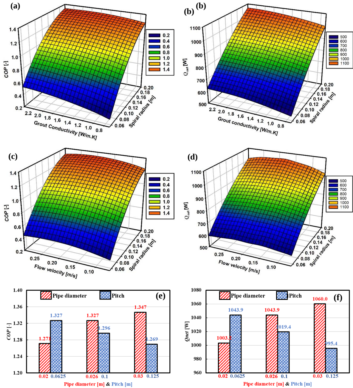
Fig. 30. Surface response of each output (a, c, and d) COP_{improvement} and (b, d, and f) Q_{net}
