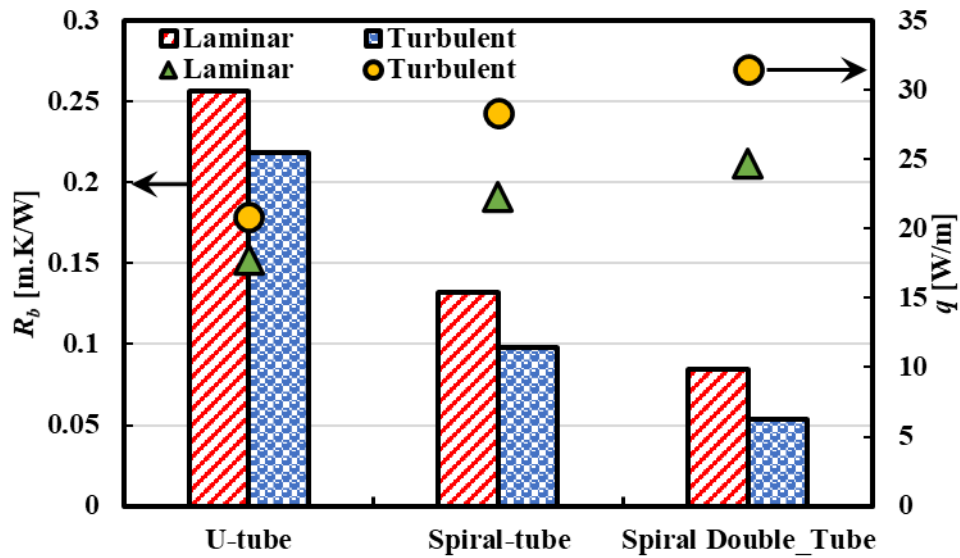
Fig. 19. Thermal resistance of single-U tubes, spiral, and spiral-double GHXs at different flow rates
