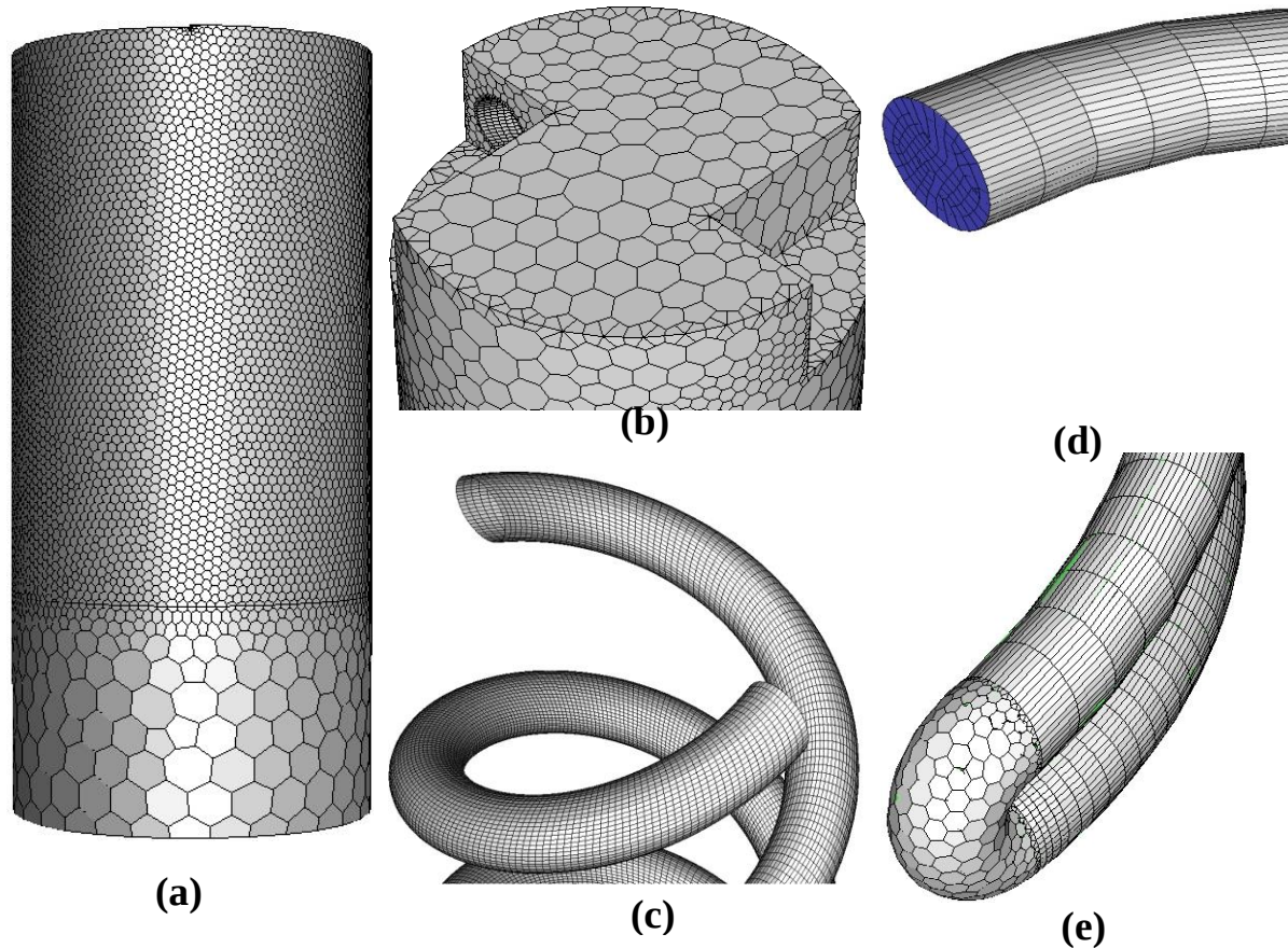
Fig. 7. Mesh elements used for each domain a) soil, b) grouting, c) fluid, d) inlet, and e) U-bend
