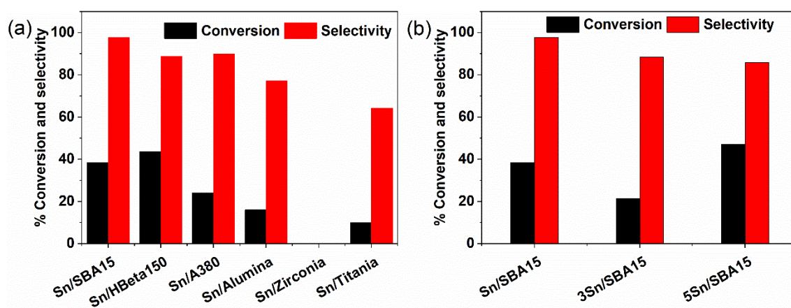
Fig. 1. Fructose selectivity and glucose conversion in the presence of (a) 1 wt. % Sn catalyst using different supports and (b) catalyst with different Sn loading over SBA15. Reaction conditions: 90 mg glucose, 90 mg catalyst, 7 mL ethanol, 90 °C, 45 minutes.
