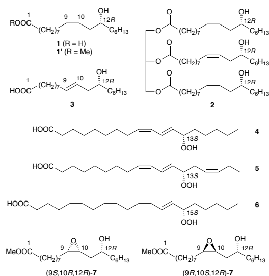
Scheme 1 Structures of chiral oxidized lipids studied in this work: ricinoleic acid ( 1 ), methyl ricinoleate ( 1' ), ricinolein ( 2 ), ricinelaic acid ( 3 ), 13-HpODE ( 4 ), 13-HpOTE ( 5 ), 15-HpETE ( 6 ), and methyl 9,10-epoxy-12-hydroxyoctadecanoate ( 7 ).
