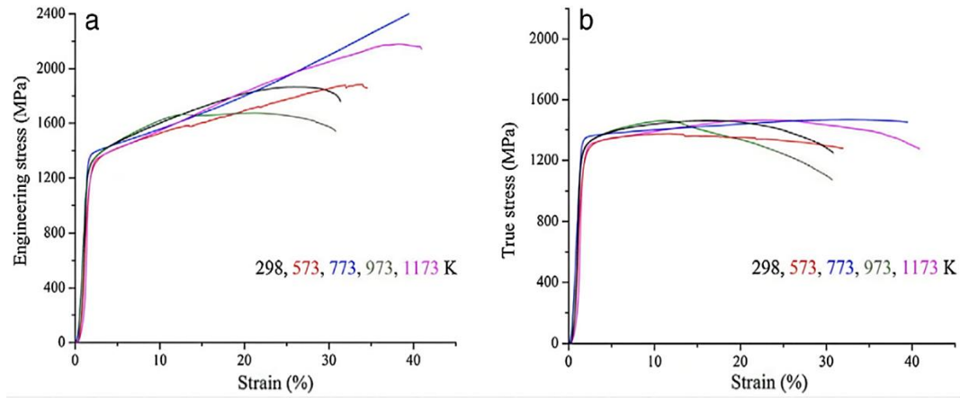
Fig. 1.9 Engineering stress and true stress vs. strain compression curves for the Ti 20 Zr 20 Hf 20 Nb 20 V 20 (a,b) and Ti 20 Zr 20 Hf 20 Nb 20 Cr 20 alloys in the as-cast state.
