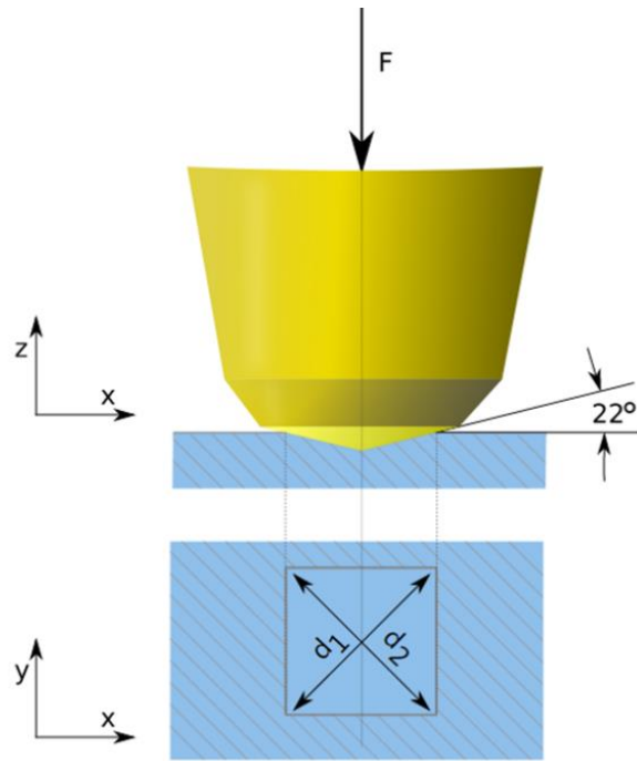
Fig. 2.3 Vickers test scheme
