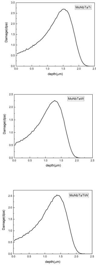
Fig. 3.2 Depth profile of damage induced by irradiation with 6.4 MeV \text{Fe}^{3+}
