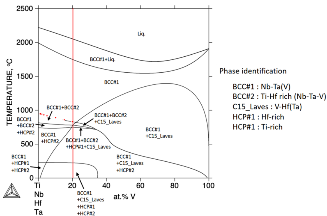
Fig. 4.1 Phase diagram for HfNbTaTiV
