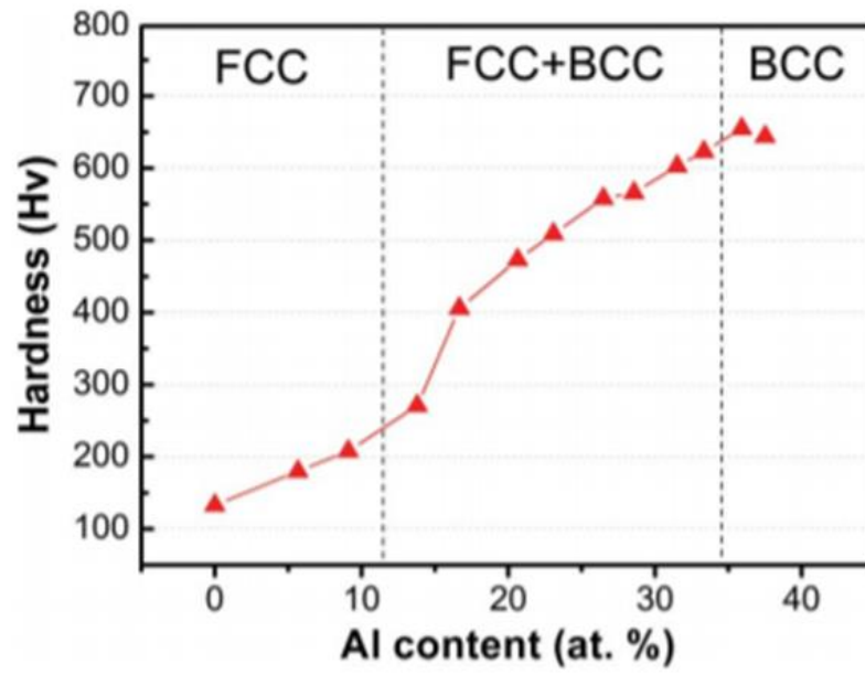
Fig. 1.6 Hardness of the \text{Al}_x\text{CoCrCuFeNi} alloys as a function of Al content.
