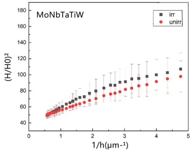
Fig. 3.10 Nix-Gao model for three HEAs after ion irradiation.
