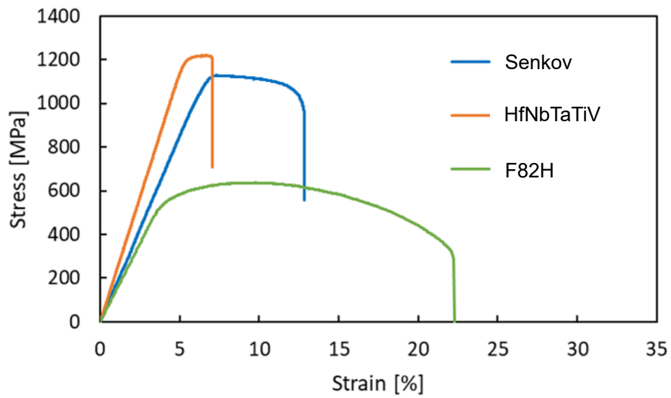
Fig. 4.6 Stress-strain curves of HfNbTaTiV, Senkov alloy, and F82H.
