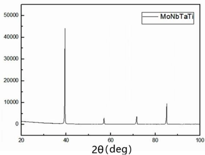
Fig.3.3 XRD patterns for the three high-entropy alloys after heat-treatment
