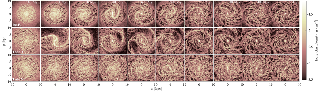
(a) Gas density distribution for all gas particles in the simulation.
