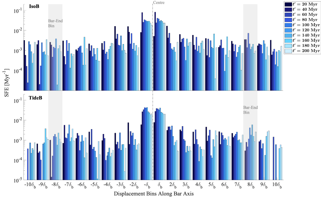
Figure 4.8: Azimuthally averaged SFE along the bar-axis for IsoB and TideB for the period immediately post-bar formation ( 0 < t' < 200 ). The bar-axis is defined by a co-rotating co-ordinate system to always align with the x -axis and the bar width is set to y \pm 1 kpc. As bar-length differs for each disk, a consistent number of bins is used creating a fractional bar element ( \delta_b ). These are numbered outwards from the centre. The time evolution of SFE is mapped via colour saturation with evolution from dark to light and bars at every 20 Myr. Again, the bin containing the bar extent is shaded in grey (Iles et al., 2022).
