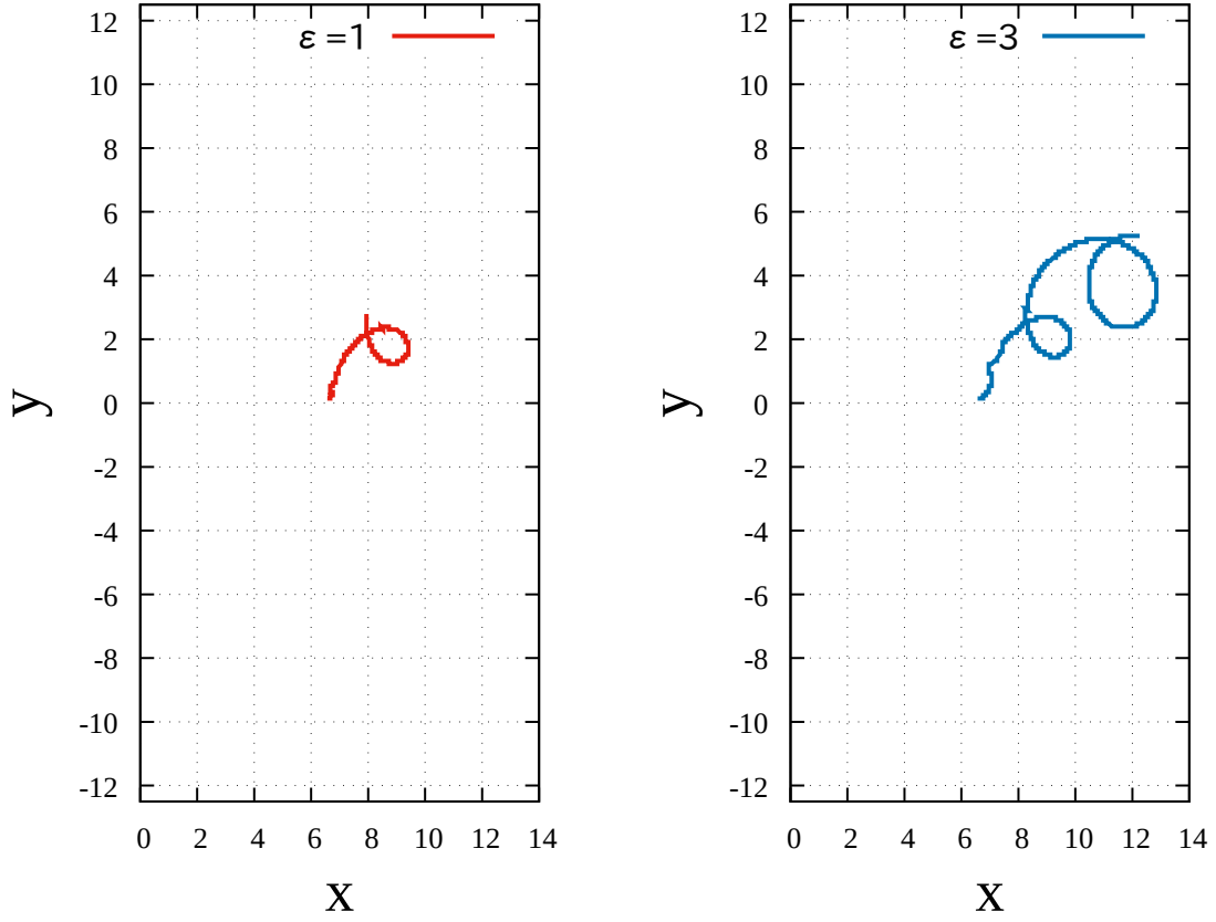
Fig. 3.7: The trajectory of the anticyclonic upper-layer eddy in the case of \varepsilon = 1 (left) and \varepsilon = 3 (right). Other parameters are the same as in figure 3.6. In both panels, the initial position of the upper-layer eddy is (X_{c,0}, Y_{c,0}) = (6.5, 0) .
