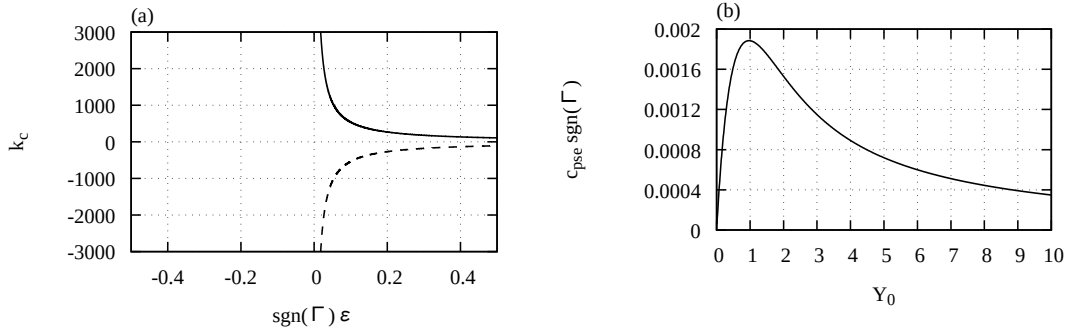
Fig. 2.3: (a) The dependencies of the wavenumbers, k_c , which satisfy c = c_{pse} on \text{sgn}(\Gamma)\varepsilon for Y_0 = 1 and is calculated from (2.36) and (2.43). Since c is a function of k^2 , there are both positive and negative k_c . As \text{sgn}(\Gamma)\varepsilon \rightarrow 0 , |k_c| diverges to infinity. (b) The dependence of the propagation velocity, c_{pse} , on Y_0 . The propagation velocity has a maximum at approximately Y_0 = 0.7 . In both panels, \gamma_H = 1 and \gamma_L = 10^{-3} .
