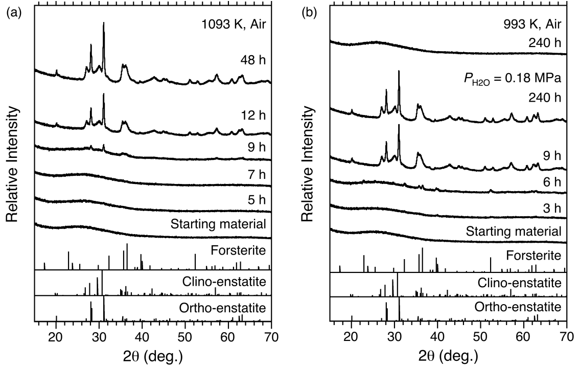
Fig. 2.2b Time evolutions for XRD patterns of the samples heated at 1093 K in air ( P_{\text{H}_2\text{O}} \sim 10^2 Pa) and at 993 K under P_{\text{H}_2\text{O}} of 0.18 MPa for different durations (a~b). A XRD pattern of the sample heated at 993 K in air for 240 h (b). Typical peaks of clino/ortho-enstatite and forsterite are also given for references.
