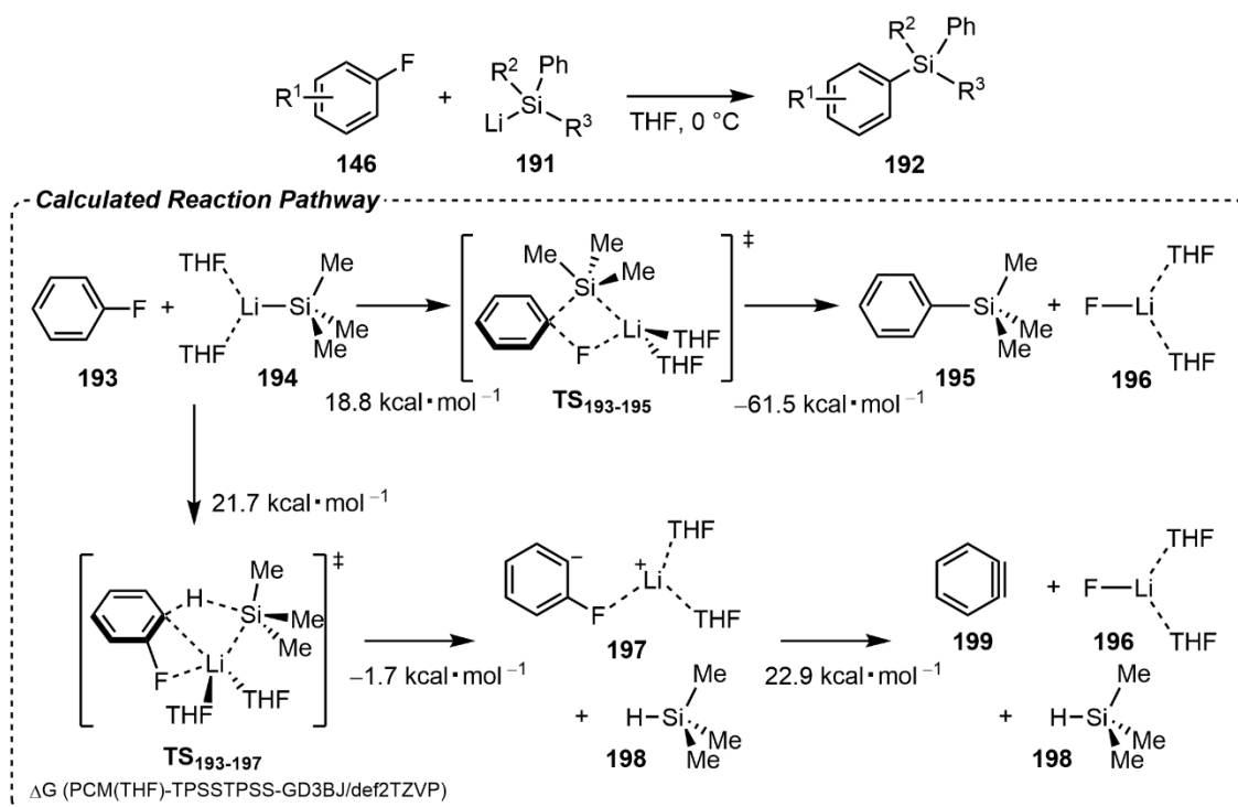
Scheme 1.31. Studer's work on the defluorosilylation of aryl fluorides.
