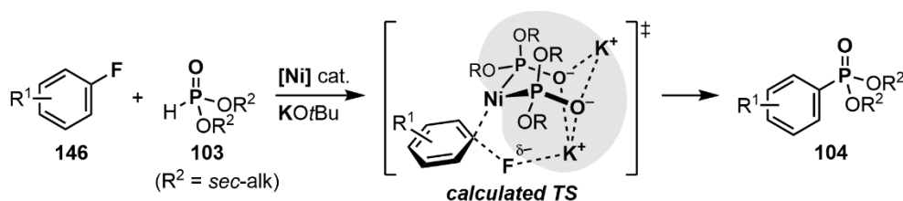
Scheme 1.39. Ni-catalyzed phosphonylation of aryl fluorides.
