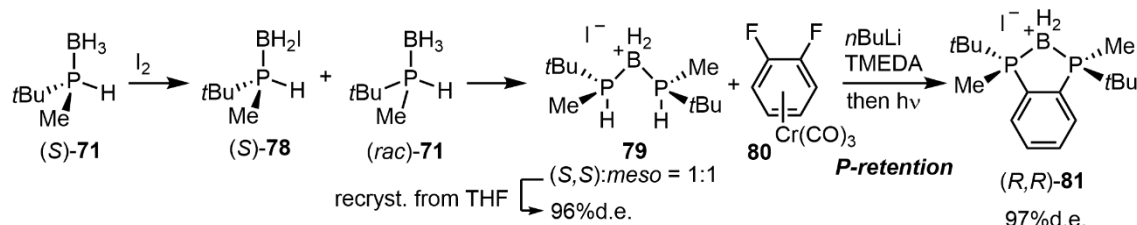
Scheme 1.12. Phosphine–borane salts as nucleophiles.
