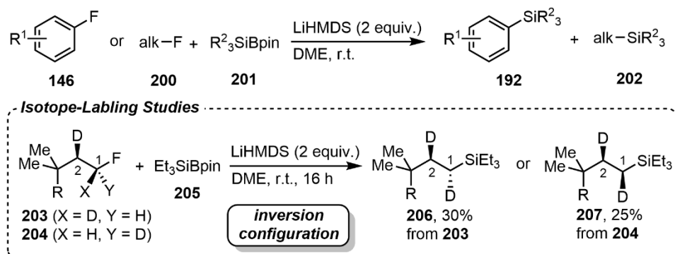
Scheme 1.32. Martin's work on the defluorosilylation of aryl fluorides.
