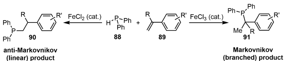
Scheme 1.15. Iron-enabled tunable selectivity in hydrophosphination.
