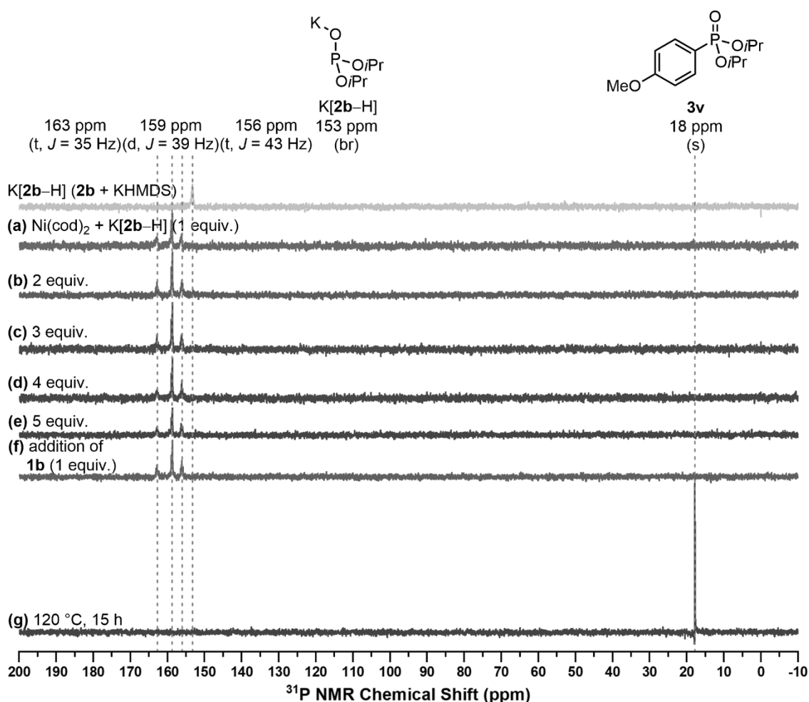
Figure 3.22. ^{31}\text{P}\{^1\text{H}\} NMR spectra of the complexation experiment in \text{PhMe-}d_8 .
