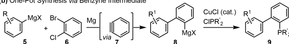
Scheme 1.1. Preparation of biaryl phosphine ligands.
