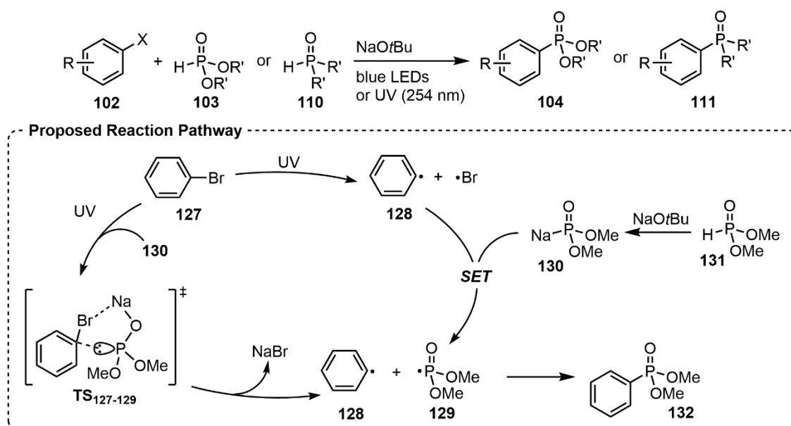
Scheme 1.21. Catalyst-free Hirao coupling enabled by photo-irradiation.
