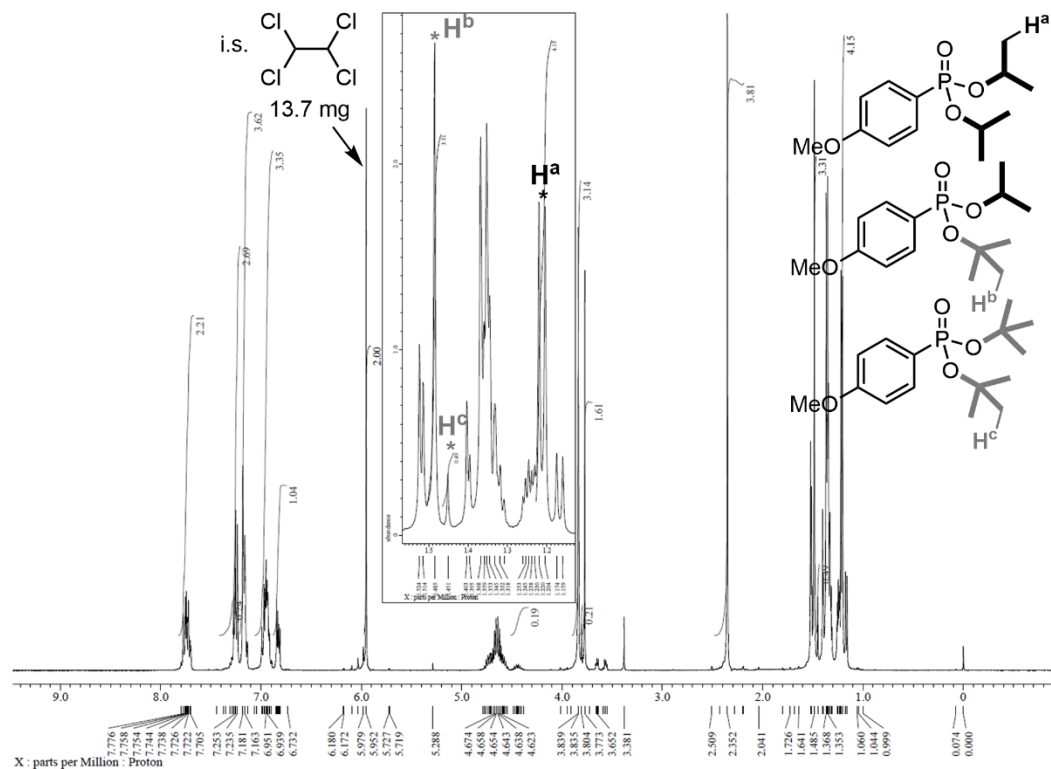
Figure 3.19. ^1H NMR spectrum of the crude reaction mixture in Scheme 3.6 (eq.3).
