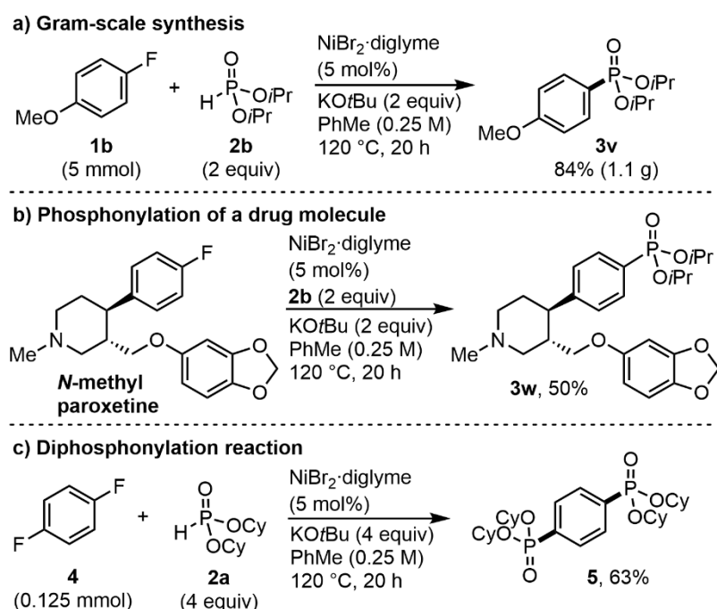
Scheme 3.2. Synthetic applications.
