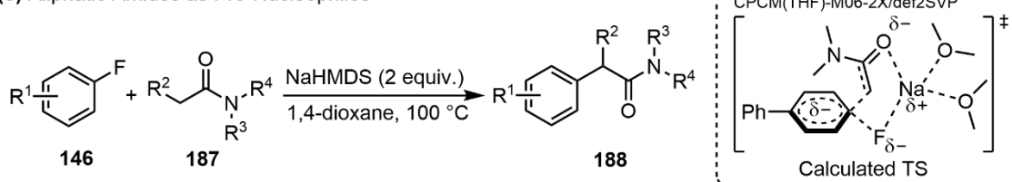
Scheme 1.29. S_NAr of non-activated aryl fluorides with carbon-centered nucleophiles.
