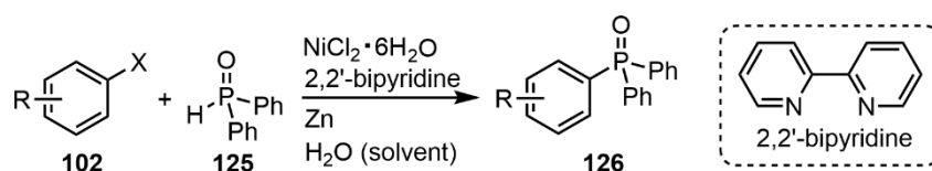
Scheme 1.20. Ni-catalyzed Hirao coupling in water.
