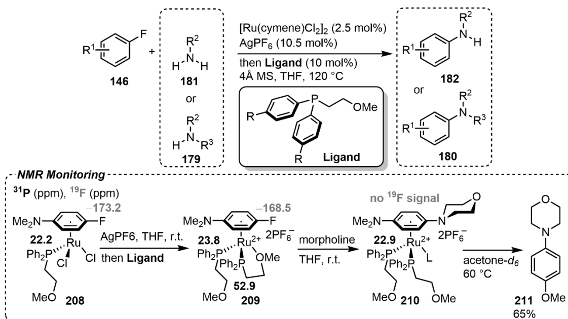
Scheme 1.33. Catalytic \text{S}_{\text{N}}\text{Ar} amination of aryl fluorides.
