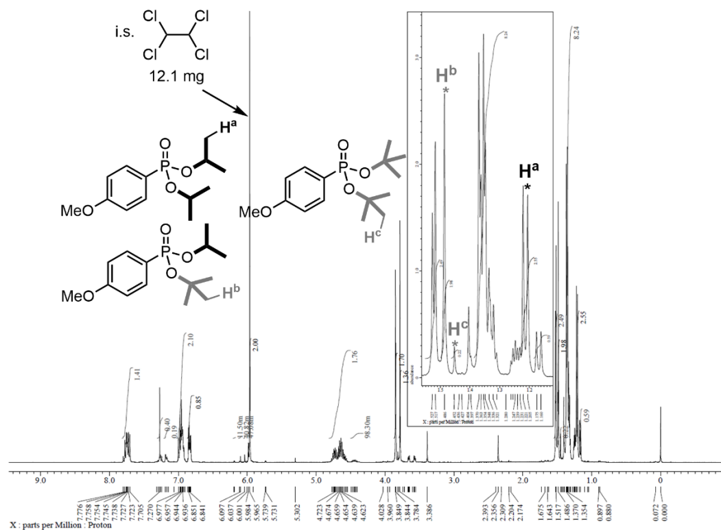
Figure 3.18. ^1H NMR spectrum of the crude reaction mixture in Scheme 3.6 (eq.2).
