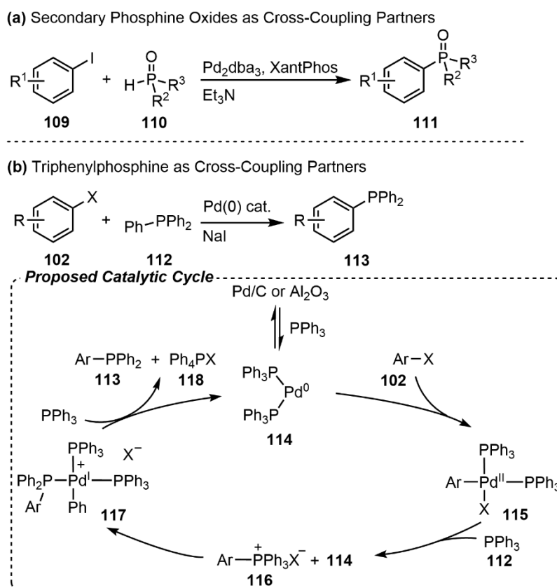
Scheme 1.18. Exploring other phosphorus cross-coupling partners.
