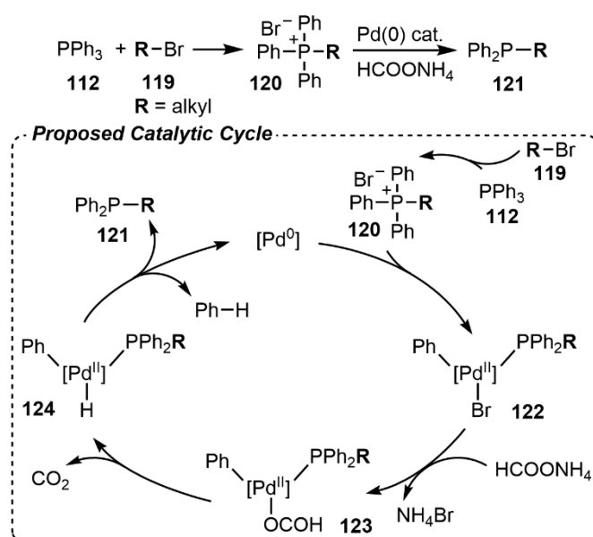
Scheme 1.19. Preparation of alkyl diphenylphosphines from phosphonium salts.
