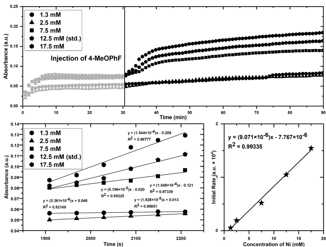
Figure 3.15. The \text{Ni}(\text{cod})_2 concentration effect on the reaction kinetics.
