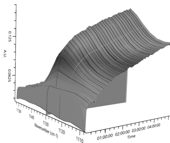
Figure 3.12. In situ FT-IR waterfall plots of 3b around 1130 \text{cm}^{-1} .
