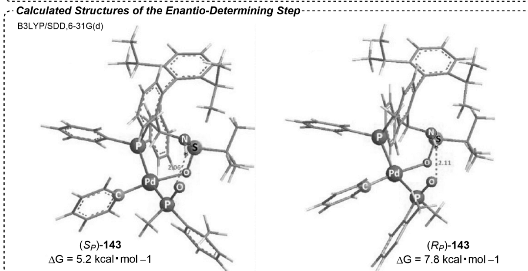
Scheme 1.23. XiaoPhos-enabled catalytic construction of P -chirogenic center by asymmetric Hirao coupling.
