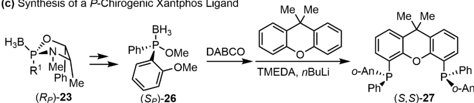
Scheme 1.3. Ephedrine as a chiral auxiliary for P -chirogenic compound synthesis.
