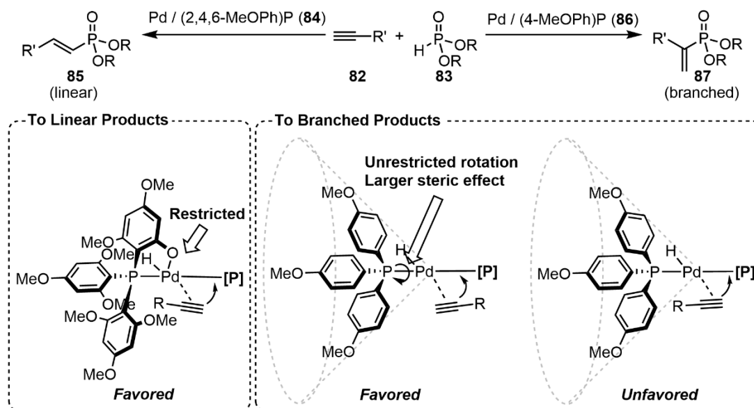
Scheme 1.14. Ligand-controlled selectivity between linear and branched hydrophosphonylation.
