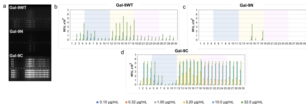
Figure S8. Fluorescence image of core M1 \alpha -DG glycopeptide printed microarray chip taken after treatment with 10.0 \mu\text{g/mL} galactin solution (a) and relative interaction of 200 \mu\text{M} core M1 \alpha -DG glycoconjugates with 0.10 \mu\text{g/mL} to 32.0 \mu\text{g/mL} Gal-9WT (b), Gal-9N (c), and Gal-9C (d).
