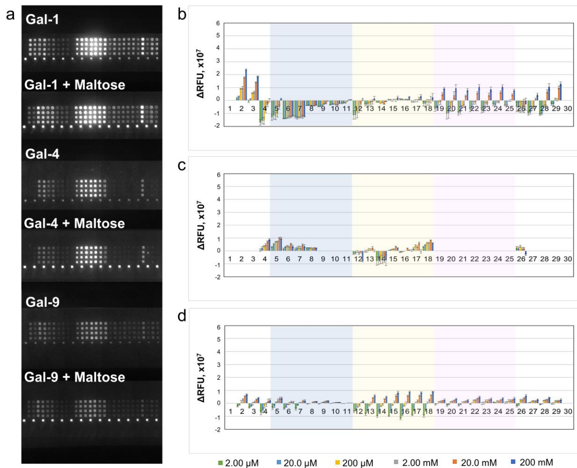
Figure S9. Fluorescence image of microarray chip is taken after treatment of 10.0 \mu g/mL lectin solution with 200 mM maltose ( a ) and relative binding properties of 200 \mu M core M1 \alpha -DG glycopeptides Gal-1 ( b ), Gal-4 ( c ), and Gal-9 ( d ) with the presence of 2.00 \mu M to 200 mM maltose.
