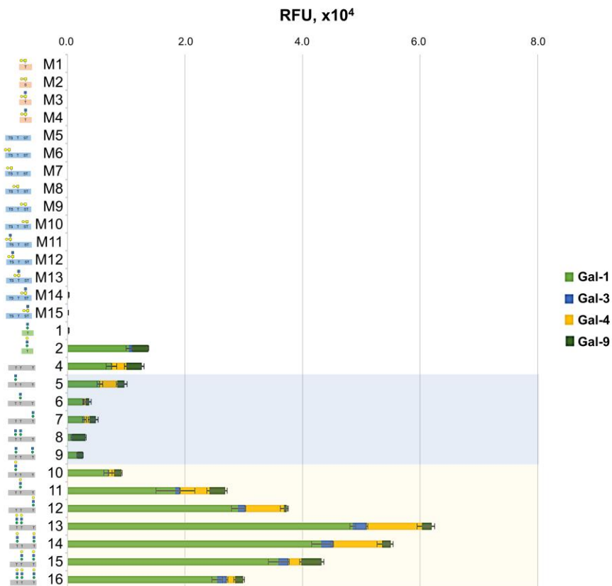
Figure S3. Synthetic MUC1 and \alpha -DG core M1 glycopeptides used for preliminary microarray experiments. (I.) Fluorescence image of microarray chip of selected galactose-terminated MUC1 and \alpha -DG glycopeptide peptide library taken after treatment with 10.0 \mu\text{g/mL} galectin solution (a) and relative interaction of 200 \mu\text{M} glycopeptides with 0.10 \mu\text{g/mL} to 32.0 \mu\text{g/mL} ConA (b), PNA (c), Gal-1 (d), Gal-3 (e), Gal-4 (f), and Gal-9 (g). (II.) Stacked chart of signal intensities of 200 \mu\text{M} of selected MUC1 and core M1 \alpha -DG glycopeptides with 3.20 \mu\text{g/mL} of galectins. The synthesis and characterization of MUC1 glycopeptides used in this study is reported elsewhere 2,3 .
