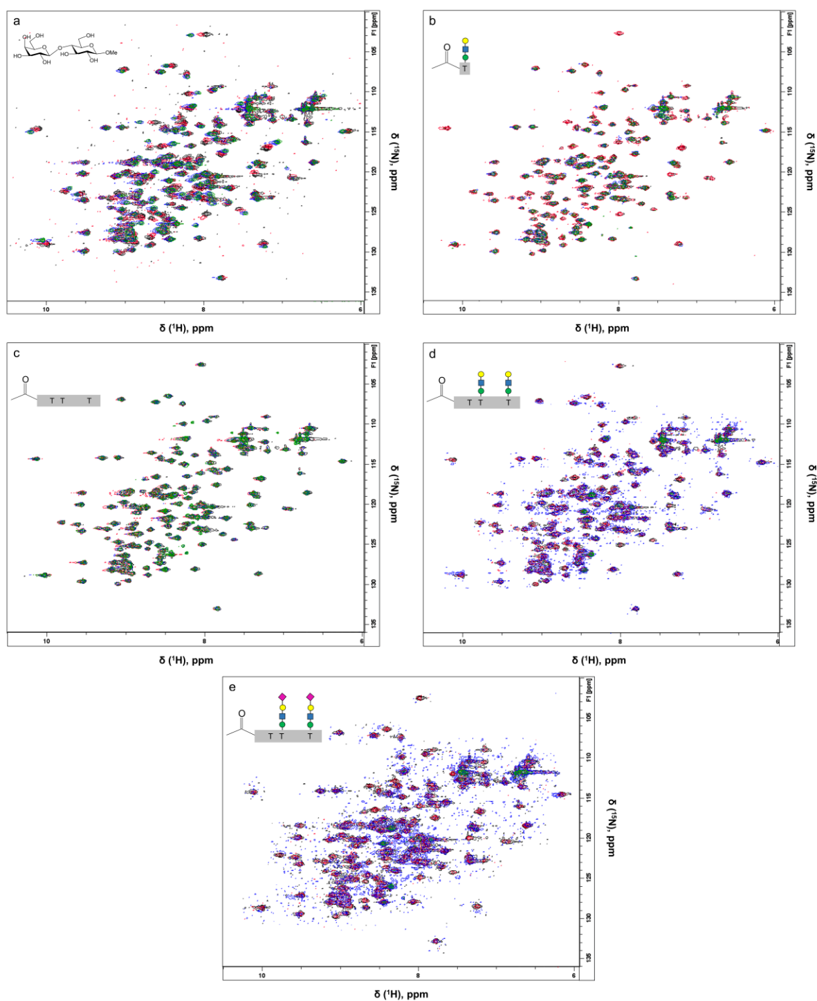
Figure S2. Overlaid ^1\text{H} - ^{15}\text{N} HSQC spectra of reduced Gal-1 (100 \mu\text{M} ) alone ( black peaks) and in the presence of methyl- \beta -lactoside (molar ratio 1:1 blue peaks, 1:16 red peaks, and 1:64 green peaks a ), LacNAc-terminated glycoamino acid 31 (molar ratio 1:1 blue peaks, 1:32 red peaks, and 1:64 green peaks b ), unglycosylated peptide 32 (molar ratio 1:1 blue peaks, 1:16 red peaks, and 1:64 green peaks c ), LacNAc-terminated glycopeptide acid 33 (molar ratio 1:0.125 blue peaks, 1:1 red peaks, and 1:2 green peaks d ), sialyl-LacNAc-terminated glycopeptide 34 (molar ratio 1:0.125 blue peaks, 1:1 red peaks, and 1:2 green peaks e ). Solution condition were 20 mM potassium phosphate buffer, pH 6.9, 50 \mu\text{M} EDTA, with 10 mM DTT made up using a \text{H}_2\text{O}/\text{D}_2\text{O} (95:5%).
