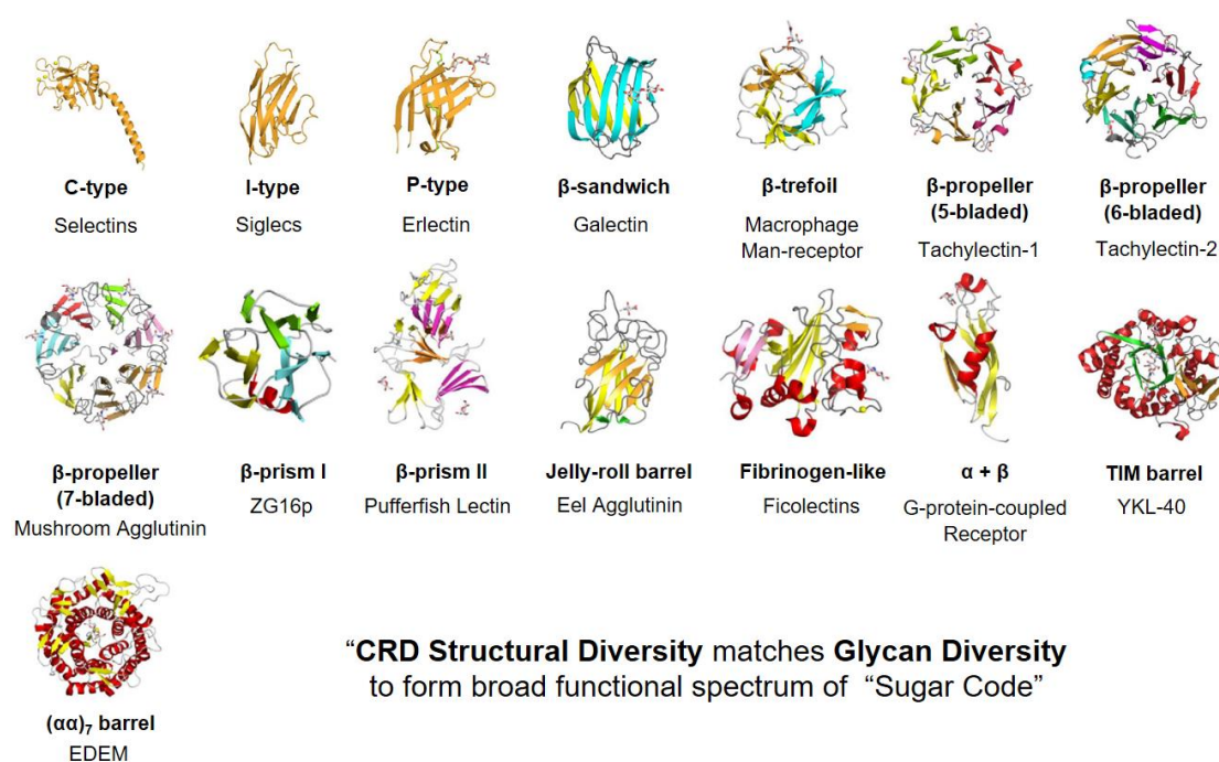
Figure 1. Diversity of folding within the superfamily of lectins (6)(7).
