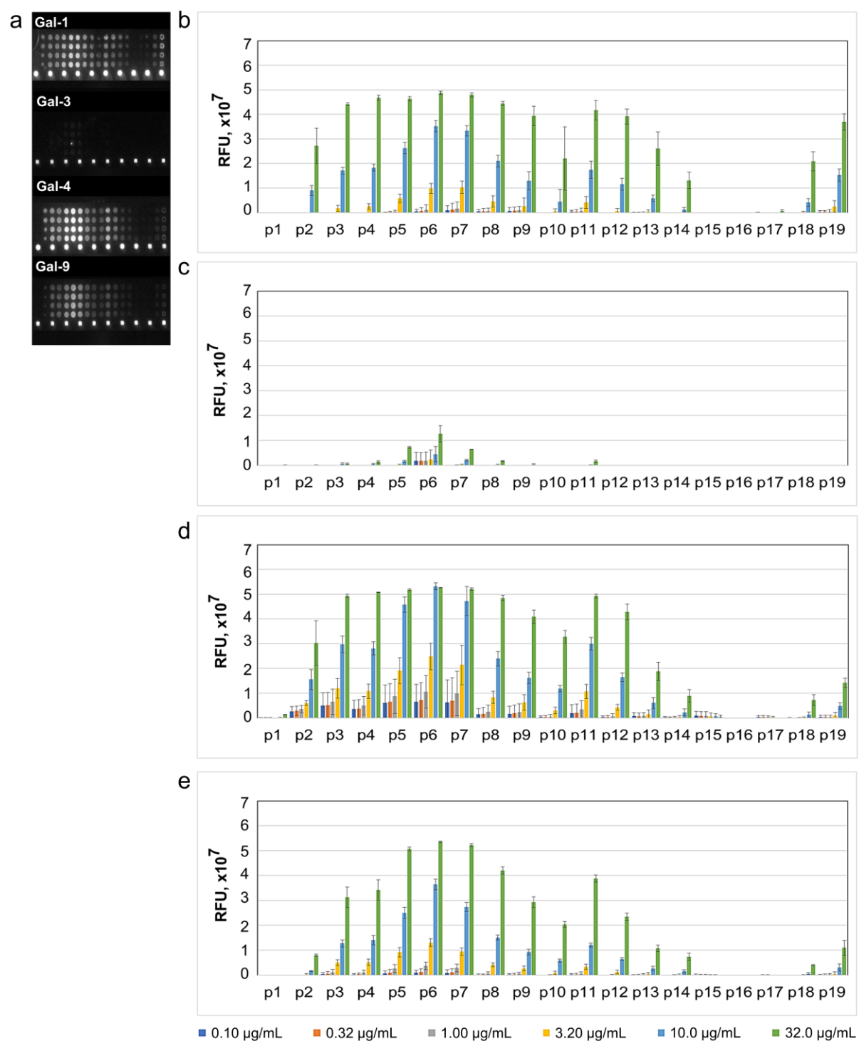
Figure S7. Fluorescence image of microarray chip of \alpha -DG unglycosylated peptide library taken after treatment with 10.0 \mu\text{g/mL} galectin solution ( a ) and relative interaction of 200 \mu\text{M} \alpha -DG unglycosylated peptides with 0.10 \mu\text{g/mL} to 32.0 \mu\text{g/mL} Gal-1 ( b ), Gal-3 ( c ), Gal-4 ( d ), and Gal-9 ( e ).
