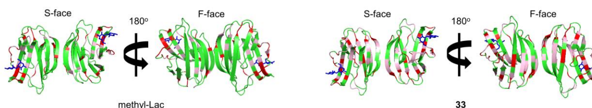
Figure 3. The crystal structure of Gal-1 (PDB access code: 1GZW) is shown with the largest \Delta\delta values highlighted in red ( \Delta\delta \geq 0.05 ) and pink ( 0.025 \leq \Delta\delta < 0.05 ) for methyl-Lac (C) and compound 33 (b) based on HSQC results. For orientation, lactose is presented in all models.
