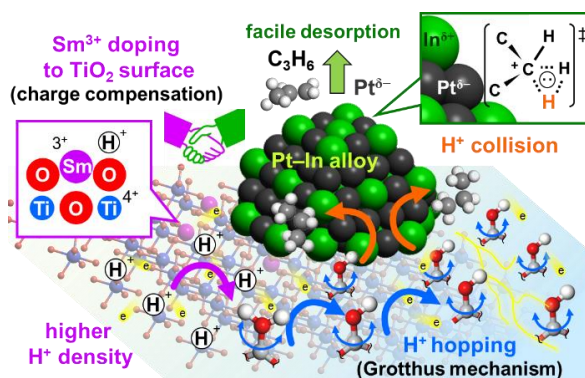
Scheme 1.2. The catalyst design for enhancing electroassisted PDH at low temperatures. \text{Sm}^{3+} is doped into \text{TiO}_2 surface to increase the number of surface protons by charge compensation. Pt–In alloy is used for selective formation of propylene and to enhance the proton collision with propane.
