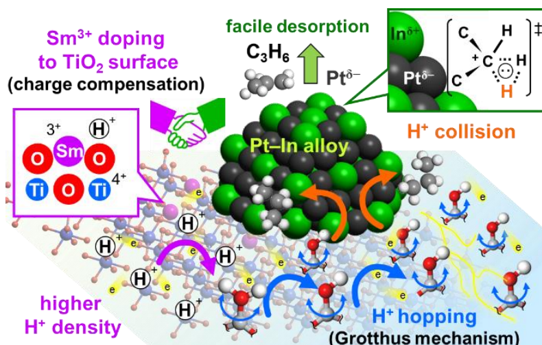
Scheme 3.1. The catalyst design for enhancing electroassisted PDH at low temperatures. Sm 3+ is doped into TiO 2 surface to increase the number of surface protons by charge compensation. Pt–In alloy is used for selective formation of propylene and to enhance the proton collision with propane.
