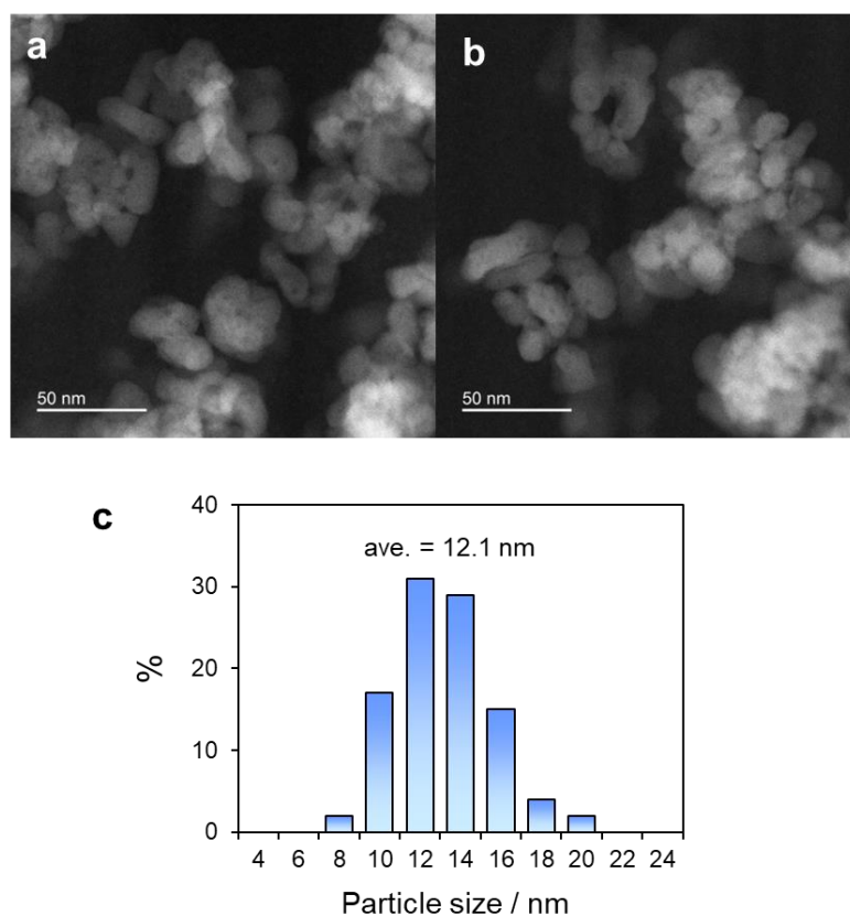
Figure 3.5. (a, b) HAADF-STEM images of Sm-TiO 2 (Sm: 1 mol%) and (c) the corresponding particle size distribution.
