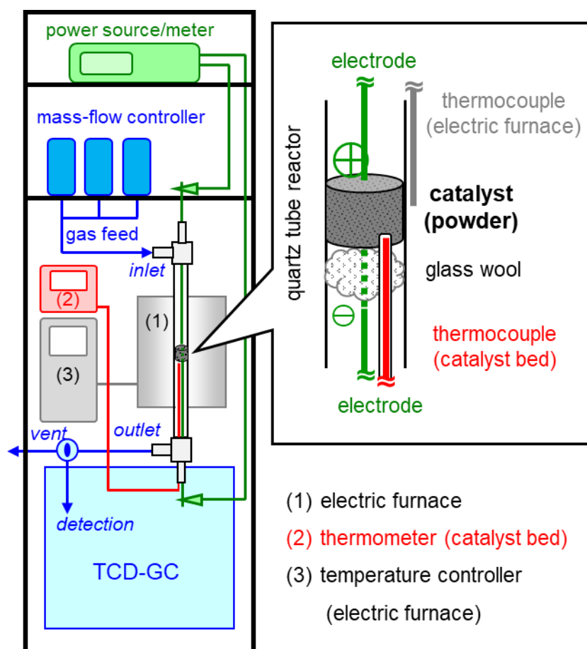
Figure 4.1. The detailed setup of the reactor for electroassisted \text{CO}_2 -OCM. The thermocouple for the catalyst bed was covered with a capillary glass tube for insulation protection.
