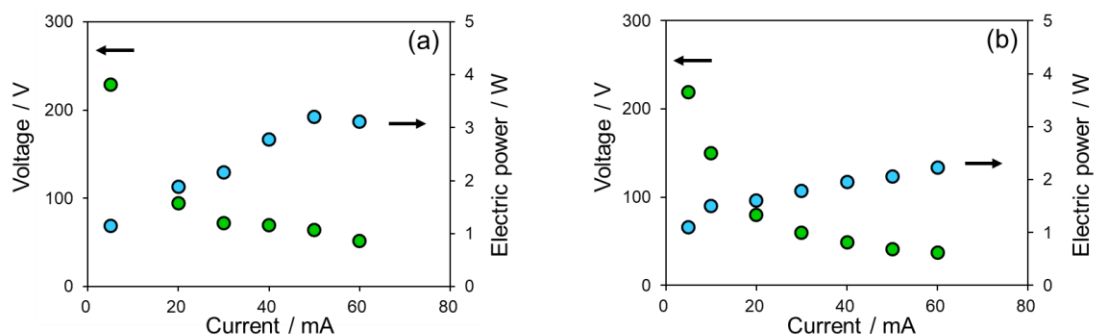
Figure 2.13. The relationship between voltage, current, and electric power for electro-assisted PDH over Pt-In/TiO 2 at (a) 250°C and (b) 300°C.
