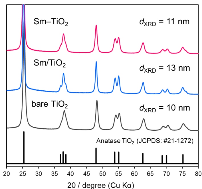
Figure 3.4. XRD patterns of bare \text{TiO}_2 (JRC-TIO-7, anatase) and the corresponding Sm-doped ( \text{Sm}-\text{TiO}_2 ) and -loaded ( \text{Sm/TiO}_2 ) samples. Crystallite sizes ( d_{\text{XRD}} ) estimated using Scherrer's equation are shown.
