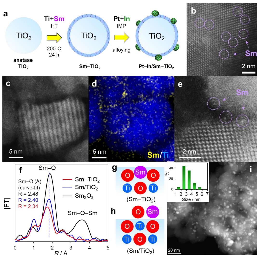
Figure 3.2. (a) Schematic illustration of catalyst preparation: hydrothermal (HT) synthesis of \text{Sm-TiO}_2 and the subsequent impregnation and alloying of \text{Pt-In/Sm-TiO}_2 . (b) HAADF-STEM image and the (c-e) the corresponding cross-sectional analysis of \text{Sm-TiO}_2 ( \text{Sm} : 1 mol%) using FIB etching: (c) HAADF-STEM image, (d) elemental map acquired by EDX, and (e) high-resolution HAADF-STEM image focusing on the surface. (f) Fourier transforms of Sm K-edge EXAFS of Sm-containing samples. Plausible surface structures of (g) Sm-doped and (h) - loaded \text{TiO}_2 with ionic radii. (i) HAADF-STEM image of \text{Pt-In/Sm-TiO}_2 ( \text{Sm} : 1 mol%). Inset shows the particle size distribution.
