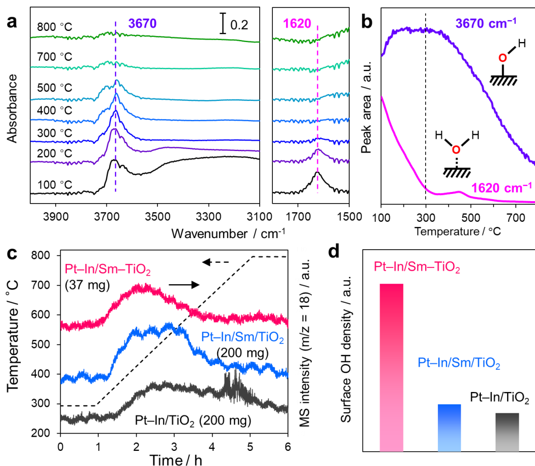
Figure 3.12. Estimation of surface hydroxyl groups by IR-MS-TPD analysis. (a) FT-IR spectra of Pt-In/Sm-TiO 2 upon heating under vacuum. (b) Temperature dependence of the peak area of those at 3670 cm -1 and 1620 cm -1 . (c) The MS-TPD spectra for the dehydration condensation of surface hydroxyl groups. Values in parentheses indicate the amount of catalyst used for the analysis. (d) The density of surface hydroxyl groups.
