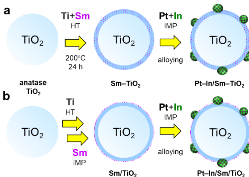
Figure 3.3. Schematic illustration of catalyst preparation: (a) hydrothermal (HT) synthesis for \text{Sm}-\text{TiO}_2 and the subsequent impregnation (IMP) and alloying for \text{Pt-In/Sm-TiO}_2 . (b) HT synthesis of Sm-free Ti layer on core anatase \text{TiO}_2 and the subsequent Sm-IMP for \text{Sm/TiO}_2 , followed by \text{Pt+In} IMP and alloying for \text{Pt-In/Sm/TiO}_2 .
