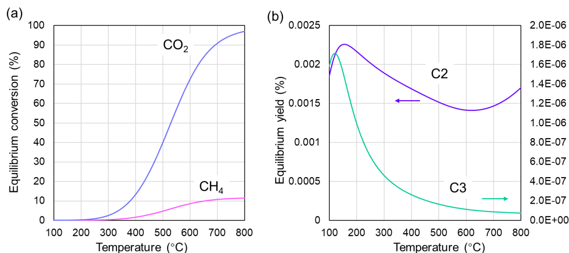
Figure 4.2. Temperature dependence of the (a) equilibrium conversions (CH 4 and CO 2 ) and (b) yields of product hydrocarbons (C 2 and C 3 hydrocarbons) in thermal CO 2 -OCM (CH 4 : CO 2 : He = 2.8:1:7.4). Calculation was done using HSC Chemistry 8 software.
