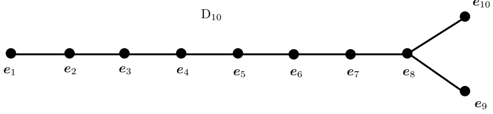
Figure 4: Dynkin diagram of type D_{10} .
