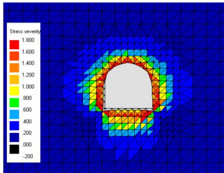
(e) Modified stress severity before mining
