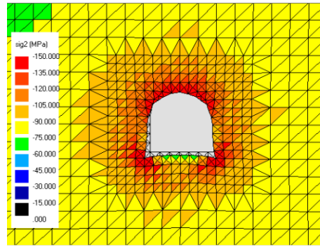
(b) Just before rockburst
