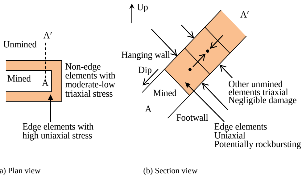
Fig. 4.6 Concept of edge element.
