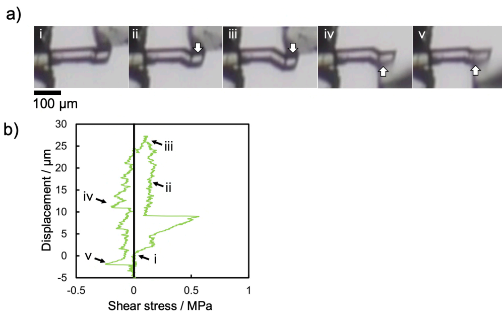
Figure S11. (a) Snapshots of ferroelastic twinning deformation of 3i ( 574 \times 49 \times 50\text{ }\mu\text{m}^3 ) upon application of shear stress under visible (VIS) light at -1\text{ }^{\circ}\text{C} ( -5\sim 2\text{ }^{\circ}\text{C} ): ii–iii) forward direction and iv–v) reverse direction. (b) Stress-displacement cycles of the crystal under VIS light.
