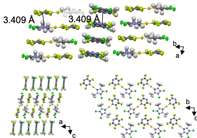
Figure S9. Comparison of the single-crystal structures of 3i at 20 °C and −20 °C.
