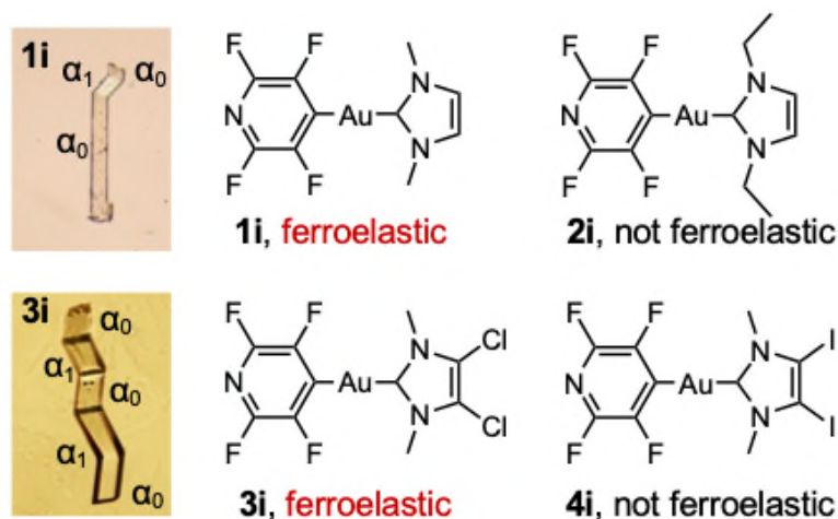
Figure 1. Chemical structures of 1i–4i and photographs of bent crystals of 1i and 3i .
