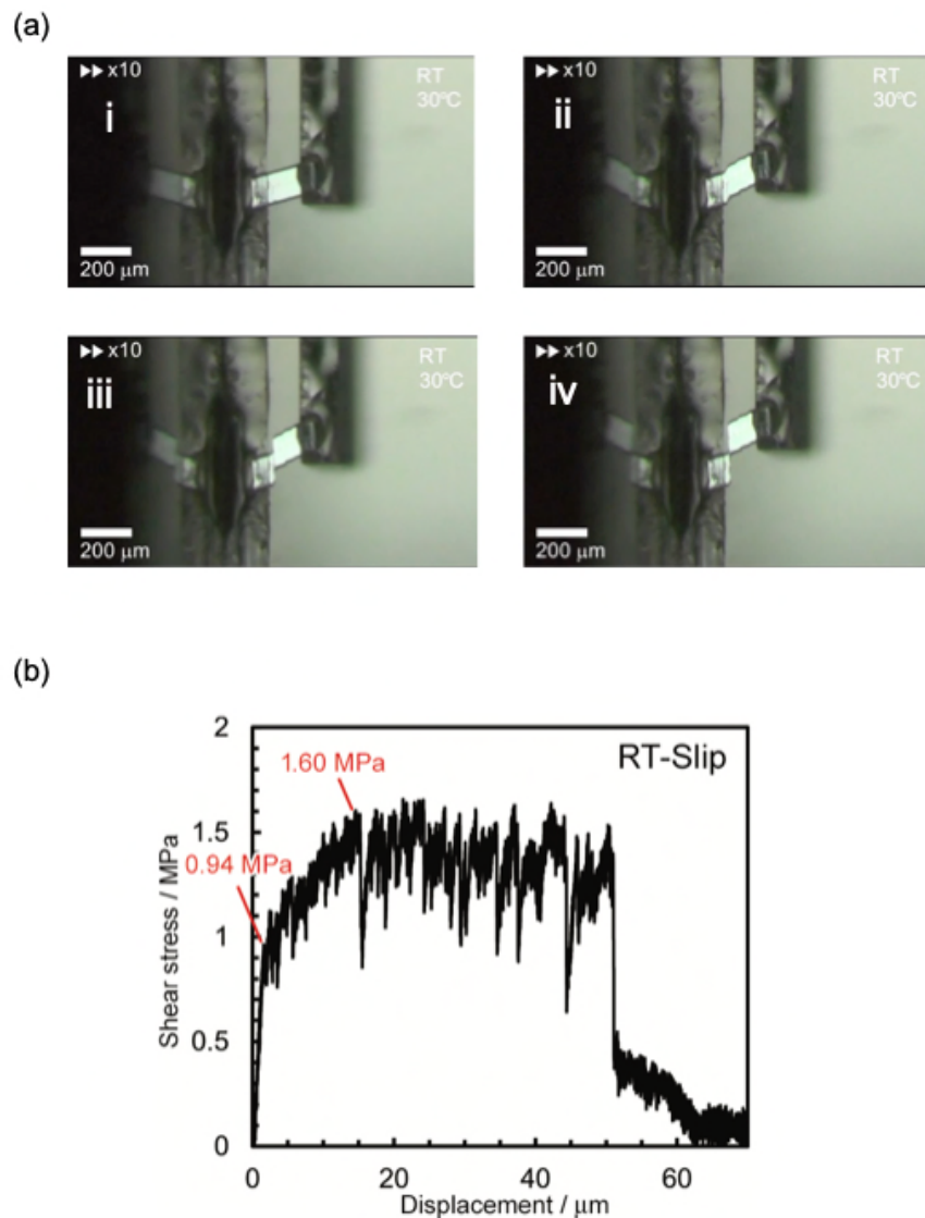
Figure S16. (a) Snapshots of slip deformation of RT upon application of shear stress under visible light at 30 °C. (b) Stress-displacement result of the crystal under VIS light.
