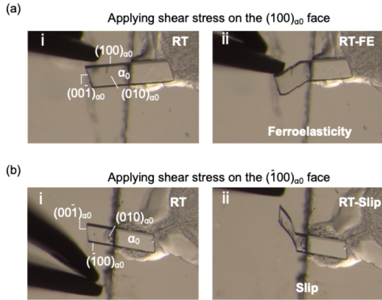
Figure S15. Photographic images of deformed RT . The mechanical properties of the RT crystal were investigated by applying shear stress at the (100)_{\alpha 0} face and (\bar{1}00)_{\alpha 0} face, which showed (a) ferroelastic and (b) slip deformation, respectively.
