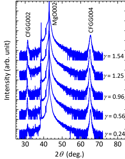
Fig. S2. XRD \theta - 2\theta scan for \text{Co}_2\text{Fe}_{1.03}\text{Ga}_{0.45}\text{Ge}_\gamma ( \gamma = 0.24, 0.56, 0.96, 1.25 , and 1.54 ) thin films.
