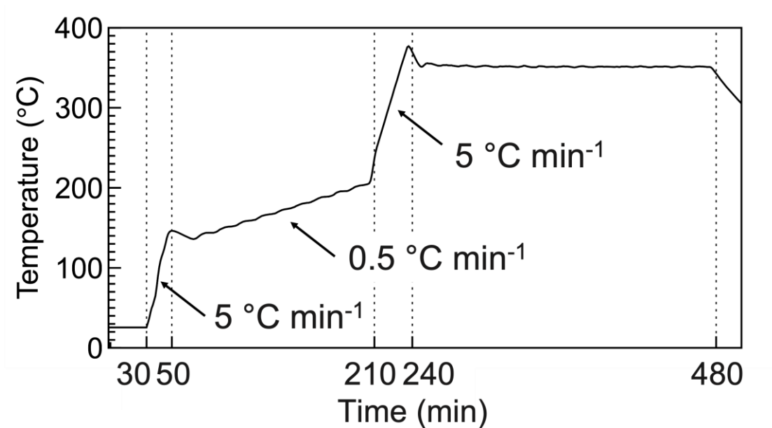
Figure S1. Temperature profile for the synthesis of CoNi/rGO catalysts.
