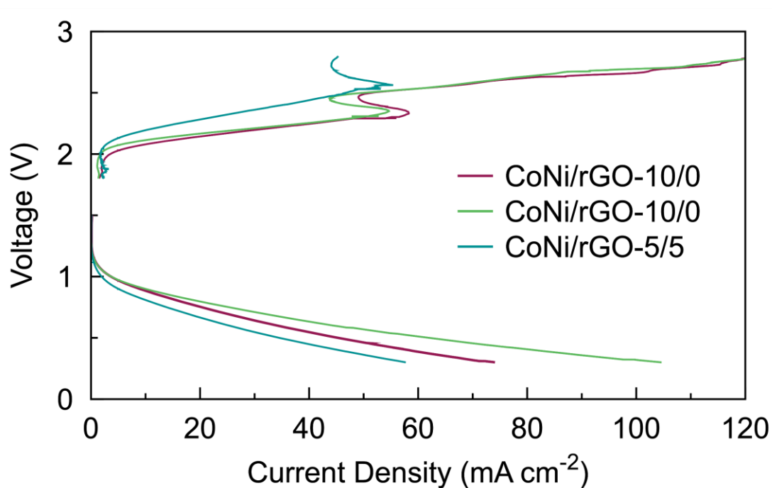
Figure S12. Charge and discharge polarization curves for ZAB using CoNi/rGO-10/0, 5/5, and 0/10 catalysts.
