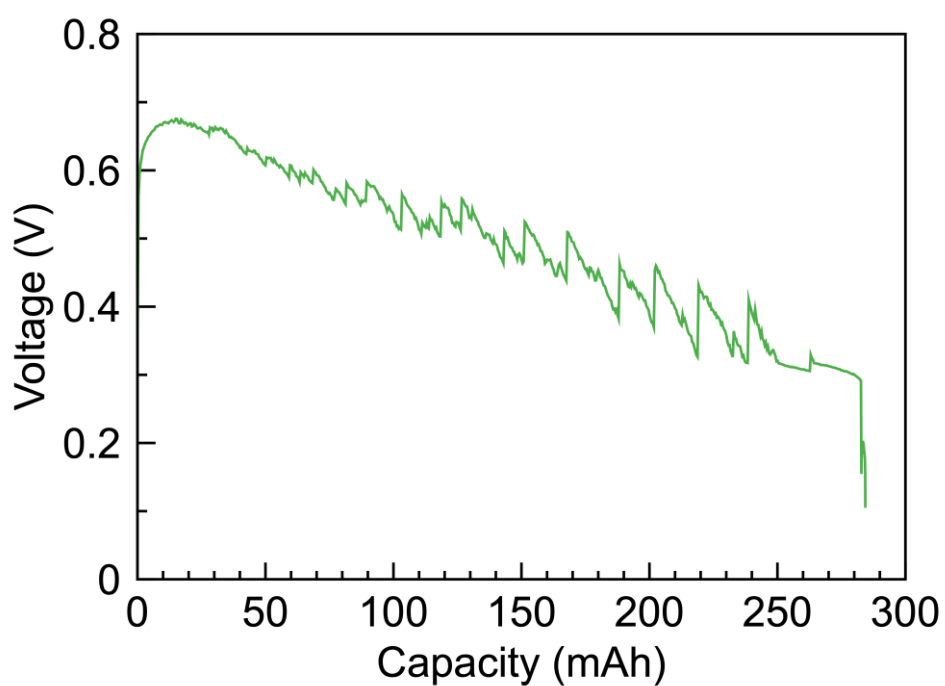
Figure S11. Discharge profile of ZAB with CoNi/rGO-5/5 catalyst for the air electrode at 100 \text{ mA} \cdot \text{cm}^{-2} . The discharge voltage (vs. Zn anode) was more than 0.6 V during the first 1 h discharge.
