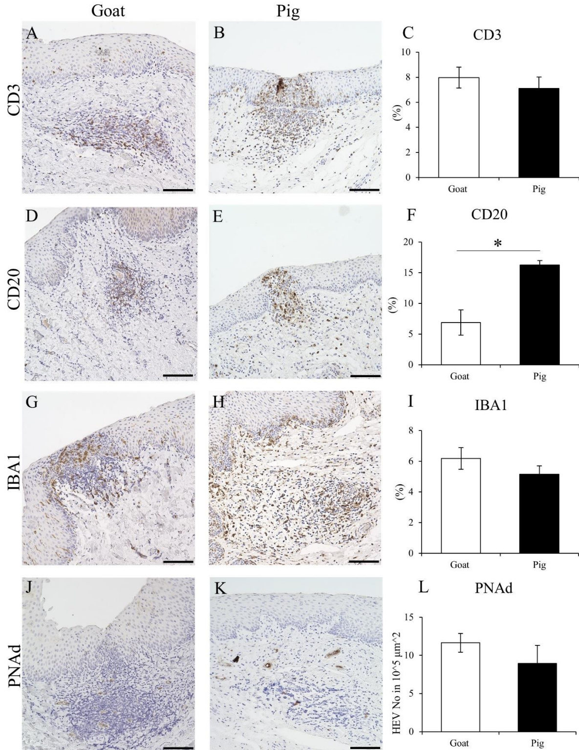
Figure 2-4. Immune cell characteristics composing LN in goat and pig vaginal vestibule
