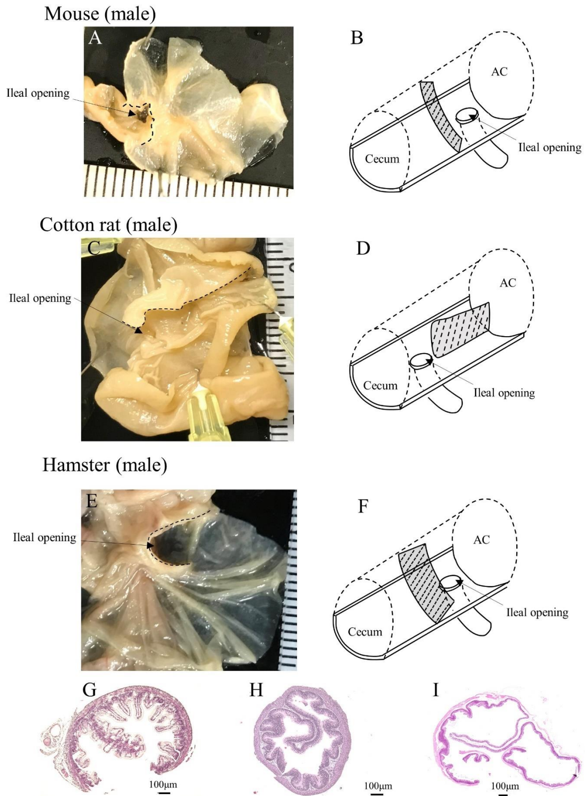
Figure 3-8. Morphological comparison of mucosal fold in the ascending colon of several rodents and SLMF appearance at different aged cotton rats.
