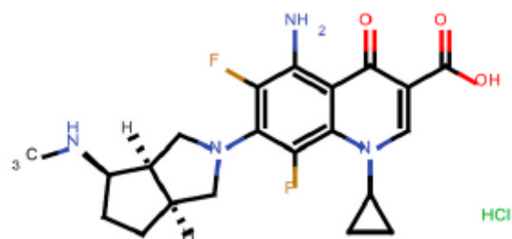
Figure 1. Chemical structure of compounds
