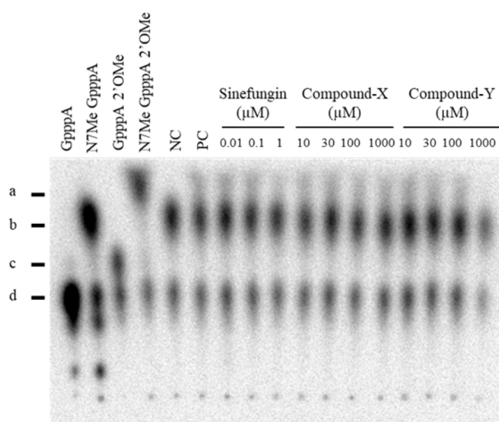
Figure 6. DENV2 MTase activity inhibitory assay using Compound-X and Compound-Y
