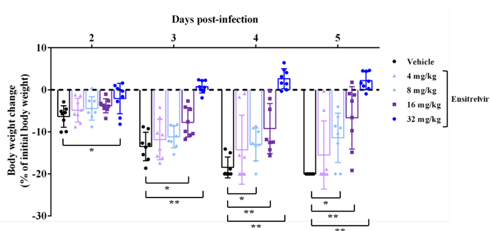
Figure 10. Effect of ensitrelvir on survival and the body weight of 40-week-old female BALB/cAJcl mice infected with mouse-adapted SARS-CoV-2 MA-P10
