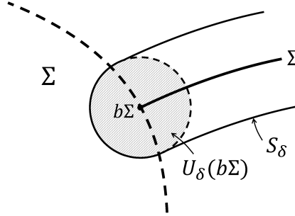
Figure 12: near the boundary of \Sigma
