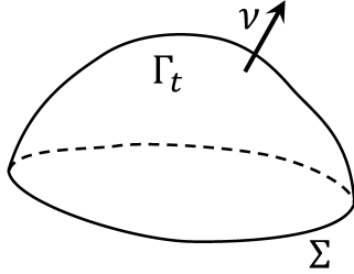
Figure 1: prescribed boundary \Sigma
