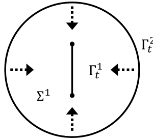
Figure 8: \Gamma_t^2 hits \Sigma^1
