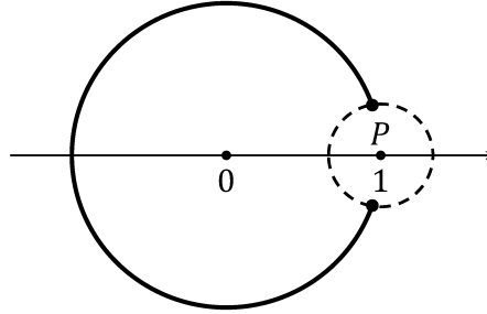
Figure 14: figure of \Gamma_0^m
