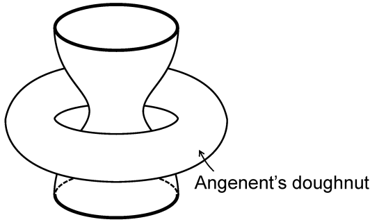
Figure 6: example of pinching
