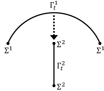
Figure 7: \Gamma_t^1 hits the upper part of \Sigma^2 in finite time.
