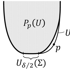
Figure 10: a pushed domain
