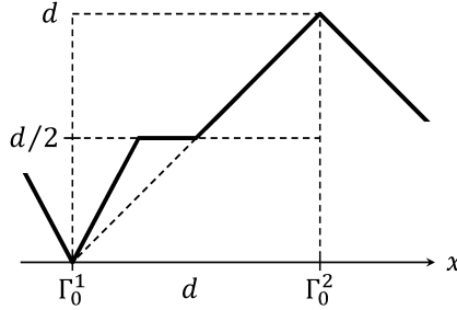
Figure 5: graph of u_0
