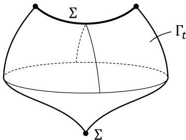
Figure 4: example of \Sigma
