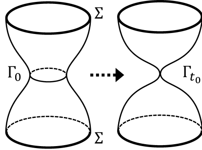
Figure 2: pinching at time t_0
