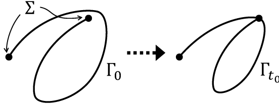
Figure 3: hitting \Sigma at time t_0
