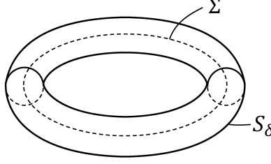
Figure 11: \Sigma and S_\delta
