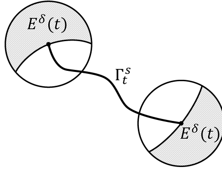
Figure 13: sets E^\delta(t) and \Gamma_t^s
