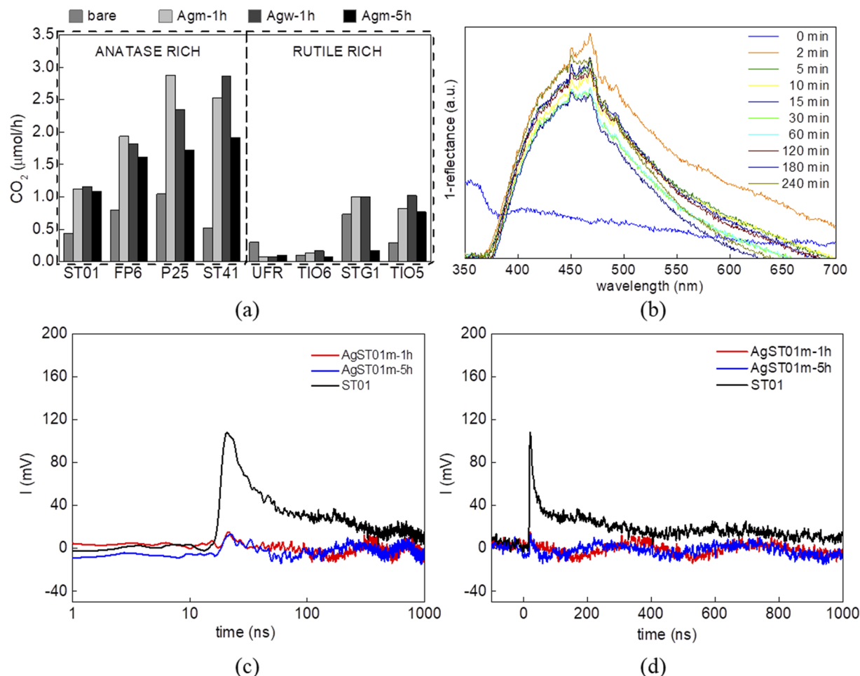
FIG. 7. (a) Photocatalytic activity of pristine and silver-modified samples under UV/vis irradiation ( \lambda > 300 \text{ nm} ), (b) DRS of AgST41w-1h suspended in aqueous solution of acetic acid before and after irradiation under UV light, and (c) and (d) TRMC data for pristine and silver-modified ST01 samples.
