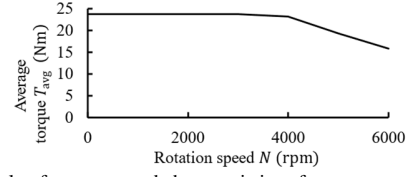
Fig. 4. Example of torque-speed characteristics of motors.
