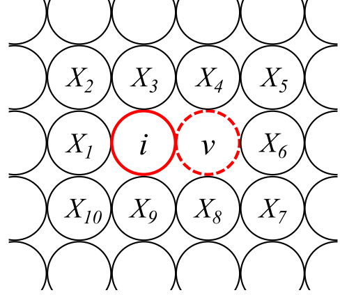
FIG. 1. Schematic depicting an i - v pair cluster, where the first and second nearest-neighboring atoms are numbered from 1 to 10 [16].
