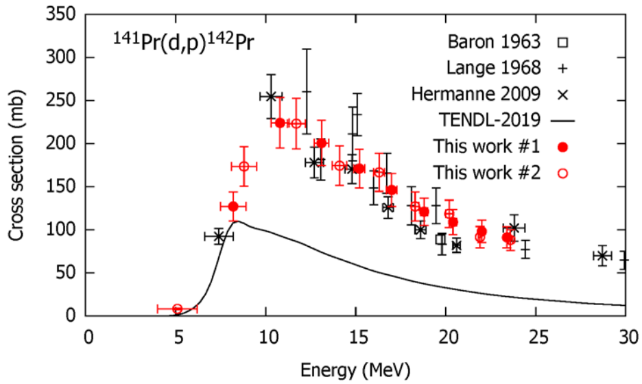
Fig. 4. Cross sections of the ^{141}\text{Pr}(\text{d},\text{p})^{142}\text{Pr} reaction in comparison with the previous data [3,5,6] and the TENDL-2019 values [14].
