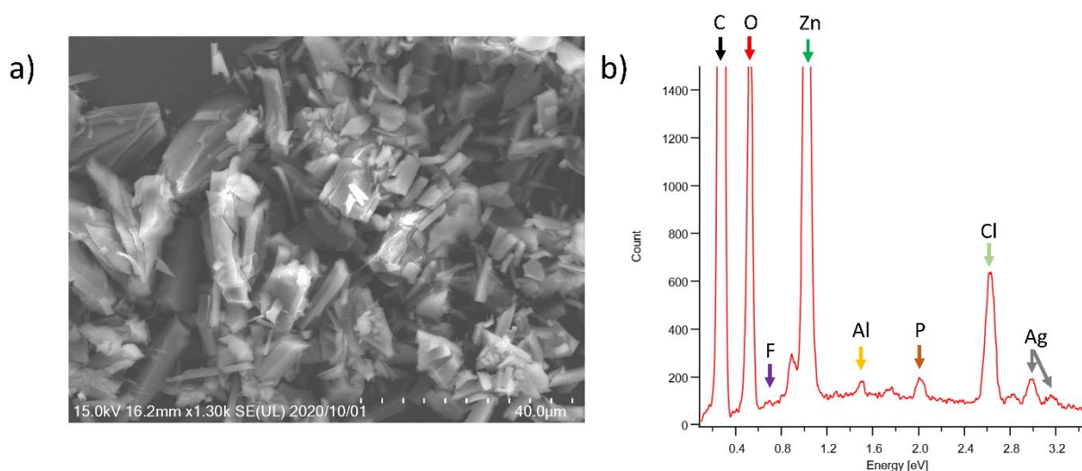
Fig. 1 a) SEM image of \text{Li}@\text{C}_{60}/\text{MOF-177} . b) EDX spectrum obtained. Only the small amounts of \text{PF}_6 are detected. Al is due to the sample holder, Ag is due to metal sputtering.
