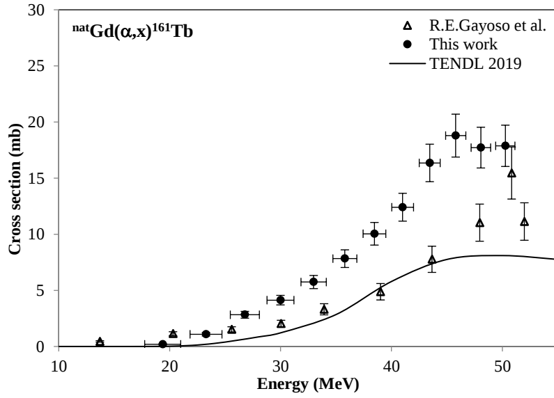
Fig. 9. Excitation function of the ^{nat}\text{Gd}(\alpha,x)^{161}\text{Tb} reaction
