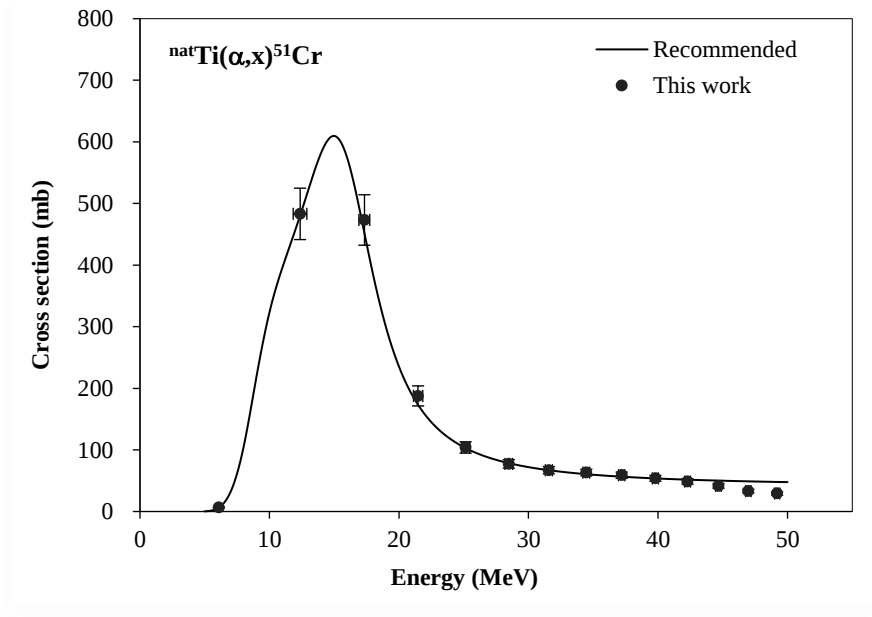
Fig. 1. Excitation function of the ^{nat}\text{Ti}(\alpha, x)^{51}\text{Cr} monitor reaction with the recommended values [18].
