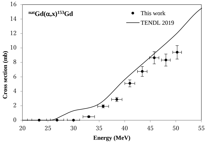
Fig. 10. Excitation function of the ^{nat}\text{Gd}(\alpha,x)^{153}\text{Gd} reaction
