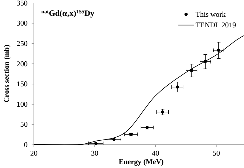
Fig. 2. Excitation function of the ^{nat}\text{Gd}(\alpha,x)^{155}\text{Dy} reaction
