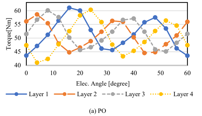
Fig. 5. Torque waveforms of reference and optimized motors
