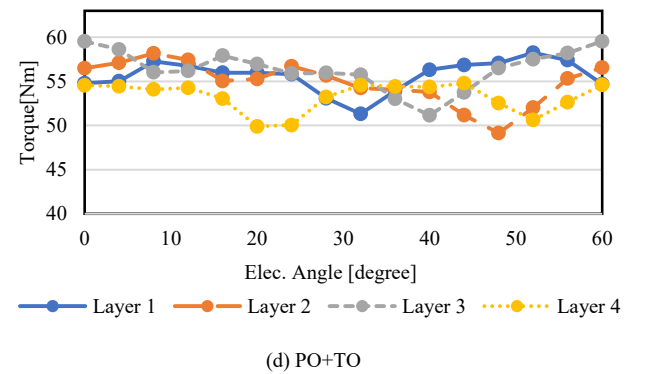
Fig. 6. Torque waveform of each layer
