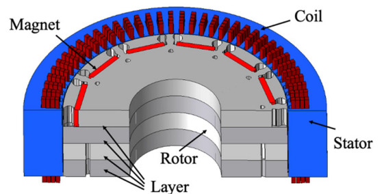
Fig. 1 Structure of the step-skewed PMSM
