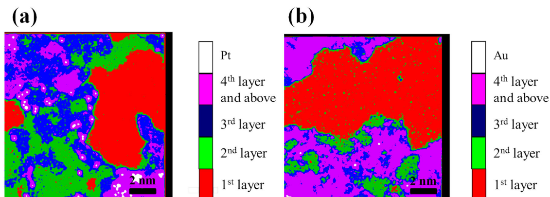
Figure 6. Pseudo-colored images of (a) Pt and (b) Au dispersed on graphene. Because the structure of the upper layers was complicated and the number of layers could not be distinguished, we classified the (1 st ) single graphene sheet and the number of nanographene layers into 2 nd , 3 rd and more than 4 layers of nanographene.
