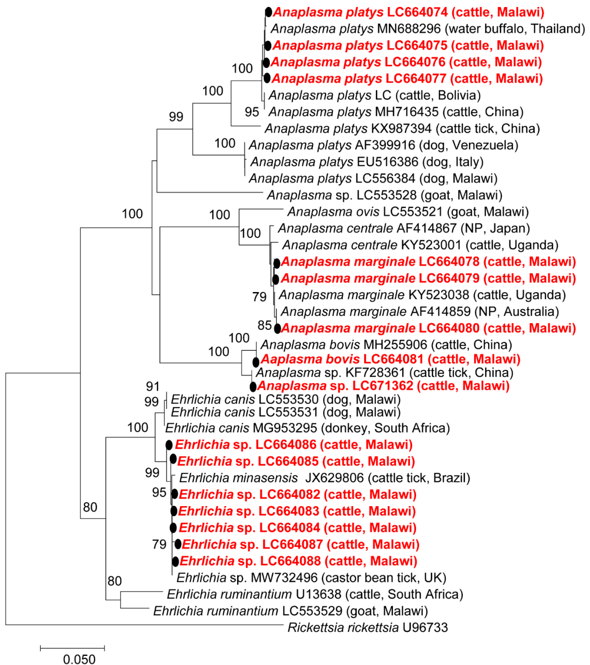
Figure 5. The maximum likelihood phylogenetic tree of the Anaplasma and Ehrlichia species detected in cattle in Malawi. The analysis was based on partial sequences of groEL gene which was constructed using the Tamura 2 parameter model. Rickettsia rickettsii was used as outgroup. All bootstrap values > 75% from 1000 replications are shown on the interior branch nodes and the sequences obtained in this study are indicated in bold. The host and country of origin are indicated in parenthesis, NP means not provided. The bar 0.050 is the genetic distance of each sequence from the root of the tree.
