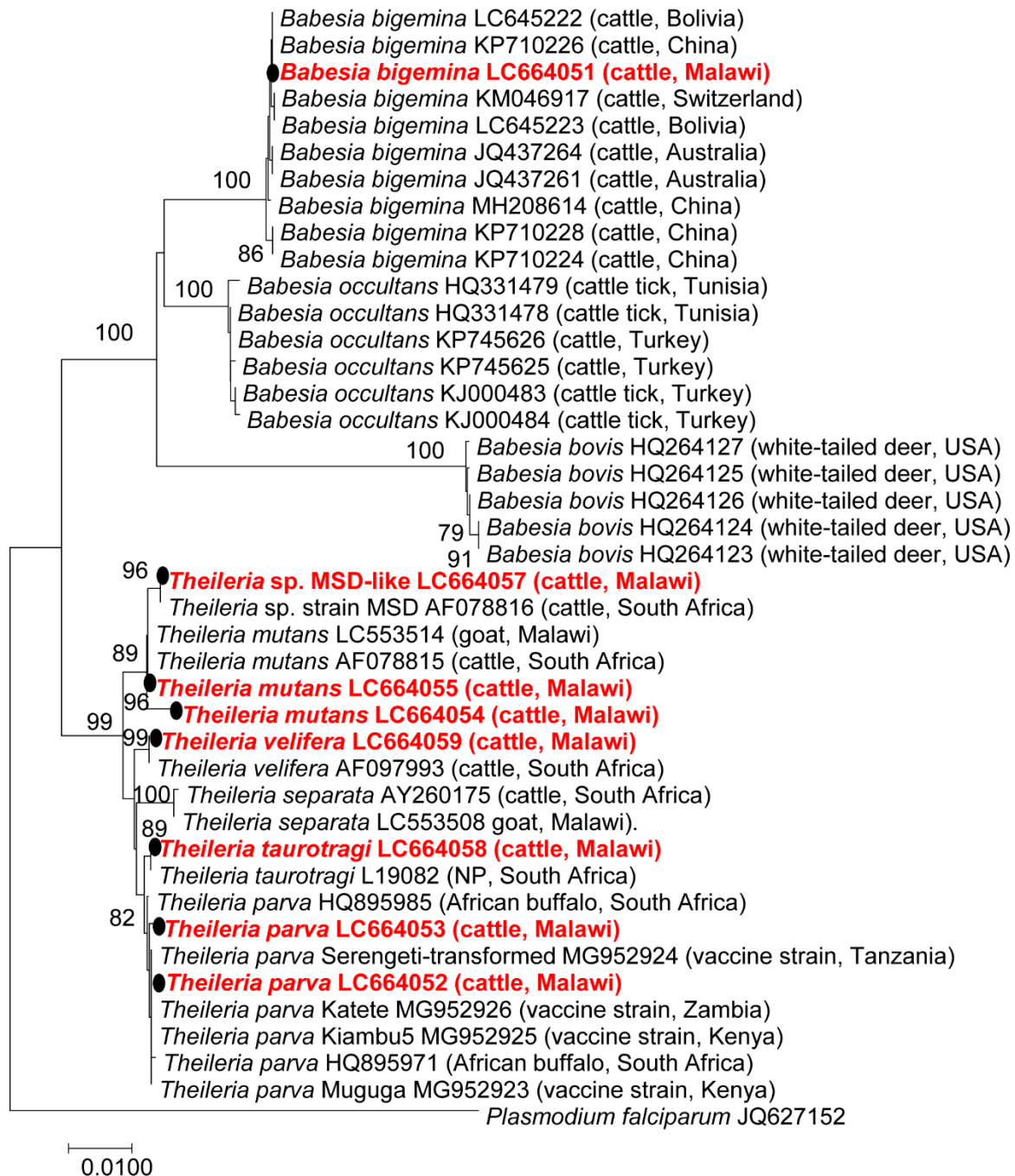
Figure 3. The maximum likelihood phylogenetic tree of the Babesia and Theileria species detected in cattle in Malawi. The analysis was based on partial sequences of 18S rDNA which was constructed using the Kimura 2 parameter model. Plasmodium falciparum was used as outgroup. All bootstrap values > 75% from 1000 replications are shown on the interior branch nodes and the sequences obtained in this study are indicated in red. The host and country of origin are indicated in parenthesis, NP means not provided. The bar 0.10 is the genetic distance of each sequence from the root of the tree.
