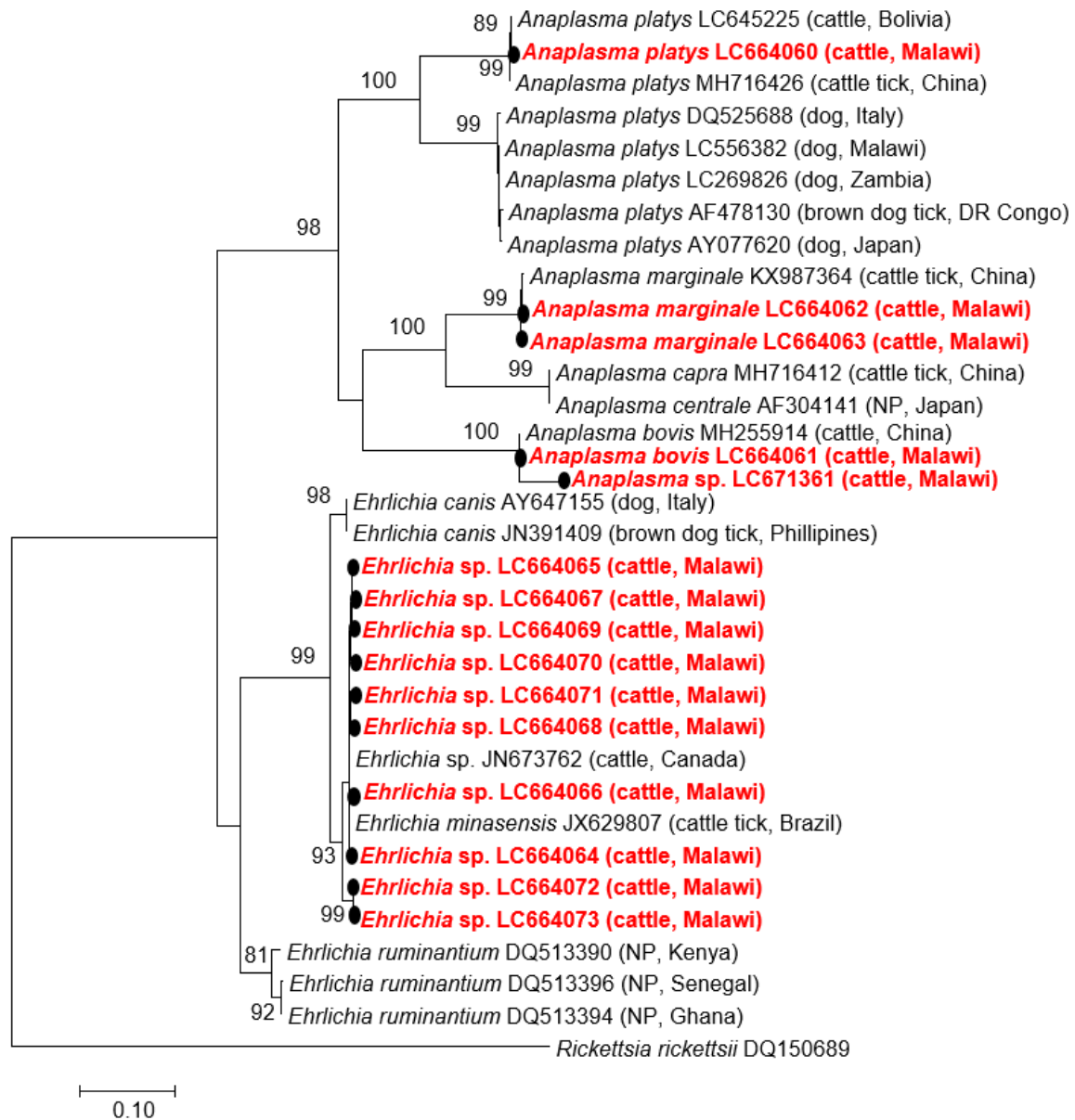
Figure 4. The maximum likelihood phylogenetic tree of Anaplasma and Ehrlichia species detected in cattle in Malawi. The analysis was based on partial sequences of gltA gene which was constructed using the Tamura 2 parameter model. Rickettsia rickettsii was used as outgroup. All bootstrap values > 75% from 1000 replications are shown on the interior branch nodes and the sequences obtained in this study are indicated in red. The host and country of origin are indicated in parenthesis, NP means not provided. The bar 0.10 is the genetic distance of each sequence from the root of the tree.
