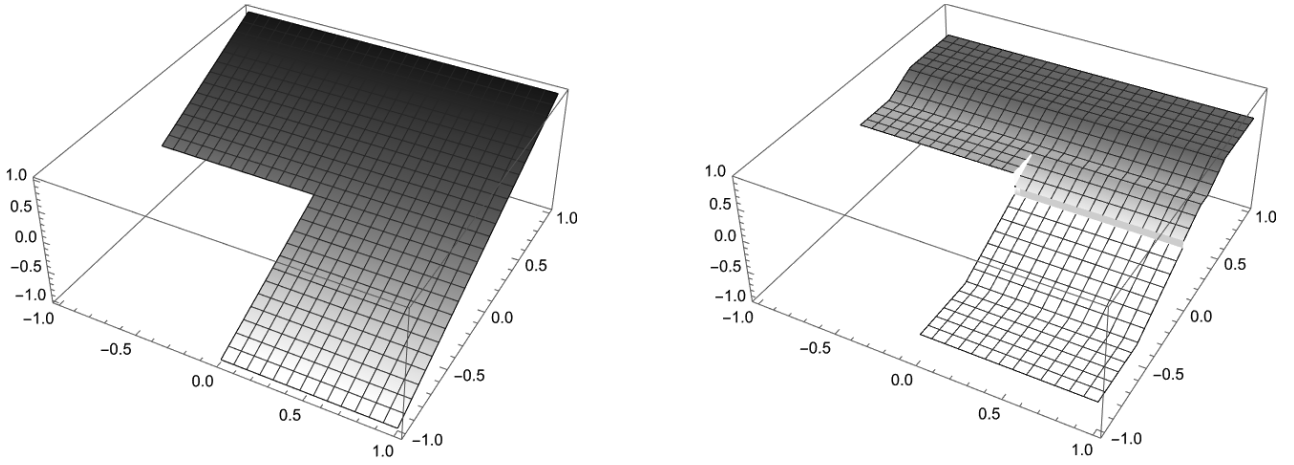
Figure 3: Example f and u in the case d = 2 , \mathcal{R} = \lambda TV_1 with a suitable choice of \lambda .
