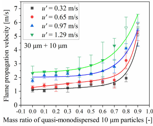
(a) Flame propagation velocity versus the mass ratio of 10-μm quasi-monodispersed particles
