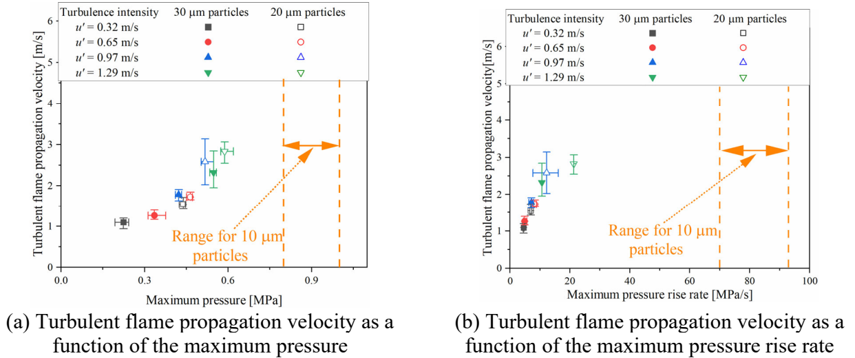
Fig. 13 Turbulent flame propagation velocity as a function of pressure characteristics for the combustion of quasi-monodispersed particles under different particle sizes.
