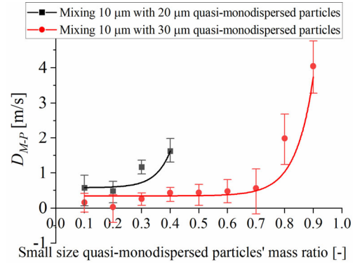
(b) D_{M-P} as a function of the mass ratio of 10- \mu m quasi-monodispersed particles
