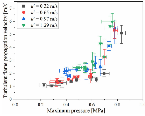
(a) Turbulent flame propagation velocity as a function of the maximum pressure
