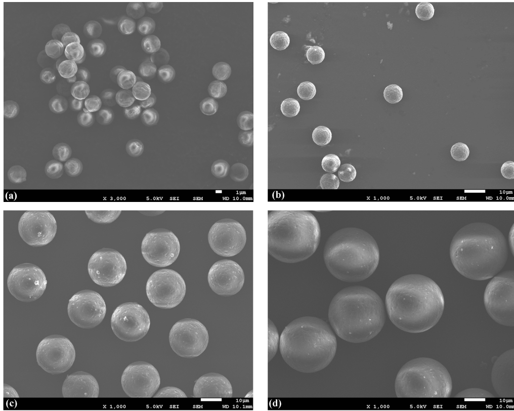
Fig. 2 Scanning electron microscopy (SEM) micrographs of the quasi-monodispersed particles: (a) 3- \mu\text{m} particles, (b) 10- \mu\text{m} particles, (c) 20- \mu\text{m} particles, and (d) 30- \mu\text{m} particles.
