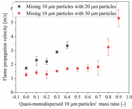
(a) Flame propagation velocity as a function of the mass ratio of 10- \mu m quasi-monodispersed particles
