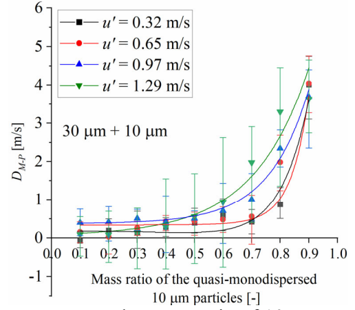
(b) D_{M-P} versus the mass ratio of 10-μm quasi-monodispersed particles
