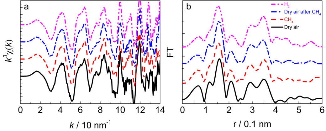
Figure 4. EXAFS for SnO 2 at 703 K. a: Sn K-edge k^3 -weighted EXAFS oscillations ( k^3\chi(k) ) and b: their Fourier transforms in dry air, CH 4 , dry air after CH 4 and H 2 .
