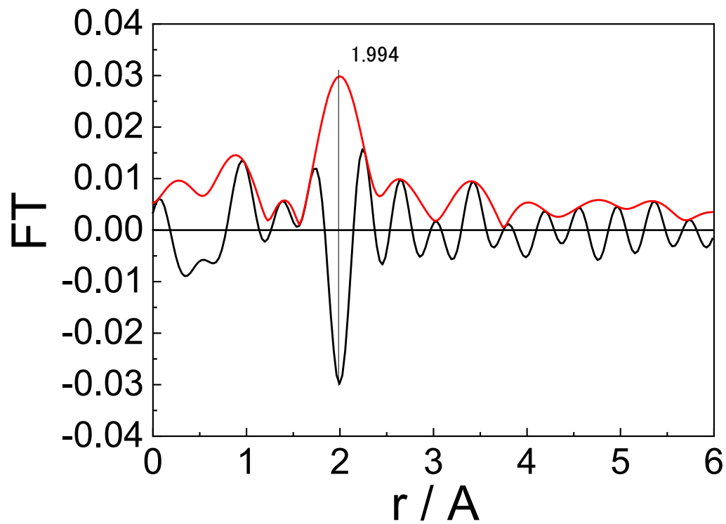
Figure 8. Imaginary (black) and absolute (red) parts of phase-corrected Fourier transform of difference spectrum of Pt–SnO 2 over the k range 2 – 9 \text{\AA} .
