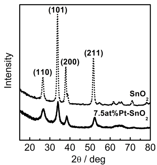
Figure 1. XRD spectra of \text{SnO}_2 and 7.5 at% Pt- \text{SnO}_2 .
