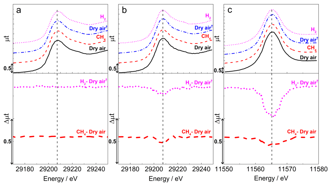
Figure 9. XANES of \text{SnO}_2 and 7.5 at% Pt- \text{SnO}_2 at 703 K. a: Sn K-edge of \text{SnO}_2 , b: Sn K-edge, and c: Pt L_3 -edge of Pt- \text{SnO}_2 . \text{Dry air}^\dagger is air after \text{CH}_4 flow.
