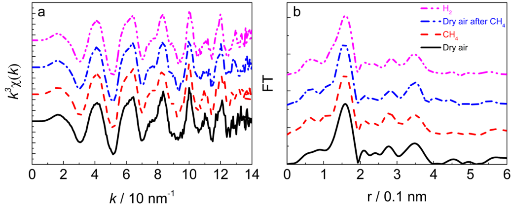
Figure 5. EXAFS for 7.5 at% Pt-SnO 2 at 703 K. a: Sn K-edge k^3 -weighted EXAFS oscillations ( k^3\chi(k) ) and b: their Fourier transforms in dry air, CH 4 , dry air after CH 4 and H 2 .
