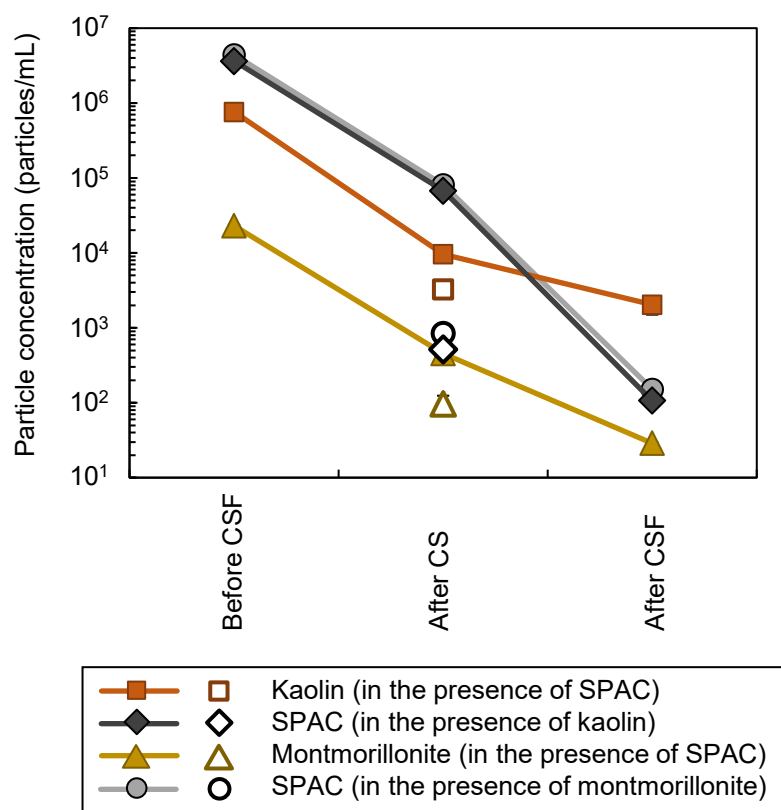
Fig. 3. Behaviors of kaolin, montmorillonite, and SPAC during the CSF process. Either kaolin or montmorillonite and SPAC were added simultaneously. The open symbols indicate the data measured after centrifugation. Data from Runs 3, 4, 5, and 6. Details of the experimental conditions are presented in Table S2. Error bars indicate standard deviations of experiments, but some of them are hidden behind the symbols.
