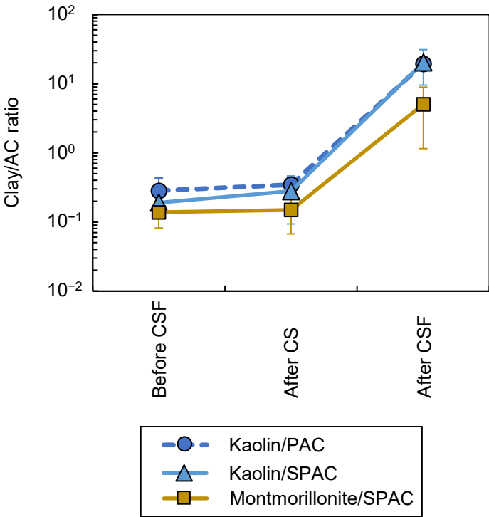
Fig. 4. Ratio of clay particles to activated carbon particles quantified by surface-area concentrations. Either kaolin or montmorillonite and either PAC or SPAC were added simultaneously. Data from Runs 1, 2, 3, 4, 5, 6, 7, 8, 9 10, 11, 12 and 13. Details of the experimental condition are presented in Table S2. Error bars indicate standard deviations of experiments, but some of them are hidden behind the symbols.
