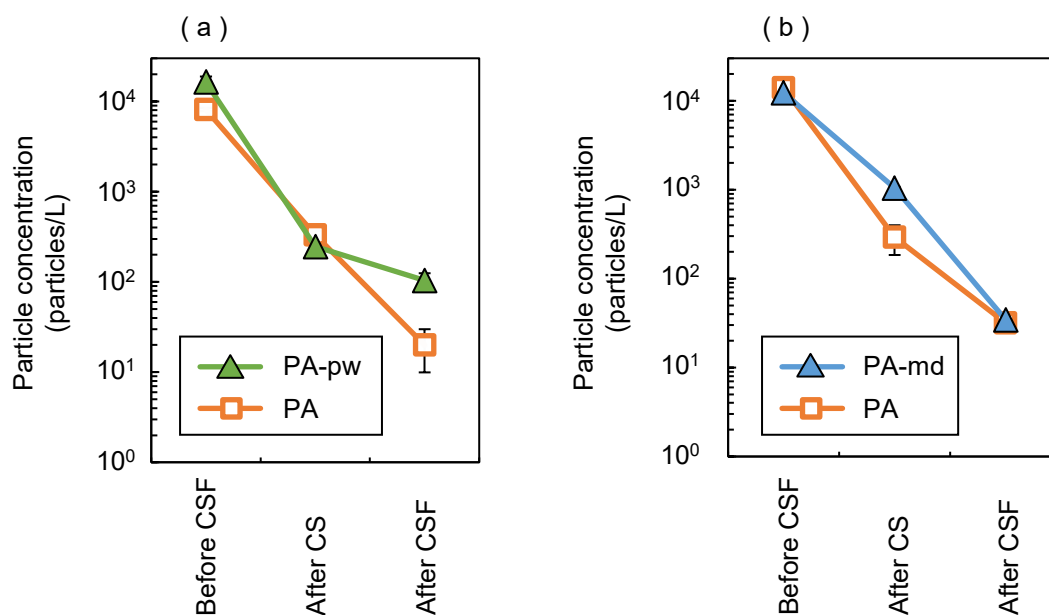
Fig. 7. Effect of photochemical/mechanical weathering on the removal of MP particles during CSF process. Panel a: PA and PA-pw were each added in the presence of kaolin and SPAC simultaneously (Run 3, 4, 9, and 10). Panel b: PA or PA-md was each added in the presence of SPAC simultaneously (Run 14, 15, 16, and 17). Details of the experimental conditions are presented in Table S2. Error bars indicate standard deviations of experiments, but some of them are hidden behind the symbols.
