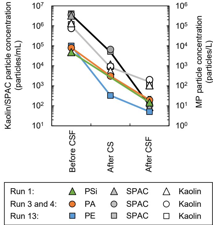
Fig. 5. Behavior of PE, PA, and PSi during the CSF process. PA, Psi, and PE were each treated by CSF in the presence of SPAC and kaolin. Data from Runs 1, 3, 4, and 13. Details of the experimental condition are presented in Table S2. Error bars indicate standard deviations of experiments, but some of them are hidden behind the symbols.
