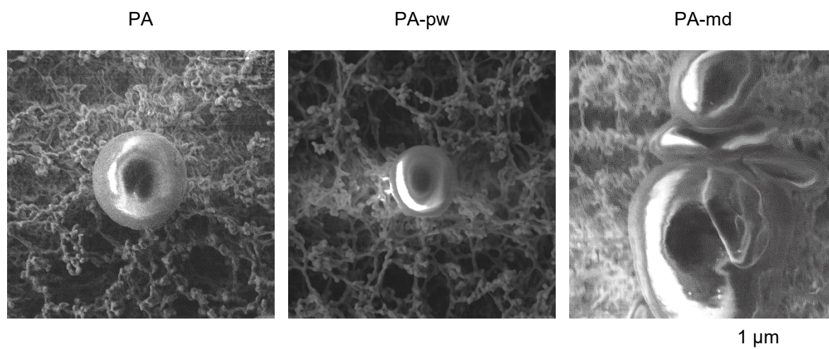
Fig. 8. Field-emission scanning electron microscope images of PA particles before and after weathering.
