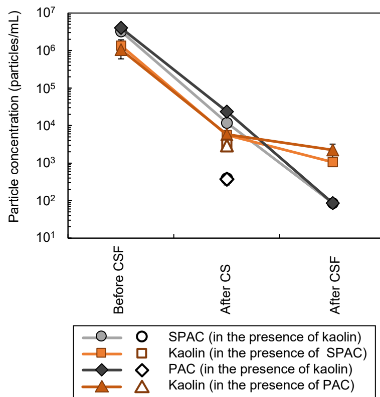
Fig. 2. Behaviors of PAC, SPAC, and kaolin during the CSF process. Kaolin and either PAC or SPAC were added simultaneously. The open symbols indicate the data measured after centrifugation. Data from Run 1 and Run 2. Details of the experimental condition are presented in Table S2. Error bars indicate standard deviations of measurements, but some of them are hidden behind the symbols.
