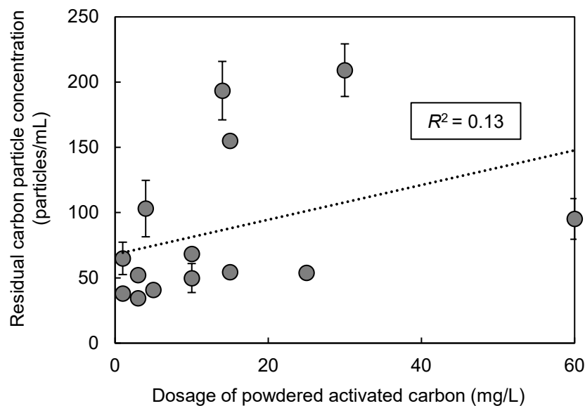
Fig. 1. Residual carbon particle concentration in sand filtrate vs. the dosage of powdered activated carbon. The sample waters were obtained from the 14 full-scale water purification plants employing the CSF process when powdered activated carbon was being injected for adsorption. The dotted line indicates the regression line. Error bars indicate standard deviations
