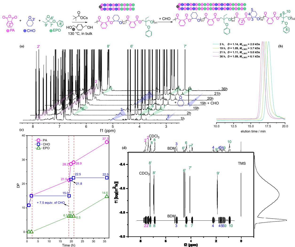
Figure 3. The polymerization from a mixture of PA/CHO/EPO monitored by NMR spectrum and SEC (entry 2 in Table 2): (a) The 1 H NMR (CDCl 3 ) spectrum of crude aliquots withdrawn from the reaction system for monitoring the conversion of PA, CHO, EPO, and the formation of resultant polymers. (b) Evolution of SEC traces (THF). (c) Plots of the degree of polymerization (DP) versus time. (d) DOSY (CDCl 3 ) spectrum of resultant polymers.
