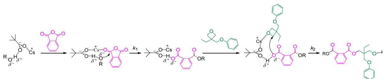
Scheme 2. Proposed mechanism of ROCOP from a mixture of PA and EPO with cesium pivalate as the catalyst and alcohol as the initiator.
