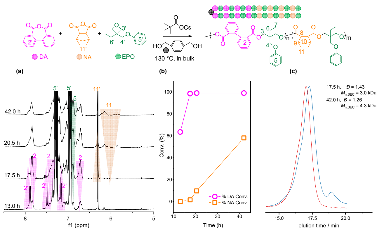
Figure 4. The polymerization from a mixture of DA/NA/EPO monitored by NMR spectrum and SEC (entry 4 in Table 2): (a) The 1 H NMR (CDCl 3 ) spectrum of crude aliquots withdrawn from the reaction system for monitoring the conversion of DA, NA, EPO, and the formation of resultant polymers. (b) Plots of monomers conversion versus time. (c) Evolution of SEC traces (THF).
