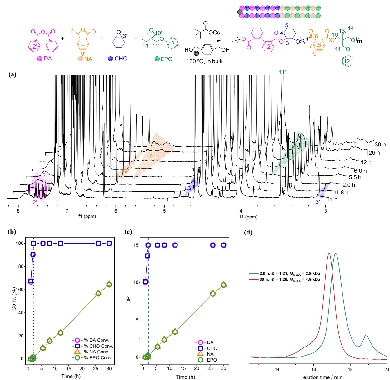
Figure 5. The polymerization from a mixture of DA/CHO/NA/EPO monitored by NMR spectrum and SEC (entry 6 in Table 2): (a) The ^1\text{H} NMR ( \text{CDCl}_3 ) spectrum of crude aliquots withdrawn from the reaction system for monitoring the conversion of DA, CHO, NA, EPO, and the formation of resultant polymers. (b) Plots of monomers conversion versus time and conversion of EPO are normalized. (c) Plots of the degree of polymerization versus time. (d) Evolution of SEC traces (THF).
