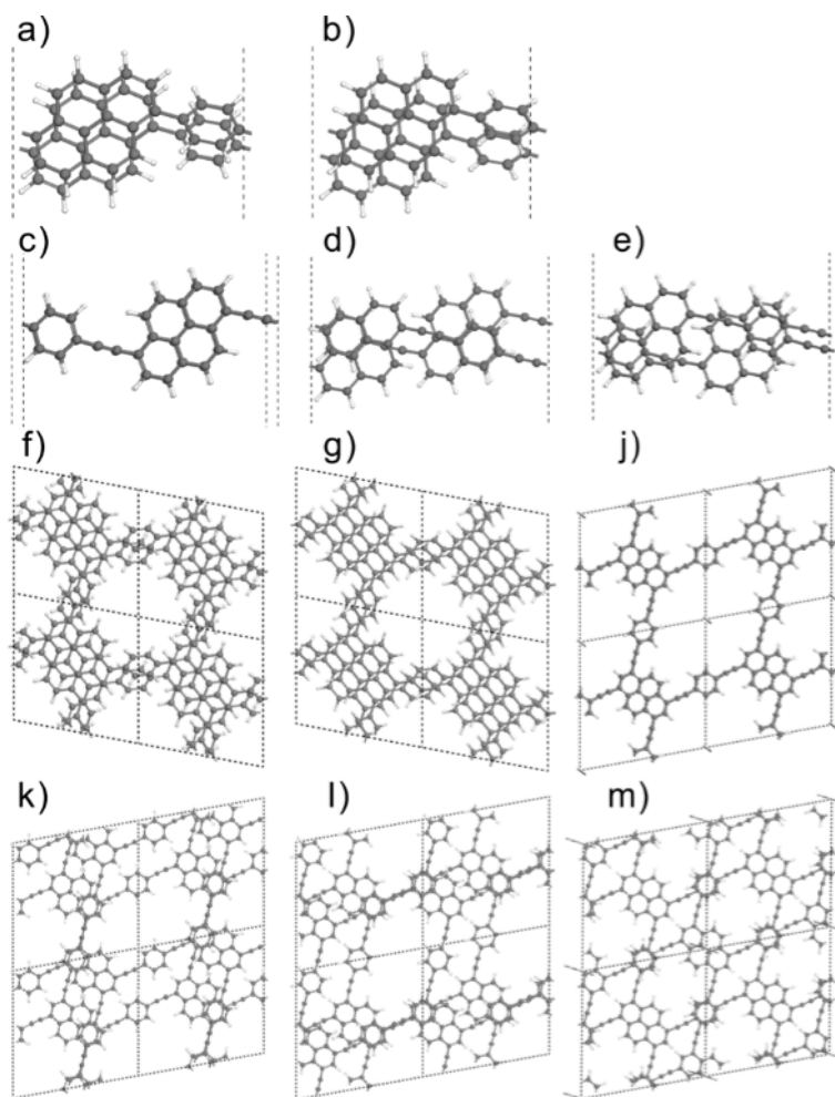
Figure 5.19. Top view of optimized bilayer structures of L-CP-D with (a) AB stacking and (b) AB' stacking, L-CP-A with (c) AA stacking, (d) AB stacking and (e) AB' stacking, N-CP-D with (f) AB stacking and (g) AB' stacking, and N-CP-A with (j) AA stacking, (k) AB stacking and (l) AB' stacking and (m) AC stacking. The dark gray and white balls represent C and H atoms, respectively.
