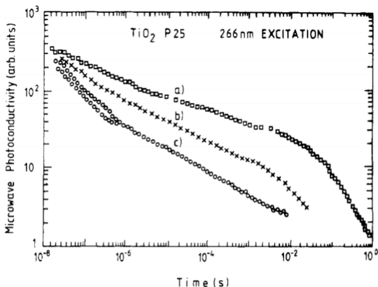
Figure 2.5. Transient photoconductivity of \text{TiO}_2 powder (P25) after laser excitation ( \lambda_{ex} = 266 \text{ nm} ; 0.5\text{--}1 \text{ mJ/cm}^2 ). (a) untreated P25; (b) platinized P25 treated with 2-propanol; (c) platinized P25. [21]
