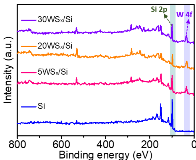
Figure 4.2 The survey spectra of bare Si, 5\text{WS}_x/\text{Si} , 20\text{WS}_x/\text{Si} , and 30\text{WS}_x/\text{Si} .
