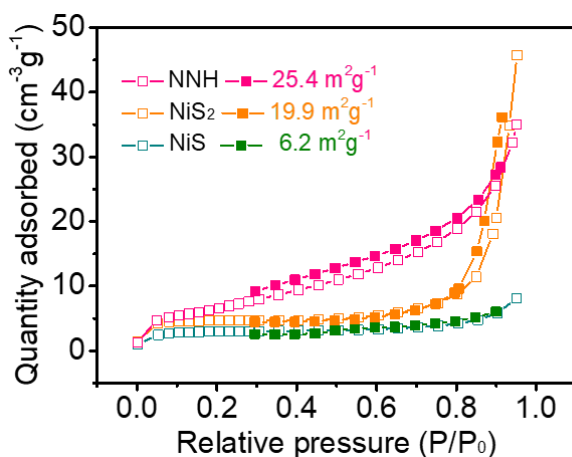
Figure 3.5 \text{N}_2 adsorption and desorption isotherms curves of the NNH, \text{NiS}_2 , and \text{NiS} .
