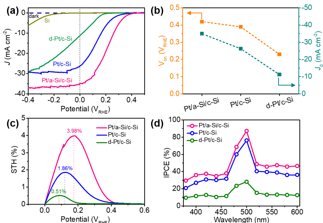
Figure 2.12 (a) LSV curves, (b) comparison of onset potentials ( V_{on} ) and photocurrent densities at 0 V RHE ( J_0 ), (c) half-cell STH efficiency, and (d) IPCE of Pt/a-Si/Si, Pt/c-Si, and d-Pt/c-Si photocathodes.
