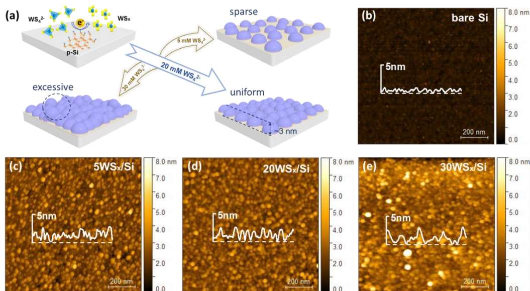
Figure 4.1 (a) Schematic illustration for self-assembled deposition of \text{WS}_x on p-Si. AFM images of (b) bare Si, (c) 5\text{WS}_x/\text{Si} , (d) 20\text{WS}_x/\text{Si} , and (e) 30\text{WS}_x/\text{Si} . The height profiles along the corresponding dashed lines are shown as the inset Figures.
