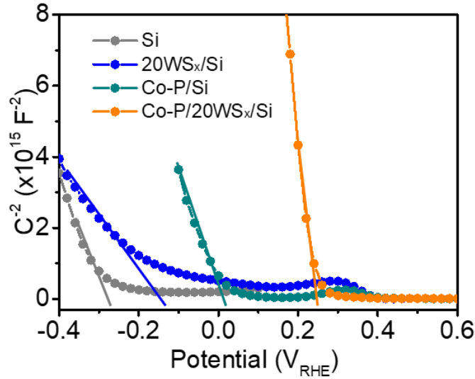
Figure 4.9 Mott-Schottky plots under dark of bare Si, 20WS x /Si, Co-P/Si, and Co-P/20WS x /Si.
