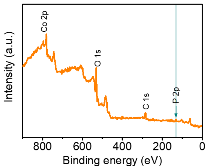
Figure 4.19 XPS survey spectrum of Co-P/20 \text{WS}_x /Si.
