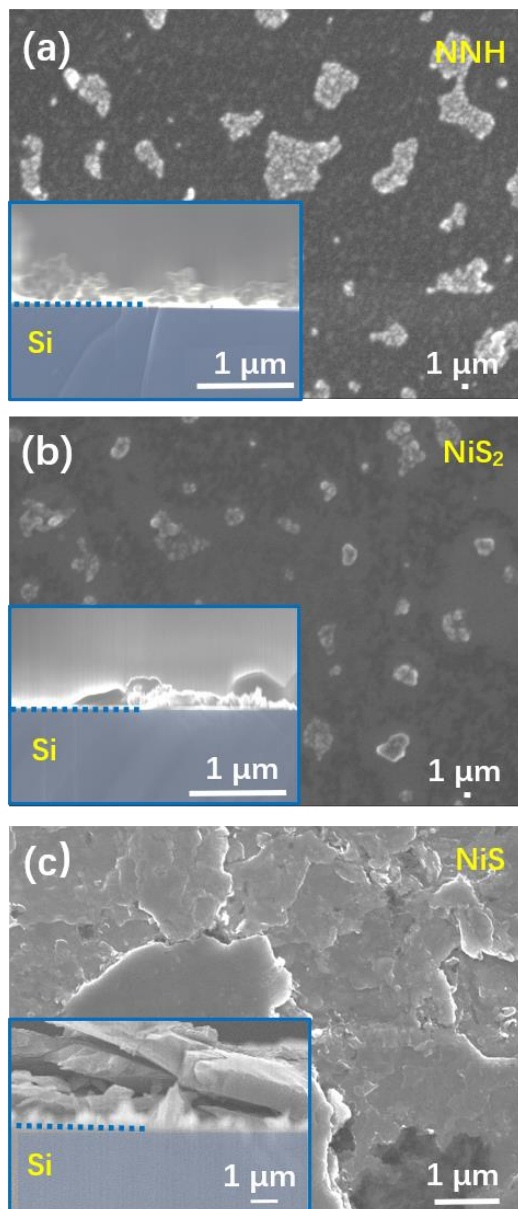
Figure 3.10 SEM images of (a)NNH/Si, (b) \text{NiS}_2/\text{Si} and (c) \text{NiS}/\text{Si} .
