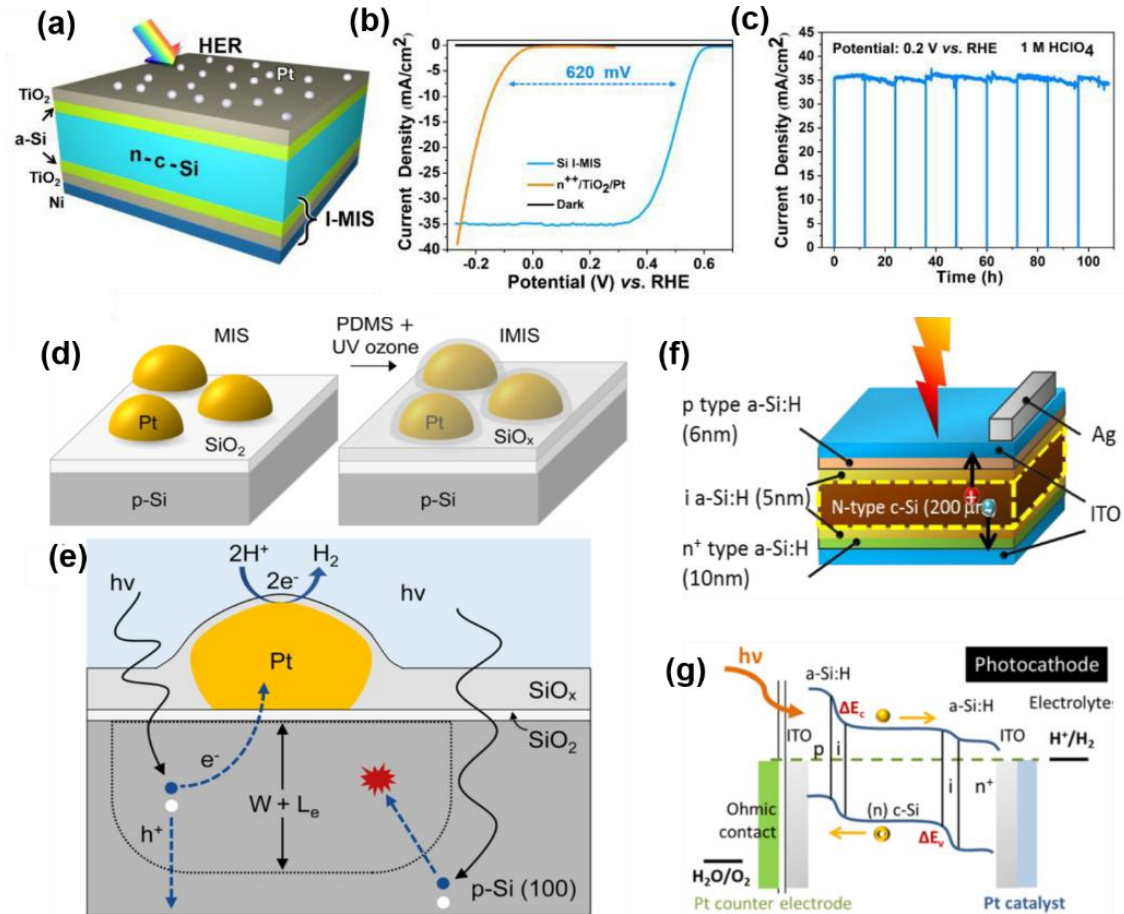
Figure 1.7 (a) Schematic diagram, (b) LSVs, and (c) durability test of the Si I-MIS photocathode. 60 Schematic diagrams of (d) a MIS photocathode and an IMIS photocathode covering a SiO x layer, and (e) the basic operational process occurring in an IMIS photocathode. 61 (f) Configuration and (g) the energy band diagram of the a-Si/c-Si heterojunction photocathode. 17
